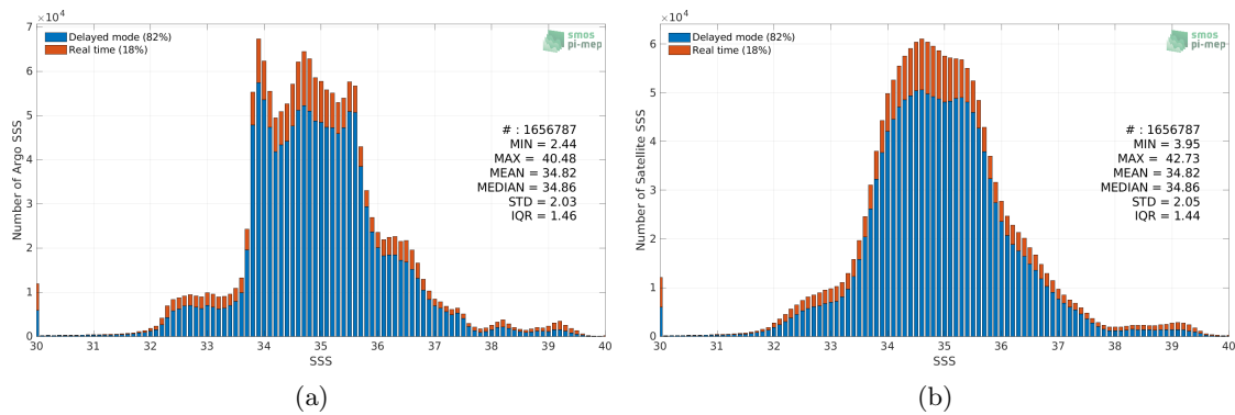
Figure 2: Histograms of SSS from Argo (a) and SMOS SSS L3 v8 - 9 Days (CATDS-CECOS-LOCEAN) (b) considering all match-up pairs per bins of 0.1 over the Global Ocean Pi-MEP region and for the full satellite product period.
