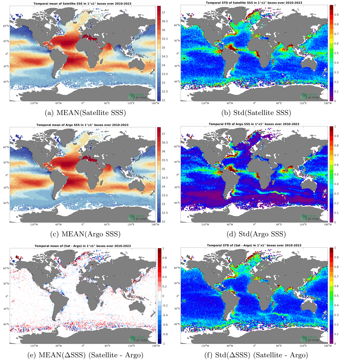
Figure 6: Temporal mean (left) and Std (right) of SSS from SMOS SSS L3 v8 - 9 Days (CATDS-CECOS-LOCEAN) (top), Argo (middle), and of \Delta SSS (Satellite - Argo). Only match-up pairs are used to generate these maps.
