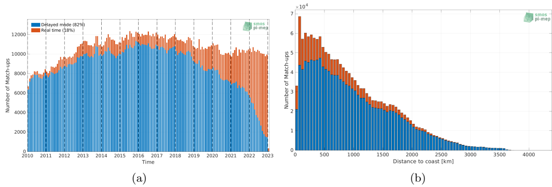
Figure 1: Number of match-ups between Argo and SMOS SSS L3 v8 - 9 Days (CATDS-CECOS-LOCEAN) SSS as a function of time (a) and as function of the distance to coast (b) over the Global Ocean Pi-MEP region and for the full satellite product period.
