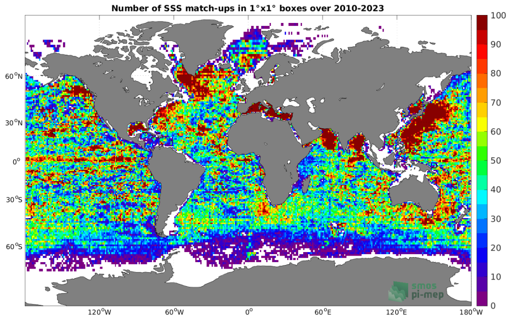
Figure 4: Number of SSS match-ups between Argo SSS and the SMOS SSS L3 v8 - 9 Days (CATDS-CECOS-LOCEAN) SSS product for the Global Ocean Pi-MEP region over 1^\circ \times 1^\circ boxes and for the full satellite product period.
