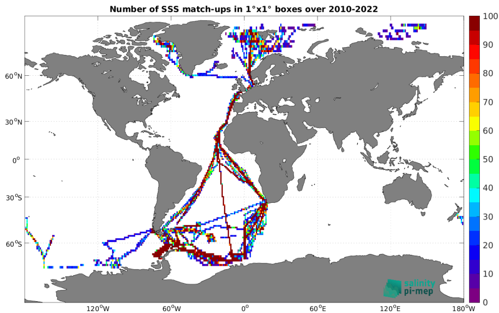
Figure 4: Number of SSS match-ups between TSG (Polarstern) SSS and the SMOS SSS L3 v8 - 18 Days (CATDS-CEC-LOCEAN) SSS product for the Global Ocean Pi-MEP region over 1^\circ \times 1^\circ boxes and for the full satellite product period.
