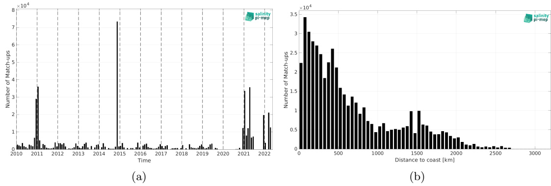
Figure 1: Number of match-ups between TSG (Polarstern) and SMOS SSS L3 v8 - 18 Days (CATDS-CEC-LOCEAN) SSS as a function of time (a) and as function of the distance to coast (b) over the Global Ocean Pi-MEP region and for the full satellite product period.
