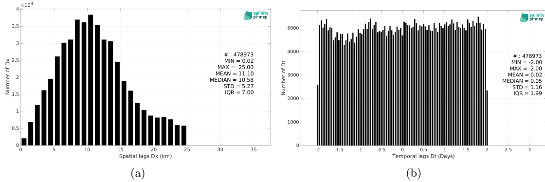
Figure 5: Histograms of the spatial (a) and temporal (b) lags between the location/time of the TSG (Polarstern) measurement and the date of the corresponding SMOS SSS L3 v8 - 18 Days (CATDS-CEC-LOCEAN) SSS pixel.
