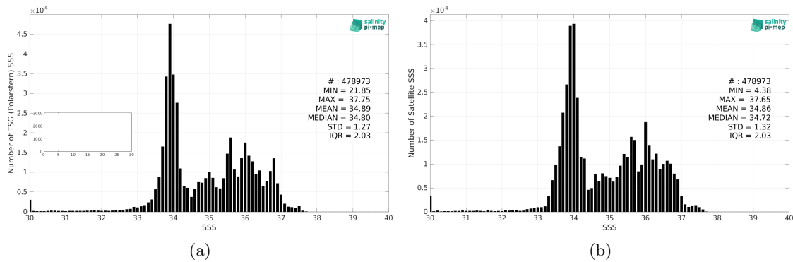
Figure 2: Histograms of SSS from TSG (Polarstern) (a) and SMOS SSS L3 v8 - 18 Days (CATDS-CEC-LOCEAN) (b) considering all match-up pairs per bins of 0.1 over the Global Ocean Pi-MEP region and for the full satellite product period.
