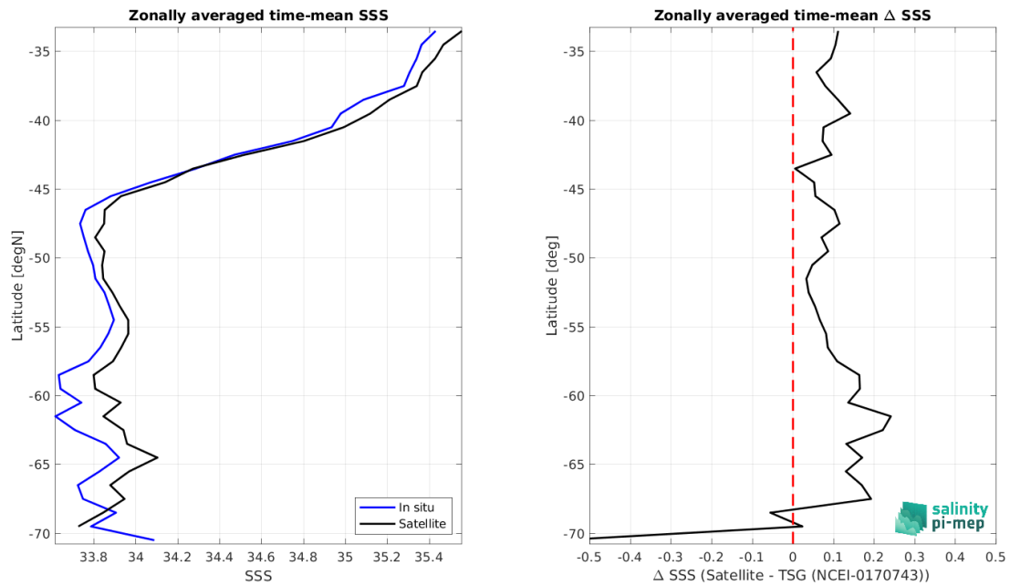
Figure 8: Left panel: Zonal mean SSS from SMOS SSS L3 v8 - 18 Days (CATDS-CEC-LOCEAN) satellite product (black) and from TSG (NCEI-0170743) (blue). Right panel: Zonal mean of \Delta SSS (Satellite - TSG (NCEI-0170743)) for all the collected Pi-MEP match-up pairs estimated over the full satellite product period.
