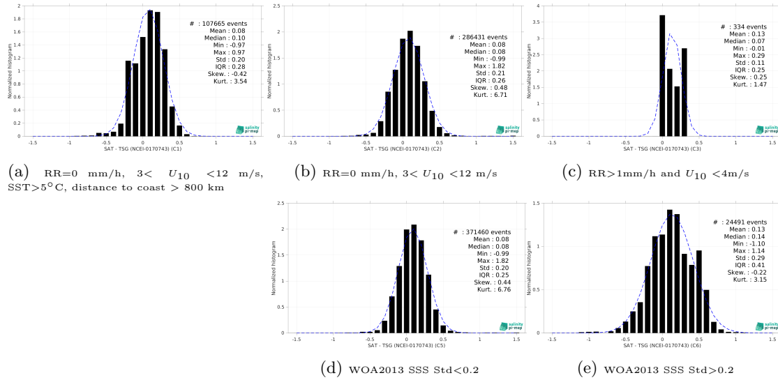
Figure 13: Normalized histogram of \Delta SSS (SMOS SSS L3 v8 - 18 Days (CATDS-CEC-LOCEAN) - TSG (NCEI-0170743)) for 5 different subdatasets corresponding to: RR=0 mm/h, 3 < U_{10} < 12 m/s, SST>5°C, distance to coast > 800 km (a), RR=0 mm/h, 3 < U_{10} < 12 m/s (b), RR>1mm/h and U_{10} < 4 m/s (c), WOA2013 SSS Std<0.2 (d), WOA2013 SSS Std>0.2 (e).
