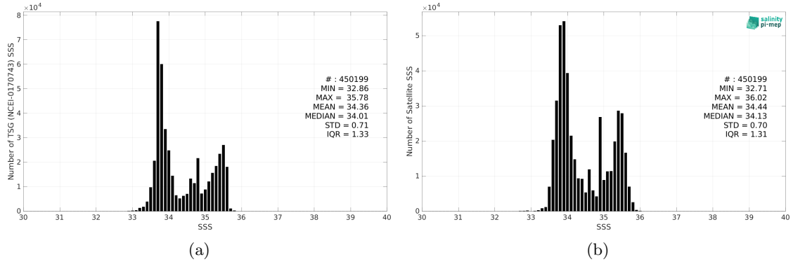
Figure 2: Histograms of SSS from TSG (NCEI-0170743) (a) and SMOS SSS L3 v8 - 18 Days (CATDS-CEC-LOCEAN) (b) considering all match-up pairs per bins of 0.1 over the Global Ocean Pi-MEP region and for the full satellite product period.
