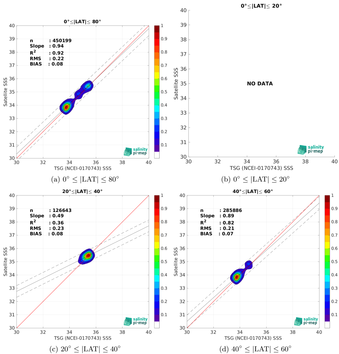
Figure 9: Contour maps of the concentration of SMOS SSS L3 v8 - 18 Days (CATDS-CEC-LOCEAN) SSS (y-axis) versus TSG (NCEI-0170743) SSS (x-axis) at match-up pairs for different latitude bands. For each plot, the red line shows x=y . The black thin and dashed lines indicate a linear fit through the data cloud and the \pm 95\% confidence levels, respectively. The number match-up pairs n , the slope and R^2 coefficient of the linear fit, the root mean square (RMS) and the mean bias between satellite and in situ data are indicated for each latitude band in each plots.
