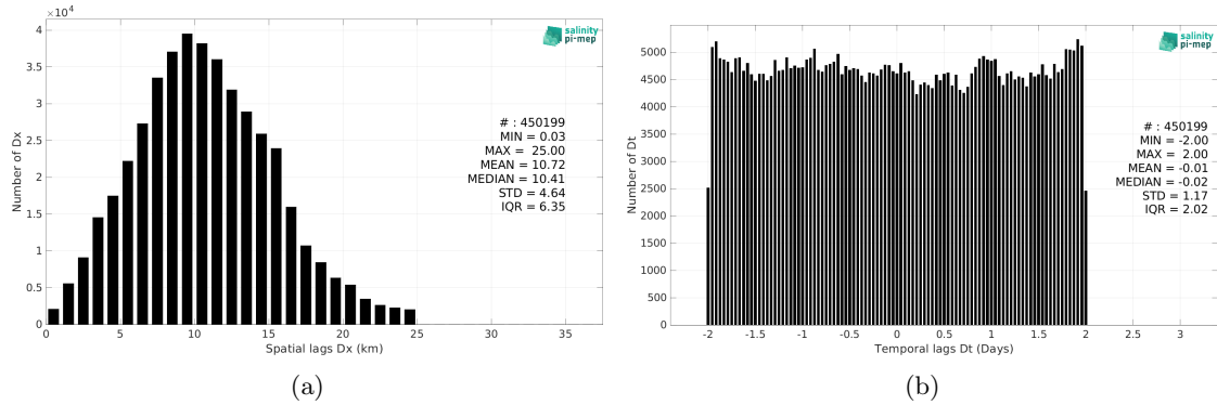
Figure 5: Histograms of the spatial (a) and temporal (b) lags between the location/time of the TSG (NCEI-0170743) measurement and the date of the corresponding SMOS SSS L3 v8 - 18 Days (CATDS-CEC-LOCEAN) SSS pixel.
