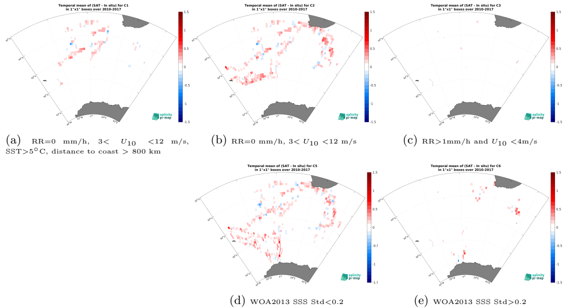
Figure 12: Temporal mean gridded over spatial boxes of size 1^{\circ}\times 1^{\circ} of \Delta\text{SSS} (SMOS SSS L3 v8 - 18 Days (CATDS-CEC-LOCEAN) - TSG (NCEI-0170743)) for 5 different subdatasets corresponding to:RR=0 mm/h, 3 < U_{10} < 12 m/s, SST >5^{\circ}\text{C} , distance to coast > 800 km (a), RR=0 mm/h, 3 < U_{10} < 12 m/s (b), RR >1 mm/h and U_{10} < 4 m/s (c), WOA2013 SSS Std <0.2 (d), WOA2013 SSS Std >0.2 (e).
