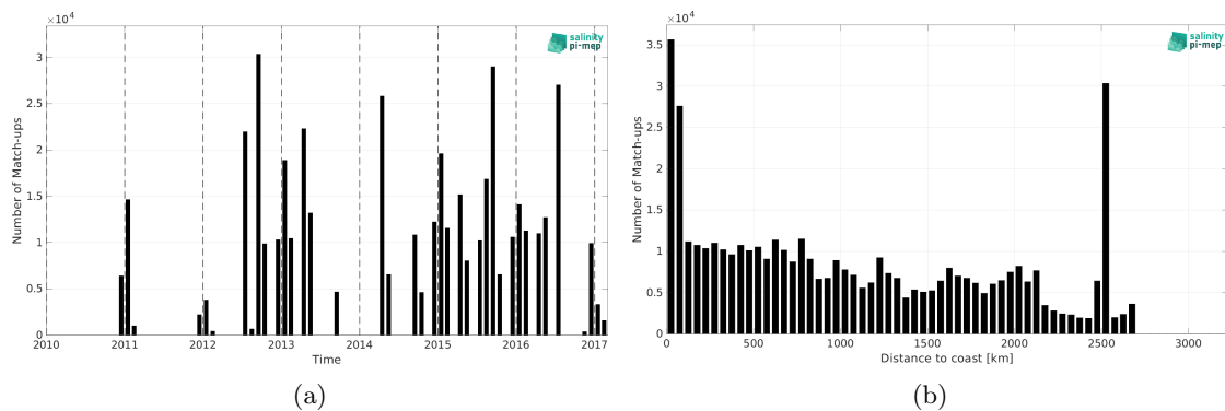
Figure 1: Number of match-ups between TSG (NCEI-0170743) and SMOS SSS L3 v8 - 18 Days (CATDS-CEC-LOCEAN) SSS as a function of time (a) and as function of the distance to coast (b) over the Global Ocean Pi-MEP region and for the full satellite product period.
