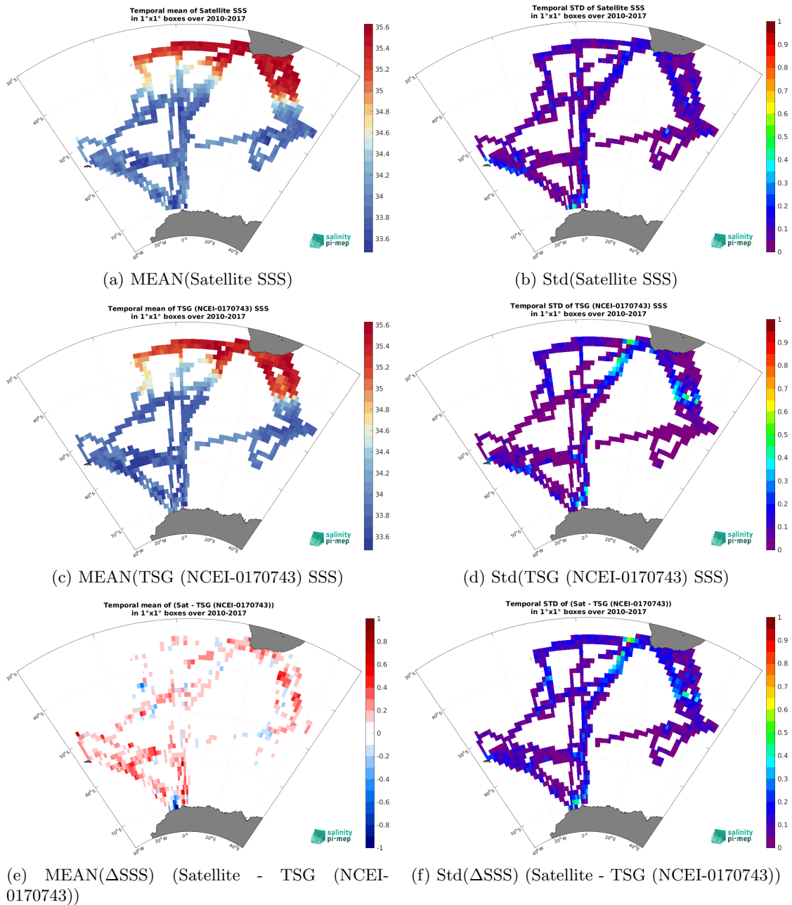
Figure 6: Temporal mean (left) and Std (right) of SSS from SMOS SSS L3 v8 - 18 Days (CATDS-CEC-LOCEAN) (top), TSG (NCEI-0170743) (middle), and of \Delta SSS (Satellite - TSG (NCEI-0170743)). Only match-up pairs are used to generate these maps.
