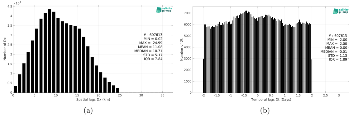
Figure 5: Histograms of the spatial (a) and temporal (b) lags between the location/time of the TSG (LEGOS-Survostral) measurement and the date of the corresponding SMOS SSS L3 v8 - 18 Days (CATDS-CEC-LOCEAN) SSS pixel.
