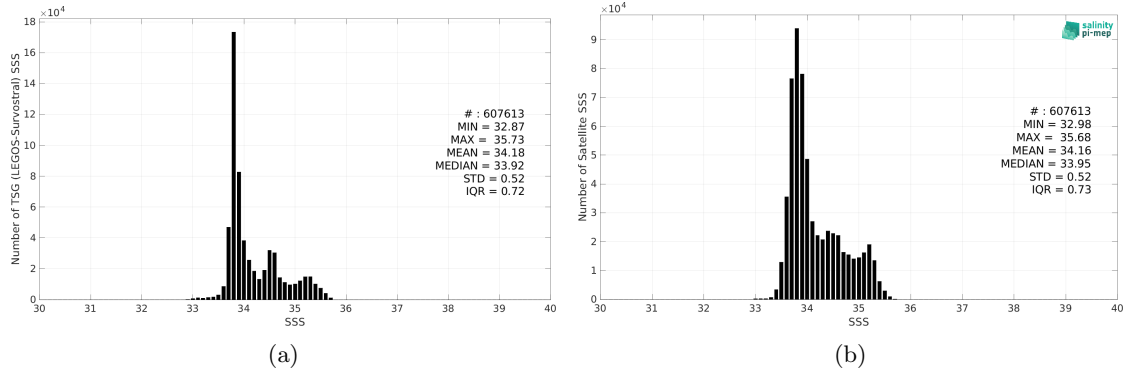
Figure 2: Histograms of SSS from TSG (LEGOS-Survostral) (a) and SMOS SSS L3 v8 - 18 Days (CATDS-CEC-LOCEAN) (b) considering all match-up pairs per bins of 0.1 over the Global Ocean Pi-MEP region and for the full satellite product period.
