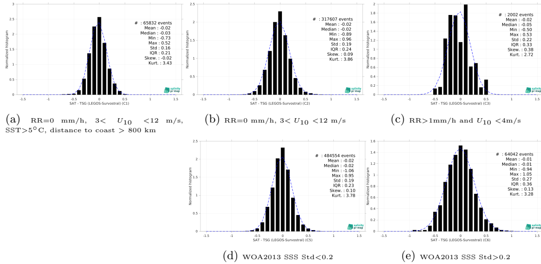
Figure 13: Normalized histogram of \Delta SSS (SMOS SSS L3 v8 - 18 Days (CATDS-CEC-LOCEAN) - TSG (LEGOS-Survostral)) for 5 different subdatasets corresponding to: RR=0 mm/h, 3 < U_{10} < 12 m/s, SST>5°C, distance to coast > 800 km (a), RR=0 mm/h, 3 < U_{10} < 12 m/s (b), RR>1mm/h and U_{10} < 4 m/s (c), WOA2013 SSS Std<0.2 (d), WOA2013 SSS Std>0.2 (e).
