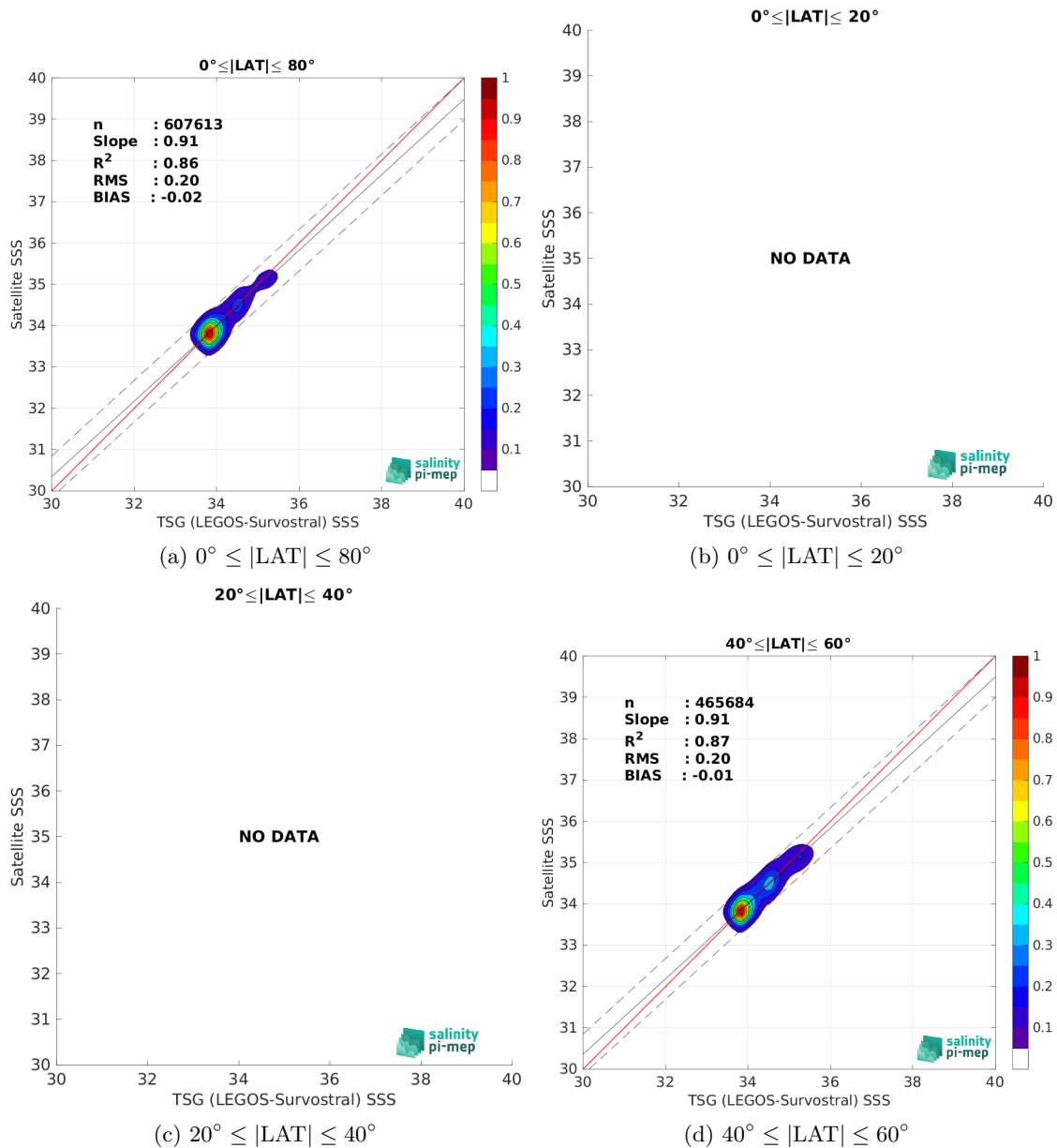
Figure 9: Contour maps of the concentration of SMOS SSS L3 v8 - 18 Days (CATDS-CEC-LOCEAN) SSS (y-axis) versus TSG (LEGOS-Survostral) SSS (x-axis) at match-up pairs for different latitude bands. For each plot, the red line shows x=y . The black thin and dashed lines indicate a linear fit through the data cloud and the \pm 95\% confidence levels, respectively. The number match-up pairs n , the slope and R^2 coefficient of the linear fit, the root mean square (RMS) and the mean bias between satellite and in situ data are indicated for each latitude band in each plots.
