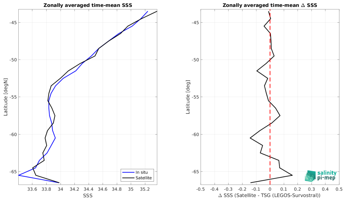
Figure 8: Left panel: Zonal mean SSS from SMOS SSS L3 v8 - 18 Days (CATDS-CEC-LOCEAN) satellite product (black) and from TSG (LEGOS-Survostral) (blue). Right panel: Zonal mean of \Delta SSS (Satellite - TSG (LEGOS-Survostral)) for all the collected Pi-MEP match-up pairs estimated over the full satellite product period.
