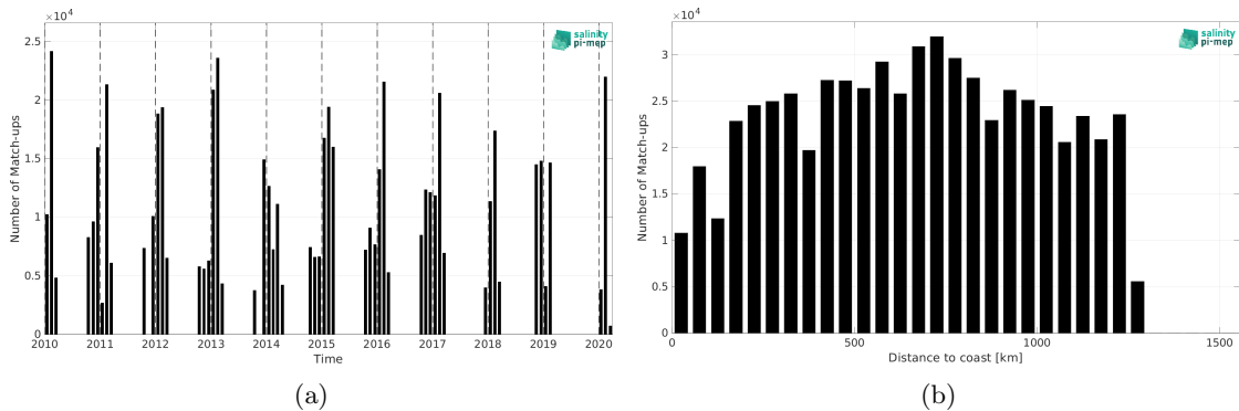
Figure 1: Number of match-ups between TSG (LEGOS-Survostral) and SMOS SSS L3 v8 - 18 Days (CATDS-CEC-LOCEAN) SSS as a function of time (a) and as function of the distance to coast (b) over the Global Ocean Pi-MEP region and for the full satellite product period.
