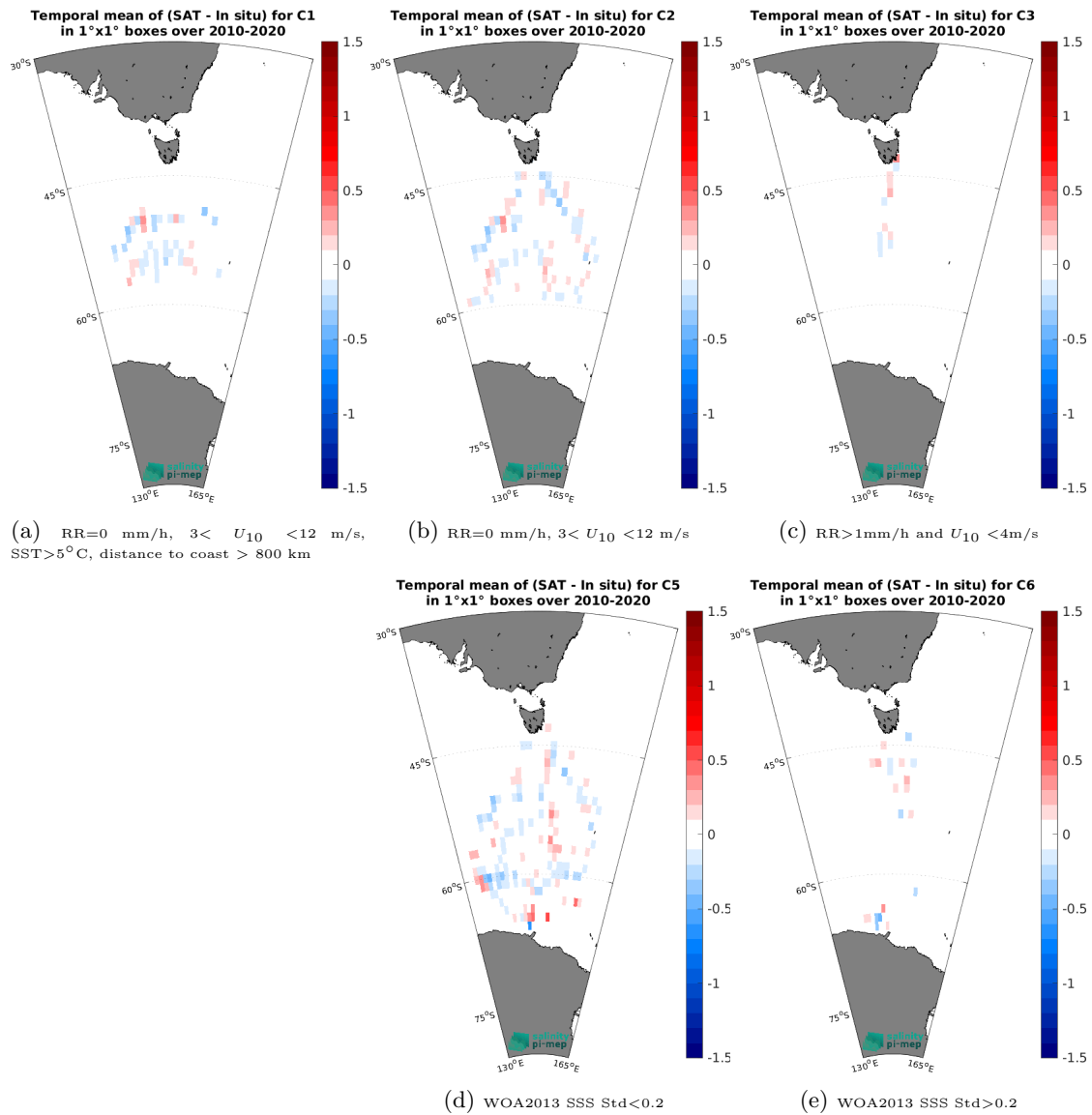
Figure 12: Temporal mean gridded over spatial boxes of size 1^\circ \times 1^\circ of \Delta\text{SSS} (SMOS SSS L3 v8 - 18 Days (CATDS-CEC-LOCEAN) - TSG (LEGOS-Survostral)) for 5 different subdatasets corresponding to: RR=0 mm/h, 3 < U_{10} < 12 m/s, SST > 5^\circ\text{C} , distance to coast > 800 km (a), RR=0 mm/h, 3 < U_{10} < 12 m/s (b), RR > 1 mm/h and U_{10} < 4 m/s (c), WOA2013 SSS Std < 0.2 (d), WOA2013 SSS Std > 0.2 (e).
