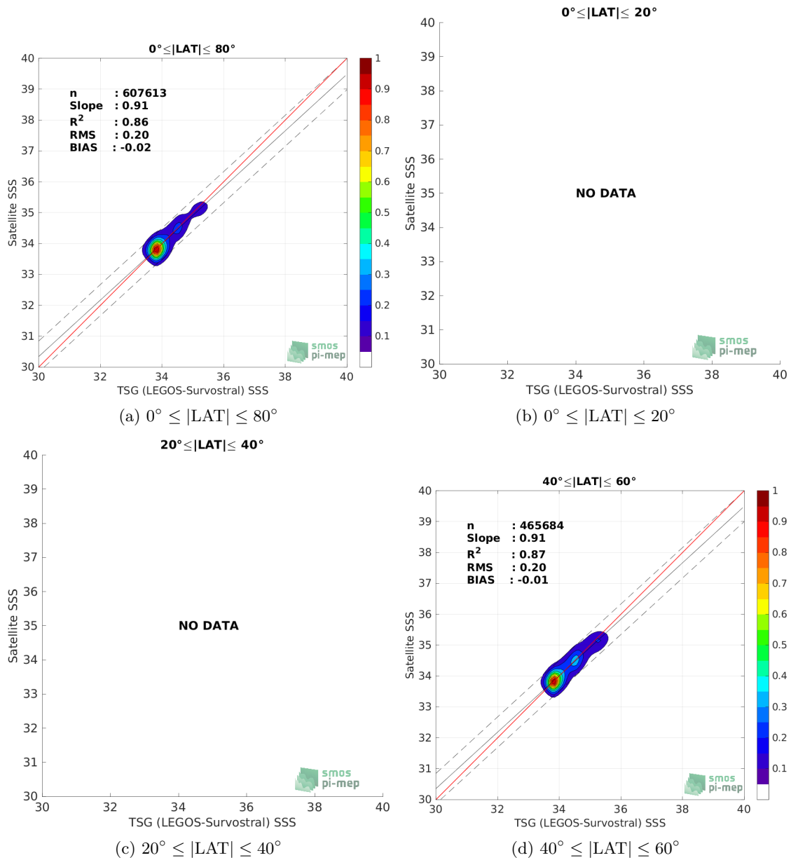
Figure 9: Contour maps of the concentration of SMOS SSS L3 v8 - 18 Days (CATDS-CECOS-LOCEAN) SSS (y-axis) versus TSG (LEGOS-Survostral) SSS (x-axis) at match-up pairs for different latitude bands. For each plot, the red line shows x=y . The black thin and dashed lines indicate a linear fit through the data cloud and the \pm 95\% confidence levels, respectively. The number match-up pairs n , the slope and R^2 coefficient of the linear fit, the root mean square (RMS) and the mean bias between satellite and in situ data are indicated for each latitude band in each plots.
