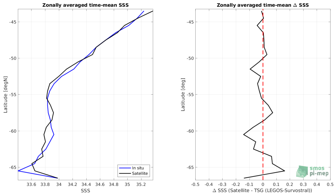
Figure 8: Left panel: Zonal mean SSS from SMOS SSS L3 v8 - 18 Days (CATDS-CECOS-LOCEAN) satellite product (black) and from TSG (LEGOS-Survostral) (blue). Right panel: Zonal mean of \Delta SSS (Satellite - TSG (LEGOS-Survostral)) for all the collected Pi-MEP match-up pairs estimated over the full satellite product period.
