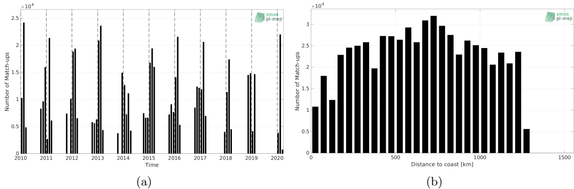
Figure 1: Number of match-ups between TSG (LEGOS-Survostral) and SMOS SSS L3 v8 - 18 Days (CATDS-CECOS-LOCEAN) SSS as a function of time (a) and as function of the distance to coast (b) over the Global Ocean Pi-MEP region and for the full satellite product period.
