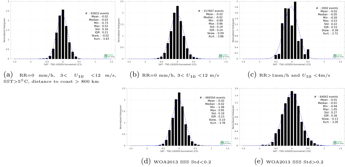
Figure 13: Normalized histogram of \Delta SSS (SMOS SSS L3 v8 - 18 Days (CATDS-CECOS-LOCEAN) - TSG (LEGOS-Survostral)) for 5 different subdatasets corresponding to: RR=0 mm/h, 3 < U_{10} < 12 m/s, SST>5°C, distance to coast > 800 km (a), RR=0 mm/h, 3 < U_{10} < 12 m/s (b), RR>1mm/h and U_{10} < 4 m/s (c), WOA2013 SSS Std<0.2 (d), WOA2013 SSS Std>0.2 (e).
