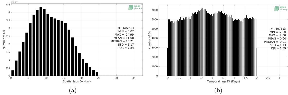
Figure 5: Histograms of the spatial (a) and temporal (b) lags between the location/time of the TSG (LEGOS-Survostral) measurement and the date of the corresponding SMOS SSS L3 v8 - 18 Days (CATDS-CECOS-LOCEAN) SSS pixel.
