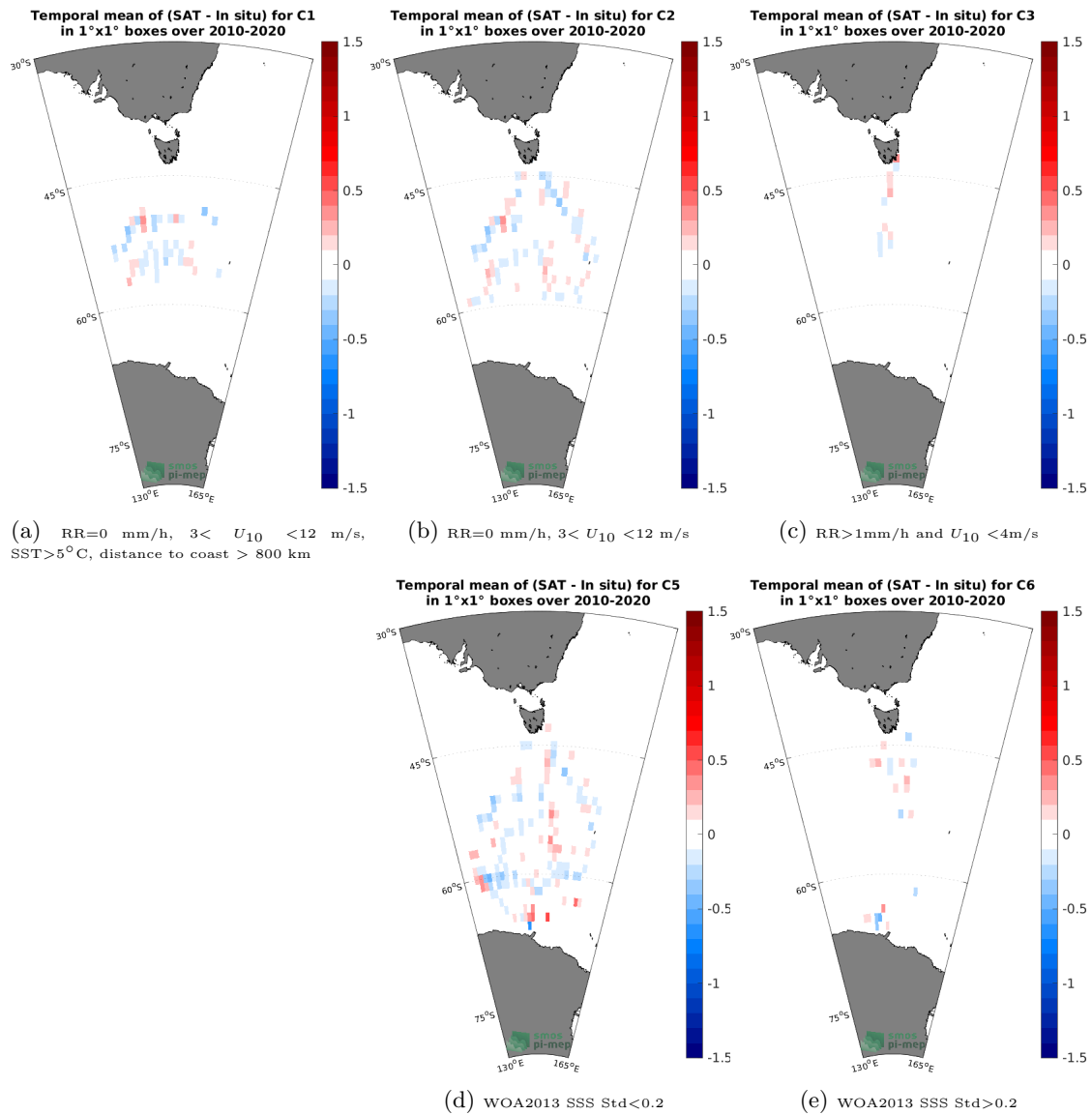
Figure 12: Temporal mean gridded over spatial boxes of size 1^\circ \times 1^\circ of \Delta SSS (SMOS SSS L3 v8 - 18 Days (CATDS-CECOS-LOCEAN) - TSG (LEGOS-Survostral)) for 5 different subdatasets corresponding to:RR=0 mm/h, 3 < U_{10} < 12 m/s, SST>5°C, distance to coast > 800 km (a), RR=0 mm/h, 3 < U_{10} < 12 m/s (b), RR>1mm/h and U_{10} < 4 m/s (c), WOA2013 SSS Std<0.2 (d), WOA2013 SSS Std>0.2 (e).
