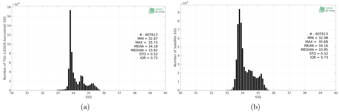
Figure 2: Histograms of SSS from TSG (LEGOS-Survostral) (a) and SMOS SSS L3 v8 - 18 Days (CATDS-CECOS-LOCEAN) (b) considering all match-up pairs per bins of 0.1 over the Global Ocean Pi-MEP region and for the full satellite product period.
