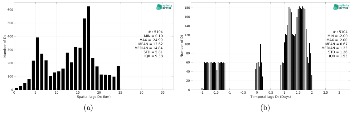
Figure 5: Histograms of the spatial (a) and temporal (b) lags between the location/time of the TSG (LEGOS-Surv-Adel) measurement and the date of the corresponding SMOS SSS L3 v8 - 18 Days (CATDS-CEC-LOCEAN) SSS pixel.
