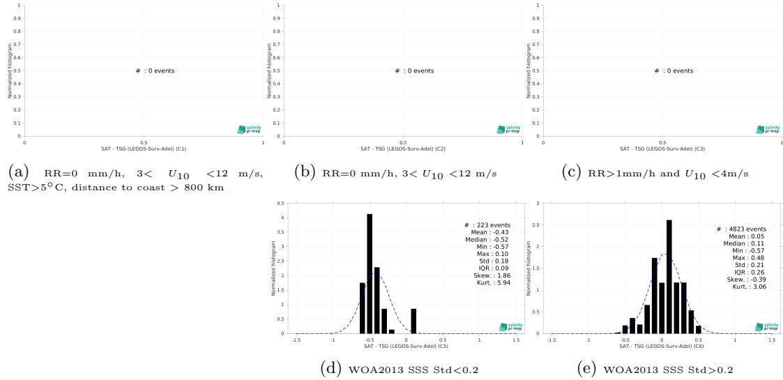
Figure 13: Normalized histogram of \Delta SSS (SMOS SSS L3 v8 - 18 Days (CATDS-CEC-LOCEAN) - TSG (LEGOS-Surv-Adel)) for 5 different subdatasets corresponding to: RR=0 mm/h, 3 < U_{10} < 12 m/s, SST > 5°C, distance to coast > 800 km (a), RR=0 mm/h, 3 < U_{10} < 12 m/s (b), RR > 1mm/h and U_{10} < 4 m/s (c), WOA2013 SSS Std < 0.2 (d), WOA2013 SSS Std > 0.2 (e).
