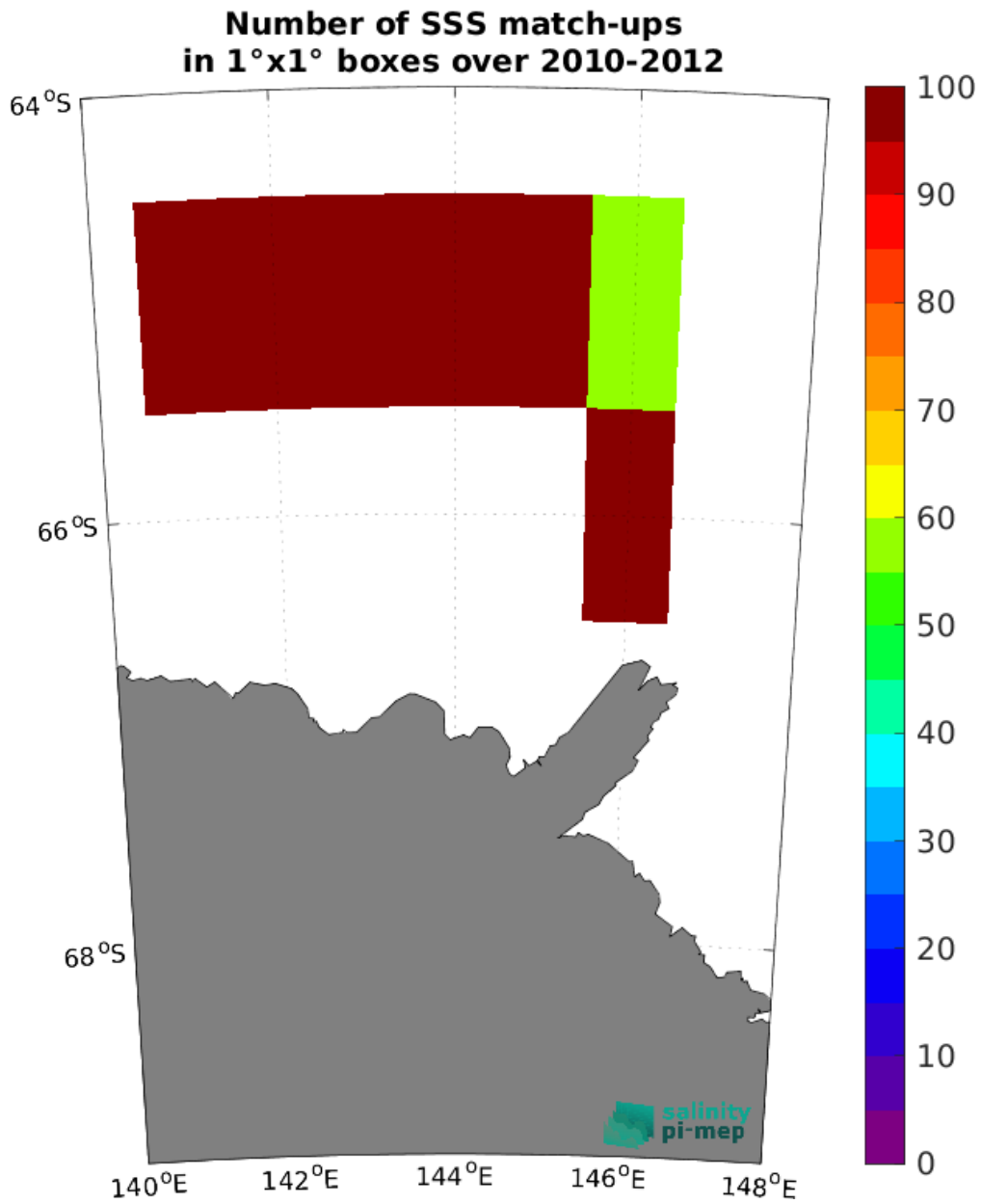
Figure 4: Number of SSS match-ups between TSG (LEGOS-Surv-Adel) SSS and the SMOS SSS L3 v8 - 18 Days (CATDS-CEC-LOCEAN) SSS product for the Global Ocean Pi-MEP region over 1^\circ \times 1^\circ boxes and for the full satellite product period.
