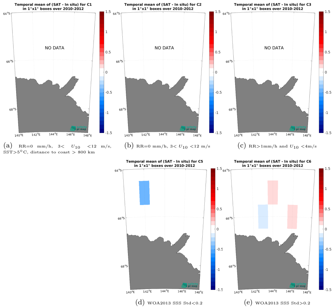
Figure 12: Temporal mean gridded over spatial boxes of size 1^\circ \times 1^\circ of \Delta SSS (SMOS SSS L3 v8 - 18 Days (CATDS-CEC-LOCEAN) - TSG (LEGOS-Surv-Adel)) for 5 different subdatasets corresponding to: RR=0 mm/h, 3 < U_{10} < 12 m/s, SST > 5^\circ\text{C} , distance to coast > 800 km (a), RR=0 mm/h, 3 < U_{10} < 12 m/s (b), RR > 1 mm/h and U_{10} < 4 m/s (c), WOA2013 SSS Std < 0.2 (d), WOA2013 SSS Std > 0.2 (e).
