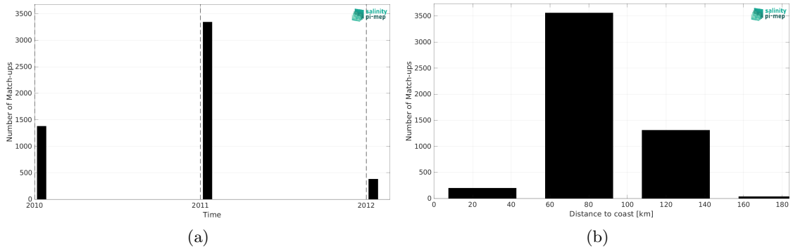
Figure 1: Number of match-ups between TSG (LEGOS-Surv-Adel) and SMOS SSS L3 v8 - 18 Days (CATDS-CEC-LOCEAN) SSS as a function of time (a) and as function of the distance to coast (b) over the Global Ocean Pi-MEP region and for the full satellite product period.
