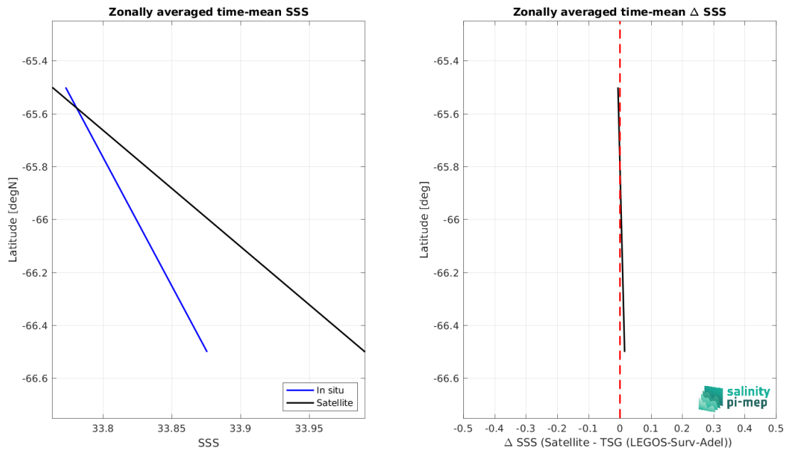
Figure 8: Left panel: Zonal mean SSS from SMOS SSS L3 v8 - 18 Days (CATDS-CEC-LOCEAN) satellite product (black) and from TSG (LEGOS-Surv-Adel) (blue). Right panel: Zonal mean of \Delta SSS (Satellite - TSG (LEGOS-Surv-Adel)) for all the collected Pi-MEP match-up pairs estimated over the full satellite product period.
