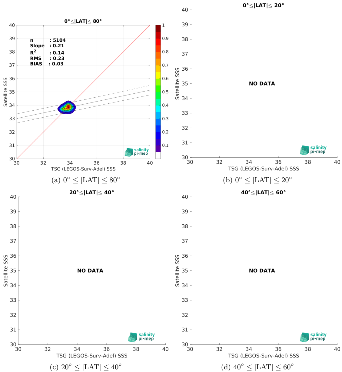
Figure 9: Contour maps of the concentration of SMOS SSS L3 v8 - 18 Days (CATDS-CEC-LOCEAN) SSS (y-axis) versus TSG (LEGOS-Surv-Adel) SSS (x-axis) at match-up pairs for different latitude bands. For each plot, the red line shows x=y . The black thin and dashed lines indicate a linear fit through the data cloud and the \pm 95\% confidence levels, respectively. The number match-up pairs n , the slope and R^2 coefficient of the linear fit, the root mean square (RMS) and the mean bias between satellite and in situ data are indicated for each latitude band in each plots.
