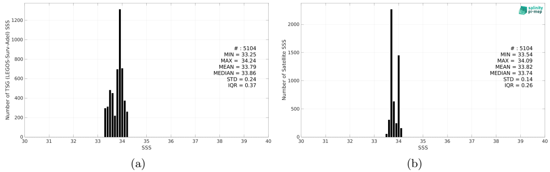
Figure 2: Histograms of SSS from TSG (LEGOS-Surv-Adel) (a) and SMOS SSS L3 v8 - 18 Days (CATDS-CEC-LOCEAN) (b) considering all match-up pairs per bins of 0.1 over the Global Ocean Pi-MEP region and for the full satellite product period.
