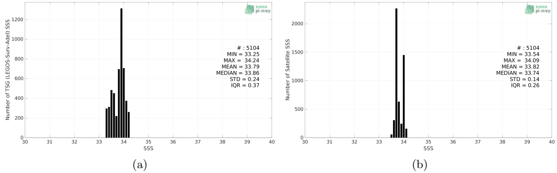
Figure 2: Histograms of SSS from TSG (LEGOS-Surv-Adel) (a) and SMOS SSS L3 v8 - 18 Days (CATDS-CECOS-LOCEAN) (b) considering all match-up pairs per bins of 0.1 over the Global Ocean Pi-MEP region and for the full satellite product period.
