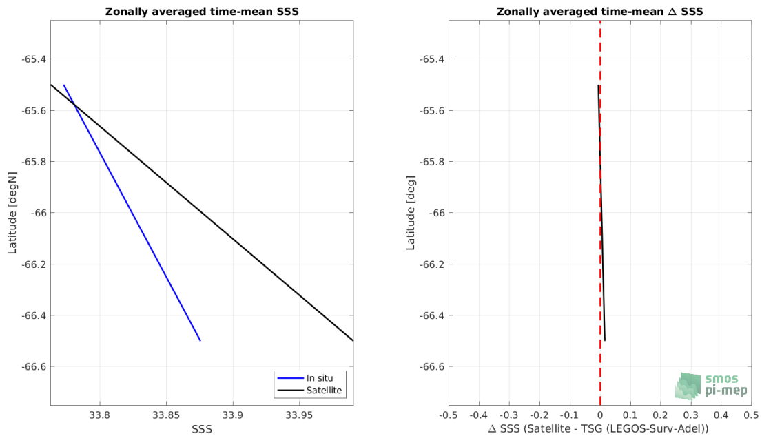
Figure 8: Left panel: Zonal mean SSS from SMOS SSS L3 v8 - 18 Days (CATDS-CECOS-LOCEAN) satellite product (black) and from TSG (LEGOS-Surv-Adel) (blue). Right panel: Zonal mean of \Delta SSS (Satellite - TSG (LEGOS-Surv-Adel)) for all the collected Pi-MEP match-up pairs estimated over the full satellite product period.
