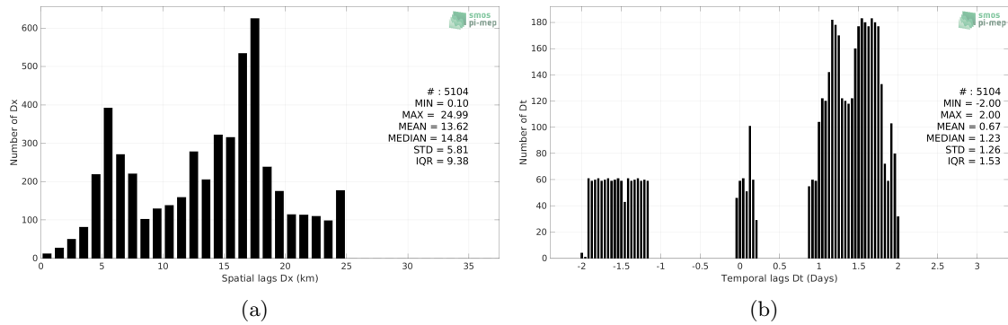
Figure 5: Histograms of the spatial (a) and temporal (b) lags between the location/time of the TSG (LEGOS-Surv-Adel) measurement and the date of the corresponding SMOS SSS L3 v8 - 18 Days (CATDS-CECOS-LOCEAN) SSS pixel.
