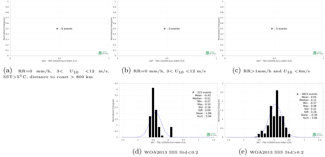
Figure 13: Normalized histogram of \Delta SSS (SMOS SSS L3 v8 - 18 Days (CATDS-CECOS-LOCEAN) - TSG (LEGOS-Surv-Adel)) for 5 different subdatasets corresponding to: RR=0 mm/h, 3 < U_{10} < 12 m/s, SST > 5°C, distance to coast > 800 km (a), RR=0 mm/h, 3 < U_{10} < 12 m/s (b), RR > 1mm/h and U_{10} < 4 m/s (c), WOA2013 SSS Std < 0.2 (d), WOA2013 SSS Std > 0.2 (e).
