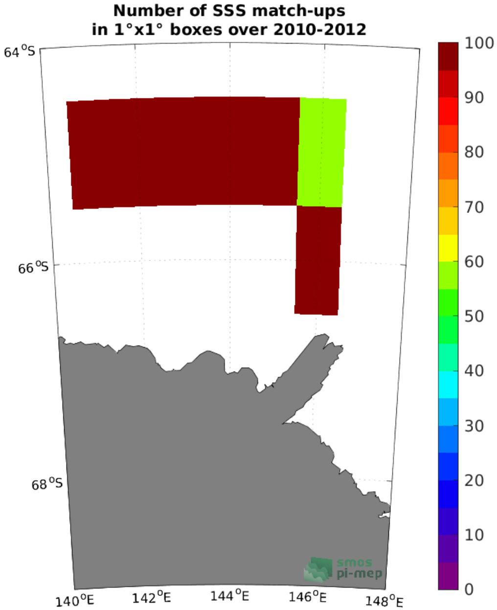
Figure 4: Number of SSS match-ups between TSG (LEGOS-Surv-Adel) SSS and the SMOS SSS L3 v8 - 18 Days (CATDS-CECOS-LOCEAN) SSS product for the Global Ocean Pi-MEP region over 1°x1° boxes and for the full satellite product period.
