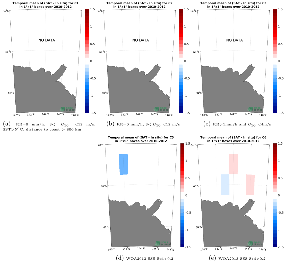
Figure 12: Temporal mean gridded over spatial boxes of size 1^\circ \times 1^\circ of \Delta SSS (SMOS SSS L3 v8 - 18 Days (CATDS-CECOS-LOCEAN) - TSG (LEGOS-Surv-Adel)) for 5 different subdatasets corresponding to:RR=0 mm/h, 3 < U_{10} < 12 m/s, SST>5°C, distance to coast > 800 km (a), RR=0 mm/h, 3 < U_{10} < 12 m/s (b), RR>1mm/h and U_{10} < 4 m/s (c), WOA2013 SSS Std<0.2 (d), WOA2013 SSS Std>0.2 (e).
