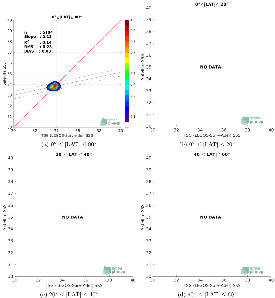
Figure 9: Contour maps of the concentration of SMOS SSS L3 v8 - 18 Days (CATDS-CECOS-LOCEAN) SSS (y-axis) versus TSG (LEGOS-Surv-Adel) SSS (x-axis) at match-up pairs for different latitude bands. For each plot, the red line shows x=y . The black thin and dashed lines indicate a linear fit through the data cloud and the \pm 95\% confidence levels, respectively. The number match-up pairs n , the slope and R^2 coefficient of the linear fit, the root mean square (RMS) and the mean bias between satellite and in situ data are indicated for each latitude band in each plots.
