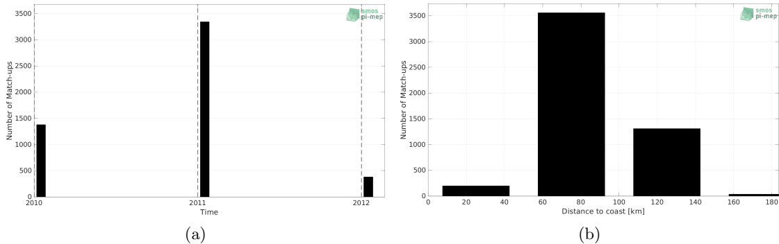
Figure 1: Number of match-ups between TSG (LEGOS-Surv-Adel) and SMOS SSS L3 v8 - 18 Days (CATDS-CECOS-LOCEAN) SSS as a function of time (a) and as function of the distance to coast (b) over the Global Ocean Pi-MEP region and for the full satellite product period.
