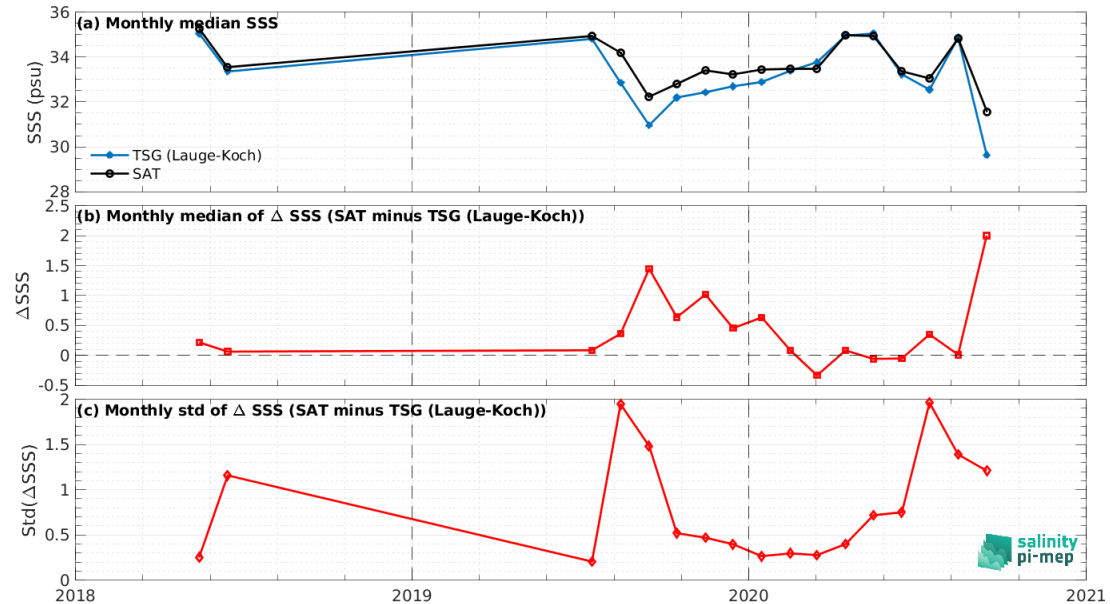
Figure 7: Time series of the monthly median SSS (top), median of \Delta SSS (Satellite - TSG (Lauge-Koch)) and Std of \Delta SSS (Satellite - TSG (Lauge-Koch)) over the Global Ocean Pi-MEP region considering all match-ups collected by the Pi-MEP.
