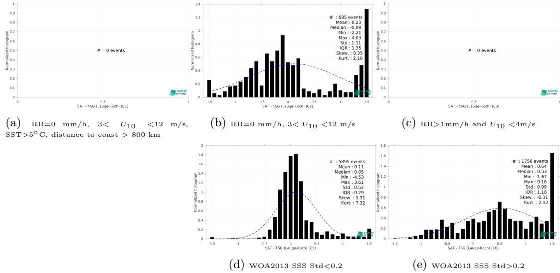
Figure 13: Normalized histogram of \Delta SSS (SMOS SSS L3 v8 - 18 Days (CATDS-CEC-LOCEAN) - TSG (Lauge-Koch)) for 5 different subdatasets corresponding to: RR=0 mm/h, 3 < U_{10} < 12 m/s, SST > 5°C, distance to coast > 800 km (a), RR=0 mm/h, 3 < U_{10} < 12 m/s (b), RR > 1mm/h and U_{10} < 4 m/s (c), WOA2013 SSS Std < 0.2 (d), WOA2013 SSS Std > 0.2 (e).
