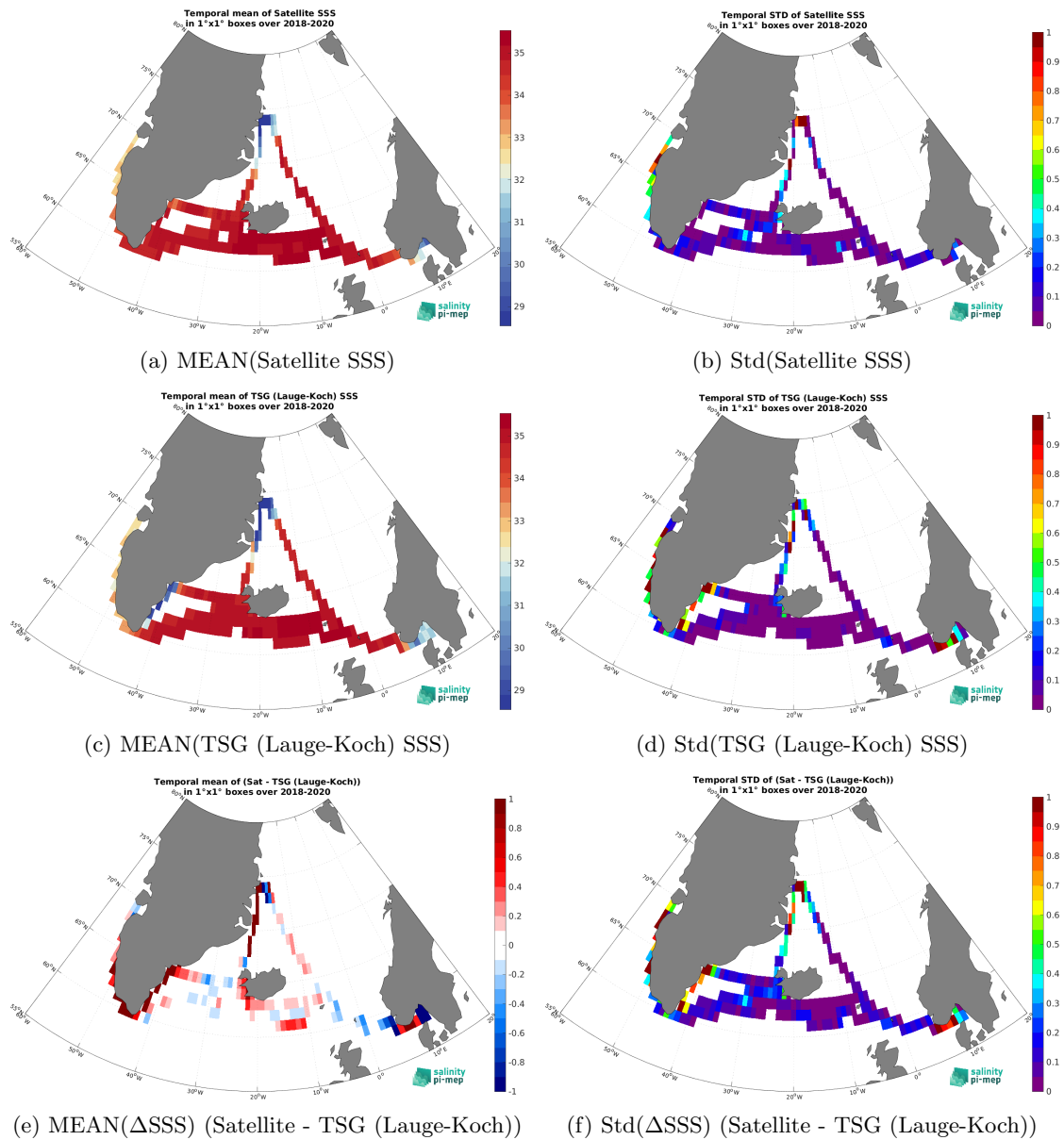
Figure 6: Temporal mean (left) and Std (right) of SSS from SMOS SSS L3 v8 - 18 Days (CATDS-CEC-LOCEAN) (top), TSG (Lauge-Koch) (middle), and of \Delta SSS (Satellite - TSG (Lauge-Koch)). Only match-up pairs are used to generate these maps.
