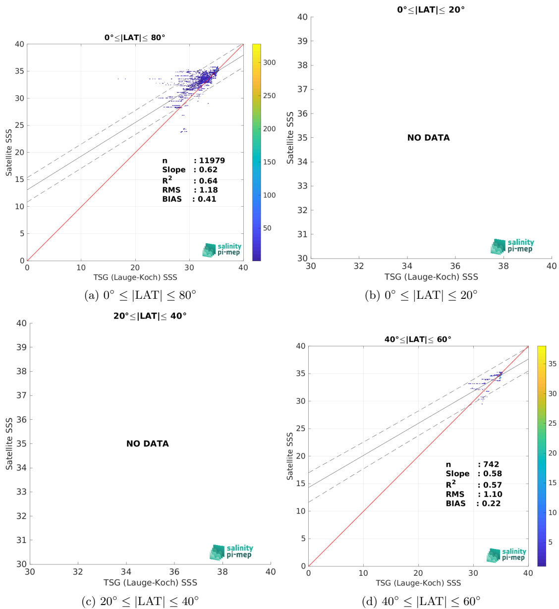
Figure 9: Contour maps of the concentration of SMOS SSS L3 v8 - 18 Days (CATDS-CEC-LOCEAN) SSS (y-axis) versus TSG (Lauge-Koch) SSS (x-axis) at match-up pairs for different latitude bands. For each plot, the red line shows x=y . The black thin and dashed lines indicate a linear fit through the data cloud and the \pm 95\% confidence levels, respectively. The number match-up pairs n , the slope and R^2 coefficient of the linear fit, the root mean square (RMS) and the mean bias between satellite and in situ data are indicated for each latitude band in each plots.
