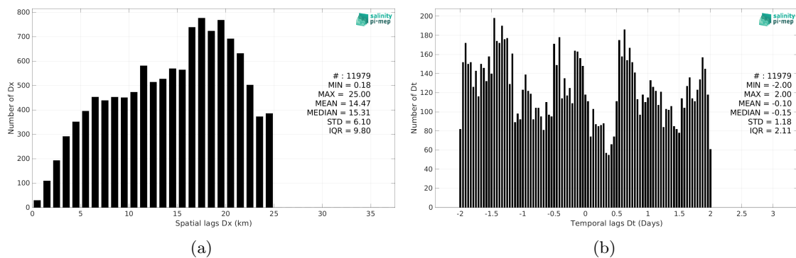
Figure 5: Histograms of the spatial (a) and temporal (b) lags between the location/time of the TSG (Lauge-Koch) measurement and the date of the corresponding SMOS SSS L3 v8 - 18 Days (CATDS-CEC-LOCEAN) SSS pixel.
