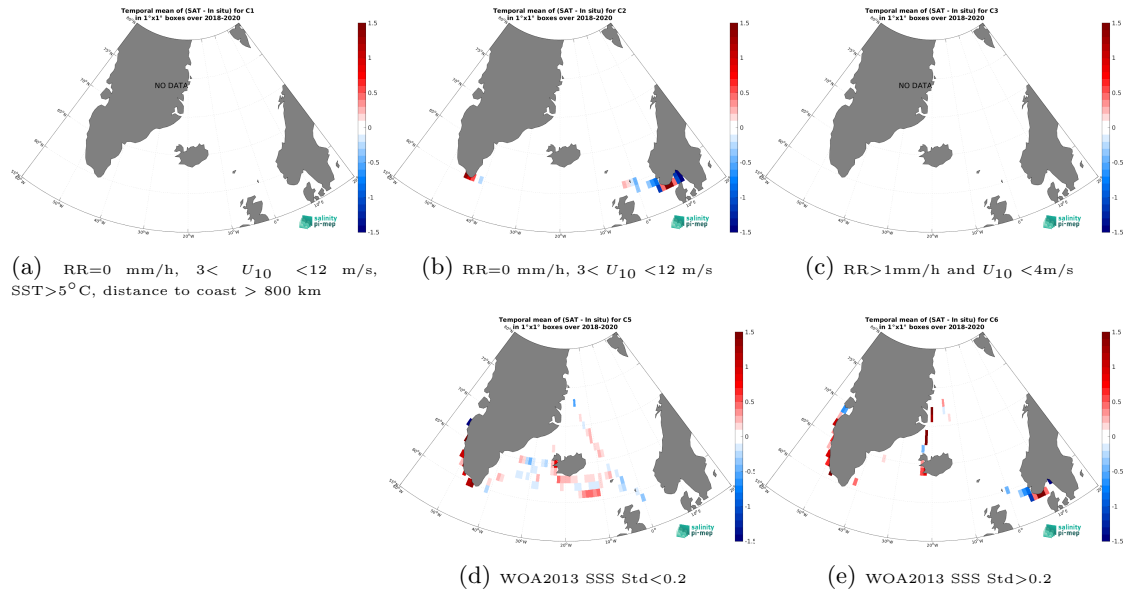
Figure 12: Temporal mean gridded over spatial boxes of size 1^{\circ}\times 1^{\circ} of \Delta\text{SSS} (SMOS SSS L3 v8 - 18 Days (CATDS-CEC-LOCEAN) - TSG (Lauge-Koch)) for 5 different subdatasets corresponding to: RR=0 mm/h, 3 < U_{10} < 12 m/s, SST > 5^{\circ}\text{C} , distance to coast > 800 km (a), RR=0 mm/h, 3 < U_{10} < 12 m/s (b), RR > 1 mm/h and U_{10} < 4 m/s (c), WOA2013 SSS Std < 0.2 (d), WOA2013 SSS Std > 0.2 (e).
