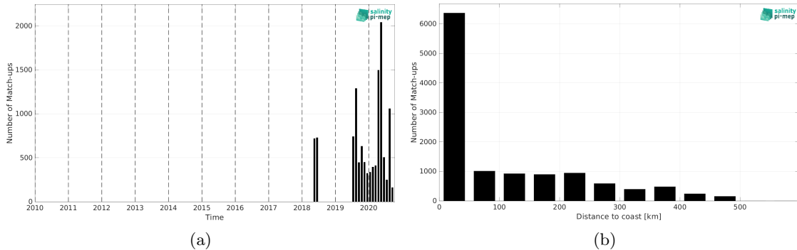
Figure 1: Number of match-ups between TSG (Lauge-Koch) and SMOS SSS L3 v8 - 18 Days (CATDS-CEC-LOCEAN) SSS as a function of time (a) and as function of the distance to coast (b) over the Global Ocean Pi-MEP region and for the full satellite product period.
