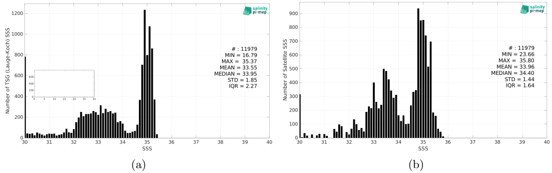
Figure 2: Histograms of SSS from TSG (Lauge-Koch) (a) and SMOS SSS L3 v8 - 18 Days (CATDS-CEC-LOCEAN) (b) considering all match-up pairs per bins of 0.1 over the Global Ocean Pi-MEP region and for the full satellite product period.
