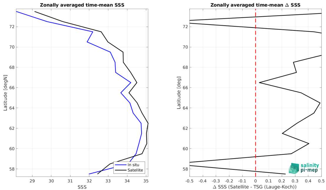
Figure 8: Left panel: Zonal mean SSS from SMOS SSS L3 v8 - 18 Days (CATDS-CEC-LOCEAN) satellite product (black) and from TSG (Lauge-Koch) (blue). Right panel: Zonal mean of \Delta SSS (Satellite - TSG (Lauge-Koch)) for all the collected Pi-MEP match-up pairs estimated over the full satellite product period.
