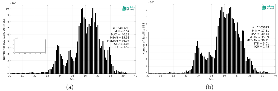
Figure 2: Histograms of SSS from TSG (CSIC-UTM) (a) and SMOS SSS L3 v8 - 18 Days (CATDS-CEC-LOCEAN) (b) considering all match-up pairs per bins of 0.1 over the Global Ocean Pi-MEP region and for the full satellite product period.
