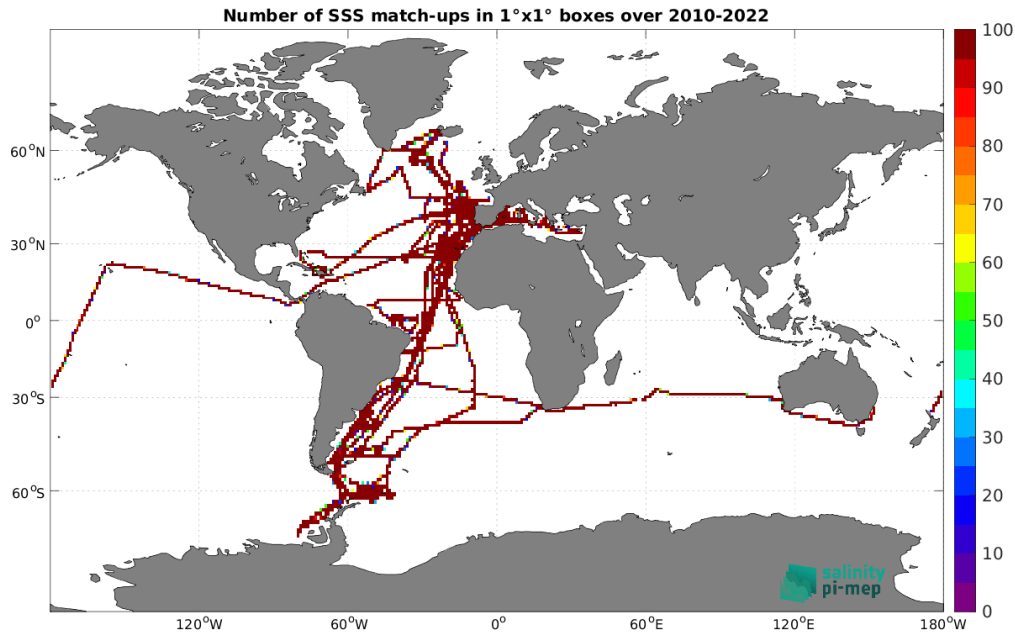
Figure 4: Number of SSS match-ups between TSG (CSIC-UTM) SSS and the SMOS SSS L3 v8 - 18 Days (CATDS-CEC-LOCEAN) SSS product for the Global Ocean Pi-MEP region over 1^\circ \times 1^\circ boxes and for the full satellite product period.
