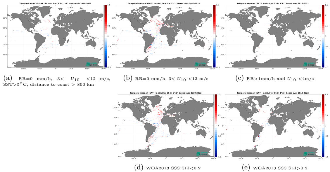
Figure 12: Temporal mean gridded over spatial boxes of size 1^\circ \times 1^\circ of \Delta SSS (SMOS SSS L3 v8 - 18 Days (CATDS-CEC-LOCEAN) - TSG (CSIC-UTM)) for 5 different subdatasets corresponding to:RR=0 mm/h, 3 < U_{10} < 12 m/s, SST >5^\circ C, distance to coast > 800 km (a), RR=0 mm/h, 3 < U_{10} < 12 m/s (b), RR >1 mm/h and U_{10} < 4 m/s (c), WOA2013 SSS Std <0.2 (d), WOA2013 SSS Std >0.2 (e).
