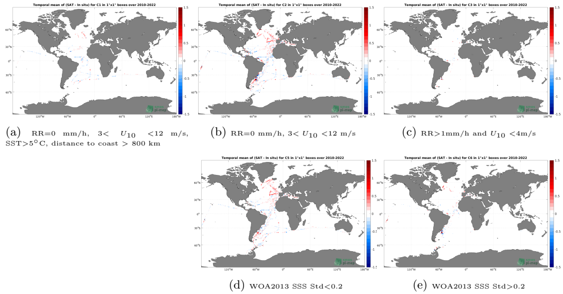
Figure 12: Temporal mean gridded over spatial boxes of size 1^\circ \times 1^\circ of \Delta SSS (SMOS SSS L3 v8 - 18 Days (CATDS-CECOS-LOCEAN) - TSG (CSIC-UTM)) for 5 different subdatasets corresponding to:RR=0 mm/h, 3 < U_{10} < 12 m/s, SST >5^\circ C, distance to coast > 800 km (a), RR=0 mm/h, 3 < U_{10} < 12 m/s (b), RR >1 mm/h and U_{10} < 4 m/s (c), WOA2013 SSS Std <0.2 (d), WOA2013 SSS Std >0.2 (e).
