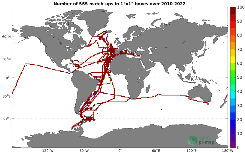
Figure 4: Number of SSS match-ups between TSG (CSIC-UTM) SSS and the SMOS SSS L3 v8 - 18 Days (CATDS-CECOS-LOCEAN) SSS product for the Global Ocean Pi-MEP region over 1^\circ \times 1^\circ boxes and for the full satellite product period.
