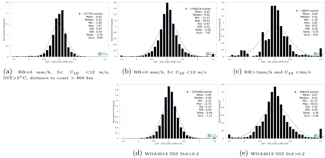
Figure 13: Normalized histogram of \Delta SSS (SMOS SSS L3 v8 - 18 Days (CATDS-CECOS-LOCEAN) - TSG (CSIC-UTM)) for 5 different subdatasets corresponding to: RR=0 mm/h, 3 < U_{10} < 12 m/s, SST>5°C, distance to coast > 800 km (a), RR=0 mm/h, 3 < U_{10} < 12 m/s (b), RR>1mm/h and U_{10} < 4 m/s (c), WOA2013 SSS Std<0.2 (d), WOA2013 SSS Std>0.2 (e).
