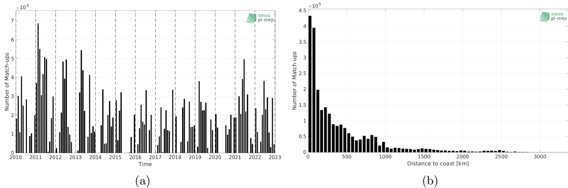
Figure 1: Number of match-ups between TSG (CSIC-UTM) and SMOS SSS L3 v8 - 18 Days (CATDS-CECOS-LOCEAN) SSS as a function of time (a) and as function of the distance to coast (b) over the Global Ocean Pi-MEP region and for the full satellite product period.
