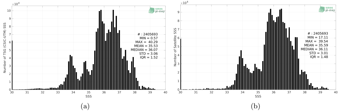
Figure 2: Histograms of SSS from TSG (CSIC-UTM) (a) and SMOS SSS L3 v8 - 18 Days (CATDS-CECOS-LOCEAN) (b) considering all match-up pairs per bins of 0.1 over the Global Ocean Pi-MEP region and for the full satellite product period.
