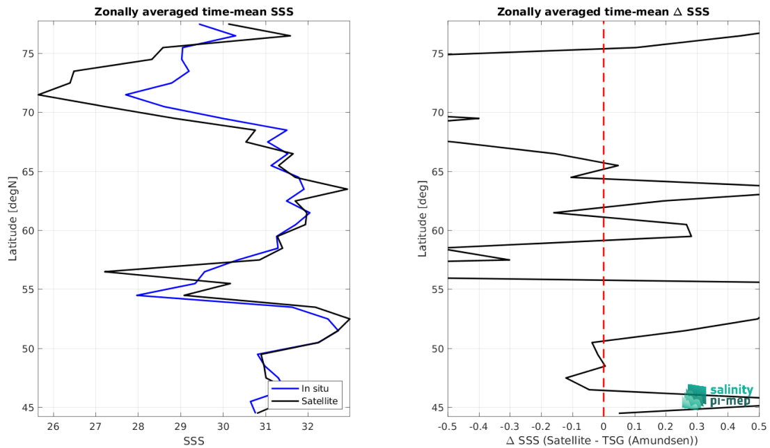
Figure 8: Left panel: Zonal mean SSS from SMOS SSS L3 v8 - 18 Days (CATDS-CEC-LOCEAN) satellite product (black) and from TSG (Amundsen) (blue). Right panel: Zonal mean of \Delta SSS (Satellite - TSG (Amundsen)) for all the collected Pi-MEP match-up pairs estimated over the full satellite product period.
