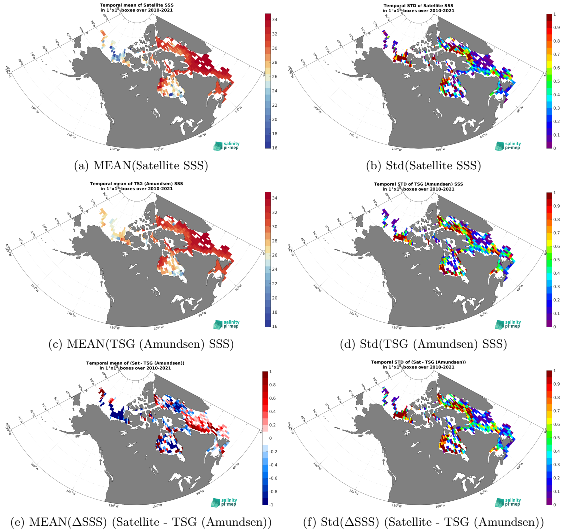
Figure 6: Temporal mean (left) and Std (right) of SSS from SMOS SSS L3 v8 - 18 Days (CATDS-CEC-LOCEAN) (top), TSG (Amundsen) (middle), and of \Delta SSS (Satellite - TSG (Amundsen)). Only match-up pairs are used to generate these maps.
