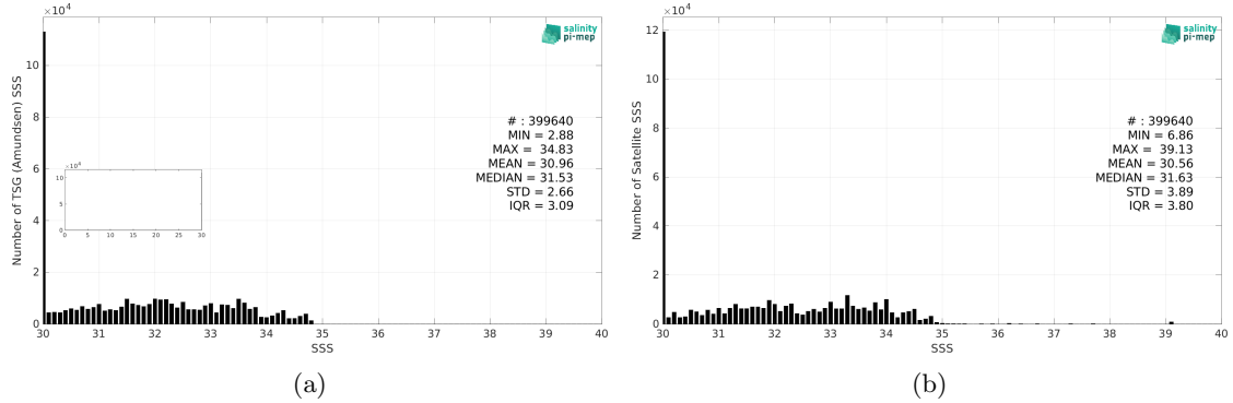
Figure 2: Histograms of SSS from TSG (Amundsen) (a) and SMOS SSS L3 v8 - 18 Days (CATDS-CEC-LOCEAN) (b) considering all match-up pairs per bins of 0.1 over the Global Ocean Pi-MEP region and for the full satellite product period.
