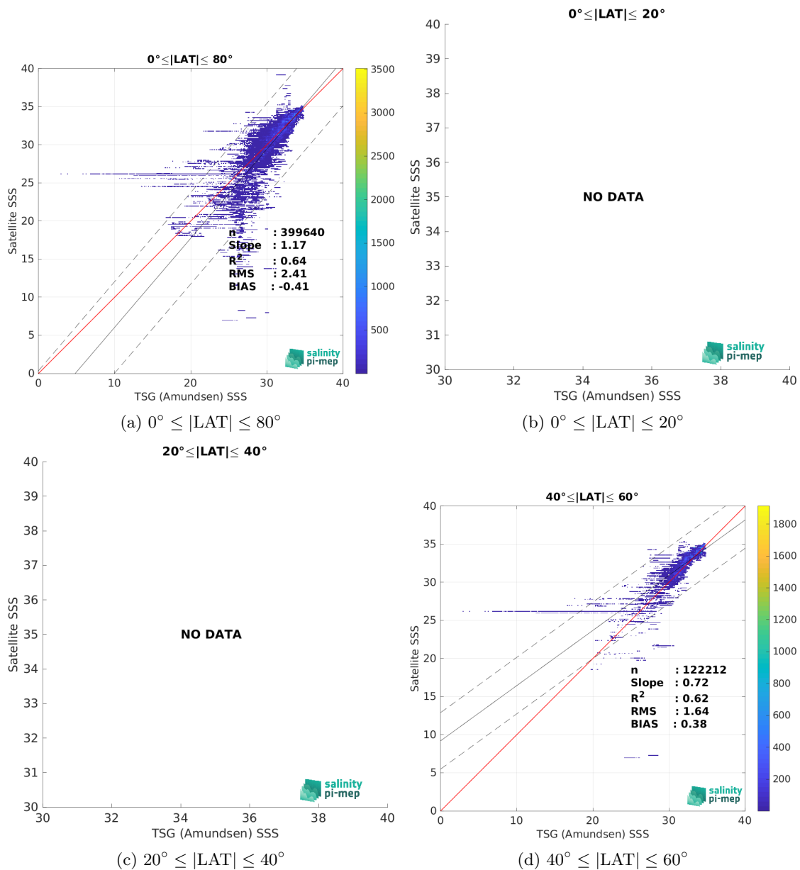
Figure 9: Contour maps of the concentration of SMOS SSS L3 v8 - 18 Days (CATDS-CEC-LOCEAN) SSS (y-axis) versus TSG (Amundsen) SSS (x-axis) at match-up pairs for different latitude bands. For each plot, the red line shows x=y . The black thin and dashed lines indicate a linear fit through the data cloud and the \pm 95\% confidence levels, respectively. The number match-up pairs n , the slope and R^2 coefficient of the linear fit, the root mean square (RMS) and the mean bias between satellite and in situ data are indicated for each latitude band in each plots.
