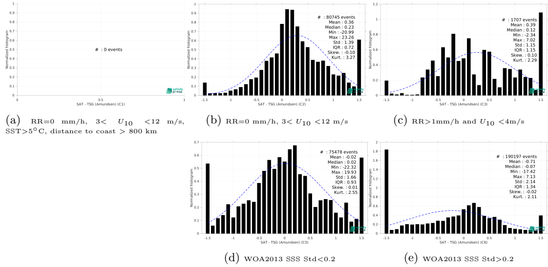
Figure 13: Normalized histogram of \Delta SSS (SMOS SSS L3 v8 - 18 Days (CATDS-CEC-LOCEAN) - TSG (Amundsen)) for 5 different subdatasets corresponding to: RR=0 mm/h, 3 < U_{10} < 12 m/s, SST>5°C, distance to coast > 800 km (a), RR=0 mm/h, 3 < U_{10} < 12 m/s (b), RR>1mm/h and U_{10} < 4 m/s (c), WOA2013 SSS Std<0.2 (d), WOA2013 SSS Std>0.2 (e).
