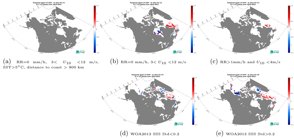
Figure 12: Temporal mean gridded over spatial boxes of size 1^{\circ}\times 1^{\circ} of \Delta\text{SSS} (SMOS SSS L3 v8 - 18 Days (CATDS-CEC-LOCEAN) - TSG (Amundsen)) for 5 different subdatasets corresponding to:RR=0 mm/h, 3 < U_{10} < 12 m/s, SST >5^{\circ}\text{C} , distance to coast > 800 km (a), RR=0 mm/h, 3 < U_{10} < 12 m/s (b), RR >1 mm/h and U_{10} < 4 m/s (c), WOA2013 SSS Std <0.2 (d), WOA2013 SSS Std >0.2 (e).
