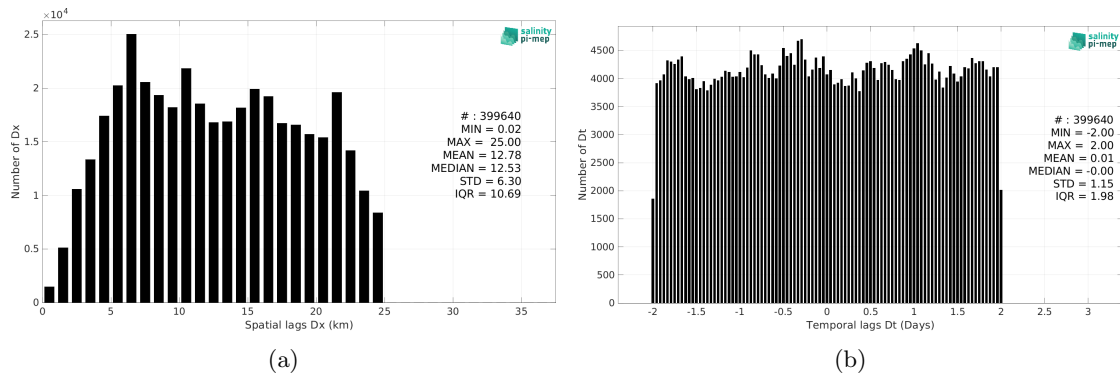
Figure 5: Histograms of the spatial (a) and temporal (b) lags between the location/time of the TSG (Amundsen) measurement and the date of the corresponding SMOS SSS L3 v8 - 18 Days (CATDS-CEC-LOCEAN) SSS pixel.
