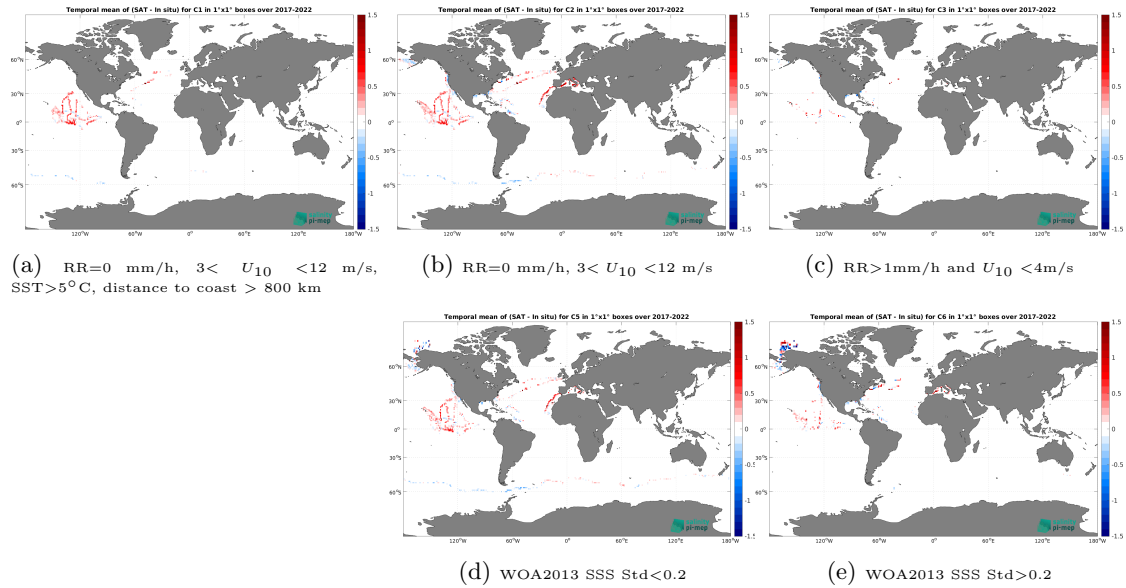
Figure 12: Temporal mean gridded over spatial boxes of size 1^\circ \times 1^\circ of \Delta SSS (SMOS SSS L3 v8 - 18 Days (CATDS-CEC-LOCEAN) - Sairdrone) for 5 different subdatasets corresponding to:RR=0 mm/h, 3 < U_{10} < 12 m/s, SST > 5^\circ\text{C} , distance to coast > 800 km (a), RR=0 mm/h, 3 < U_{10} < 12 m/s (b), RR > 1 mm/h and U_{10} < 4 m/s (c), WOA2013 SSS Std < 0.2 (d), WOA2013 SSS Std > 0.2 (e).
