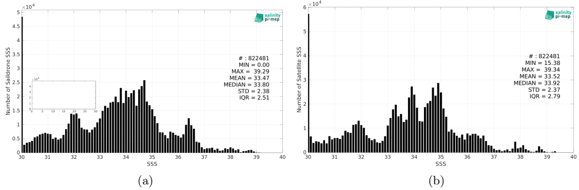
Figure 2: Histograms of SSS from Saildrone (a) and SMOS SSS L3 v8 - 18 Days (CATDS-CEC-LOCEAN) (b) considering all match-up pairs per bins of 0.1 over the Global Ocean Pi-MEP region and for the full satellite product period.
