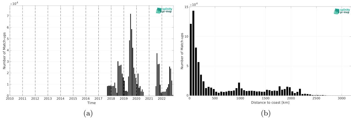
Figure 1: Number of match-ups between Saildrone and SMOS SSS L3 v8 - 18 Days (CATDS-CEC-LOCEAN) SSS as a function of time (a) and as function of the distance to coast (b) over the Global Ocean Pi-MEP region and for the full satellite product period.
