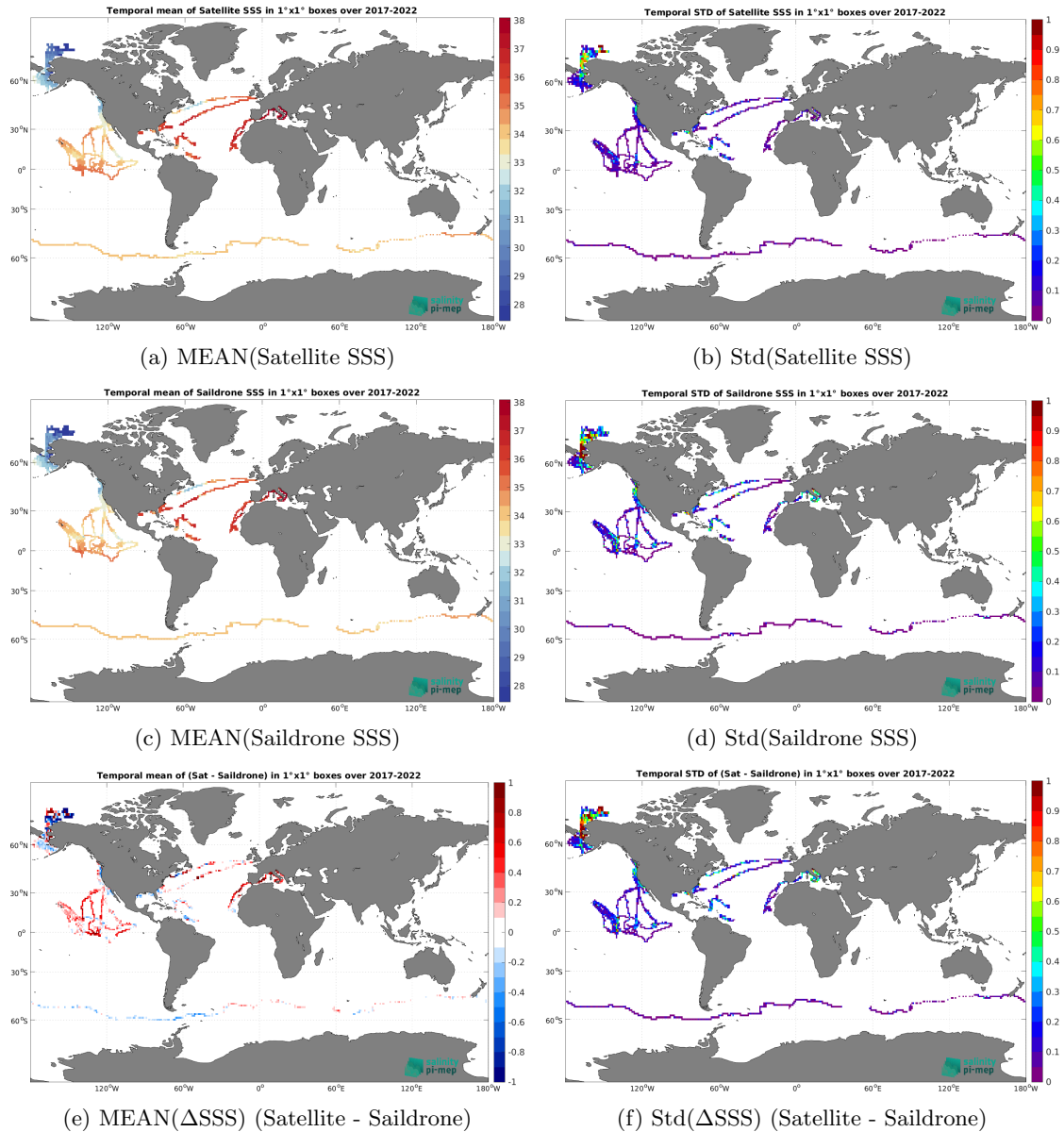
Figure 6: Temporal mean (left) and Std (right) of SSS from SMOS SSS L3 v8 - 18 Days (CATDS-CEC-LOCEAN) (top), Saildrone (middle), and of \Delta SSS (Satellite - Saildrone). Only match-up pairs are used to generate these maps.
