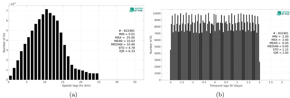
Figure 5: Histograms of the spatial (a) and temporal (b) lags between the location/time of the Sailability measurement and the date of the corresponding SMOS SSS L3 v8 - 18 Days (CATDS-CEC-LOCEAN) SSS pixel.
