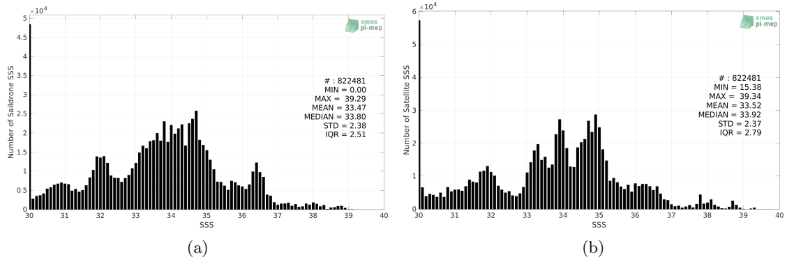
Figure 2: Histograms of SSS from Saifdrone (a) and SMOS SSS L3 v8 - 18 Days (CATDS-CECOS-LOCEAN) (b) considering all match-up pairs per bins of 0.1 over the Global Ocean Pi-MEP region and for the full satellite product period.
