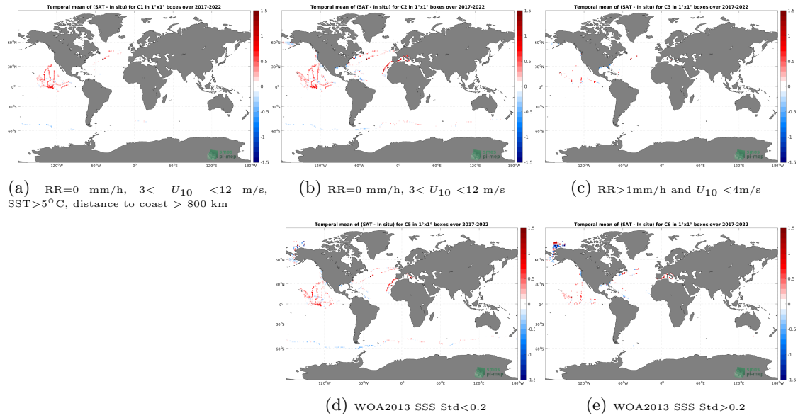
Figure 12: Temporal mean gridded over spatial boxes of size 1^\circ \times 1^\circ of \Delta SSS (SMOS SSS L3 v8 - 18 Days (CATDS-CECOS-LOCEAN) - Sairdrone) for 5 different subdatasets corresponding to:RR=0 mm/h, 3 < U_{10} < 12 m/s, SST >5^\circ C, distance to coast > 800 km (a), RR=0 mm/h, 3 < U_{10} < 12 m/s (b), RR >1 mm/h and U_{10} < 4 m/s (c), WOA2013 SSS Std <0.2 (d), WOA2013 SSS Std >0.2 (e).
