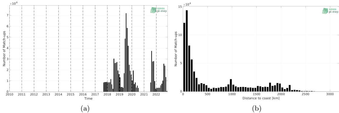
Figure 1: Number of match-ups between Saildrone and SMOS SSS L3 v8 - 18 Days (CATDS-CECOS-LOCEAN) SSS as a function of time (a) and as function of the distance to coast (b) over the Global Ocean Pi-MEP region and for the full satellite product period.
