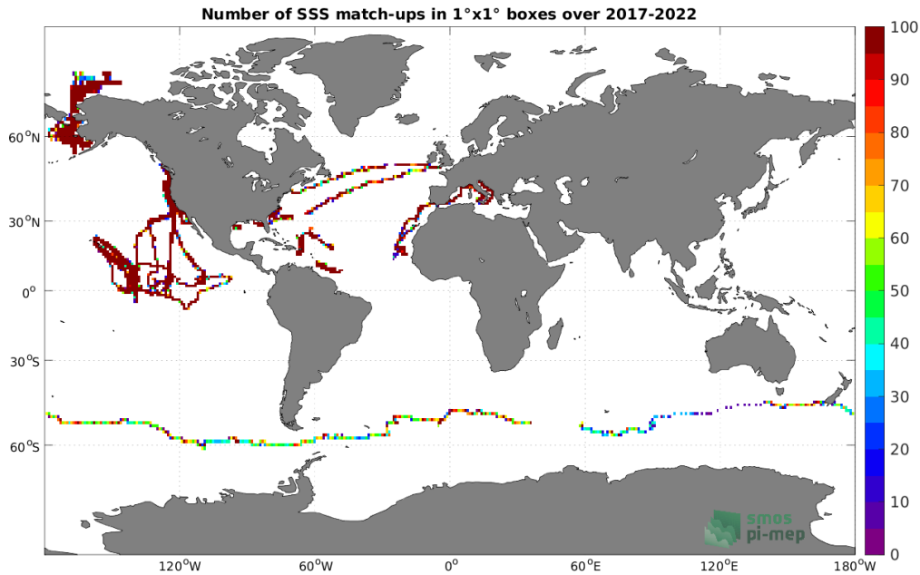
Figure 4: Number of SSS match-ups between Sairdrone SSS and the SMOS SSS L3 v8 - 18 Days (CATDS-CECOS-LOCEAN) SSS product for the Global Ocean Pi-MEP region over 1^\circ \times 1^\circ boxes and for the full satellite product period.
