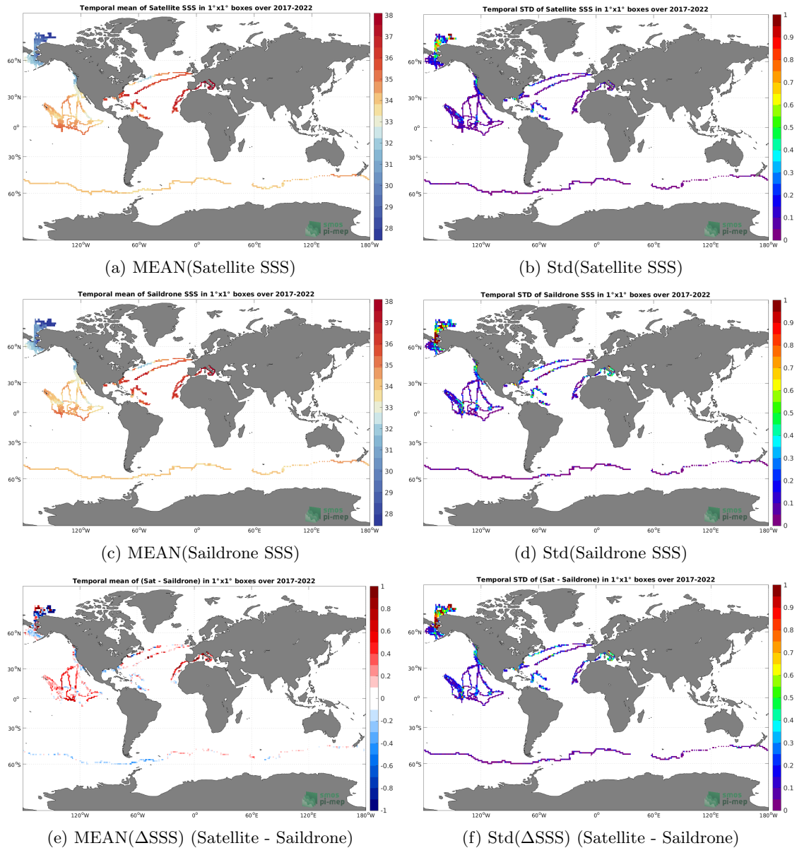
Figure 6: Temporal mean (left) and Std (right) of SSS from SMOS SSS L3 v8 - 18 Days (CATDS-CECOS-LOCEAN) (top), Saildrone (middle), and of \Delta SSS (Satellite - Saildrone). Only match-up pairs are used to generate these maps.
