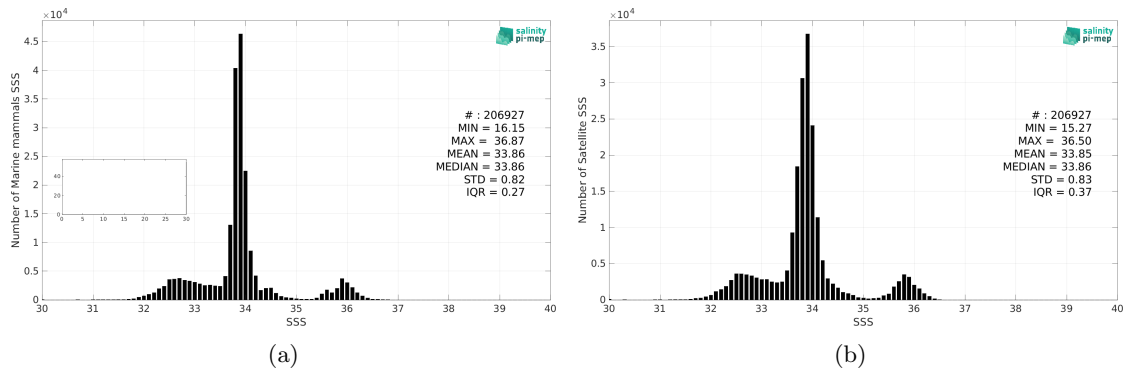
Figure 2: Histograms of SSS from Marine mammals (a) and SMOS SSS L3 v8 - 18 Days (CATDS-CEC-LOCEAN) (b) considering all match-up pairs per bins of 0.1 over the Global Ocean Pi-MEP region and for the full satellite product period.
