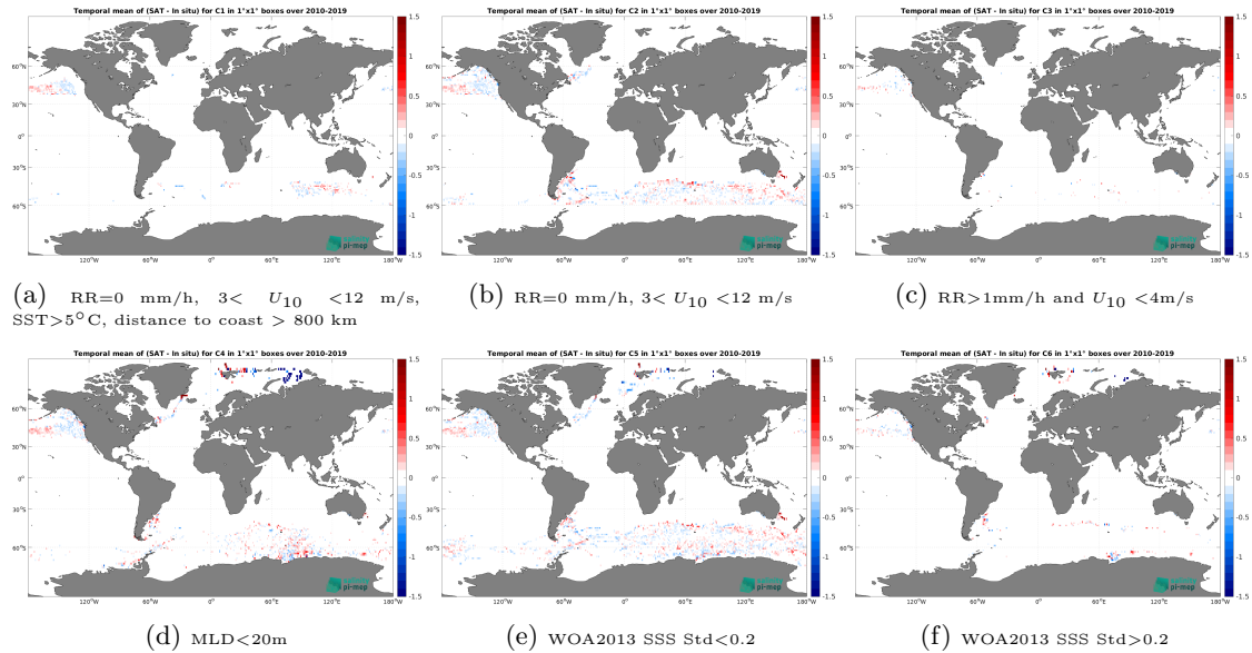
Figure 12: Temporal mean gridded over spatial boxes of size 1^{\circ}\times 1^{\circ} of \Delta\text{SSS} (SMOS SSS L3 v8 - 18 Days (CATDS-CEC-LOCEAN) - Marine mammals) for 6 different subdatasets corresponding to:RR=0 mm/h, 3 < U_{10} < 12 m/s, SST >5^{\circ}\text{C} , distance to coast > 800 km (a), RR=0 mm/h, 3 < U_{10} < 12 m/s (b), RR >1 mm/h and U_{10} < 4 m/s (c),MLD <20 m (d),WOA2013 SSS Std <0.2 (e),WOA2013 SSS Std >0.2 (f).
