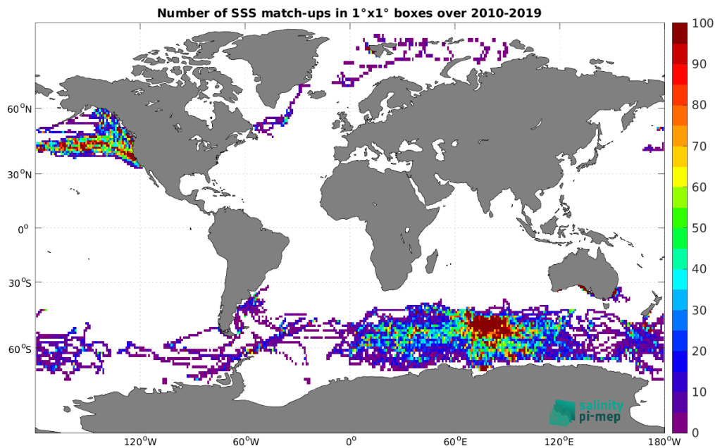
Figure 4: Number of SSS match-ups between Marine mammals SSS and the SMOS SSS L3 v8 - 18 Days (CATDS-CEC-LOCEAN) SSS product for the Global Ocean Pi-MEP region over 1^\circ \times 1^\circ boxes and for the full satellite product period.
