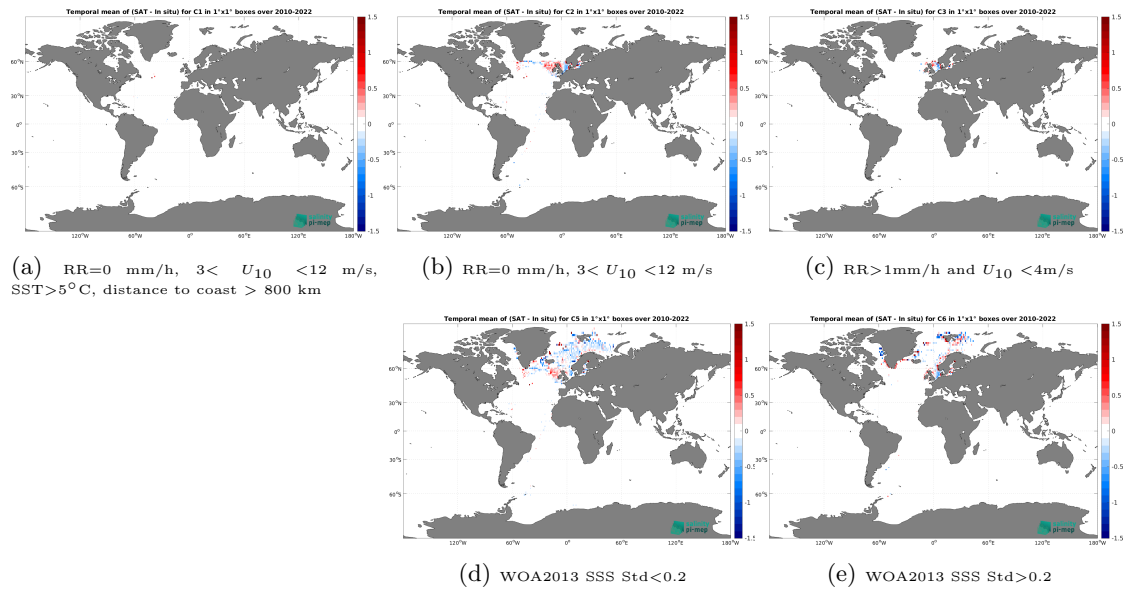
Figure 12: Temporal mean gridded over spatial boxes of size 1^\circ \times 1^\circ of \Delta SSS (SMOS SSS L3 v8 - 18 Days (CATDS-CEC-LOCEAN) - ICES) for 5 different subdatasets corresponding to:RR=0 mm/h, 3 < U_{10} < 12 m/s, SST >5^\circ C, distance to coast > 800 km (a), RR=0 mm/h, 3 < U_{10} < 12 m/s (b), RR >1 mm/h and U_{10} < 4 m/s (c), WOA2013 SSS Std <0.2 (d), WOA2013 SSS Std >0.2 (e).
