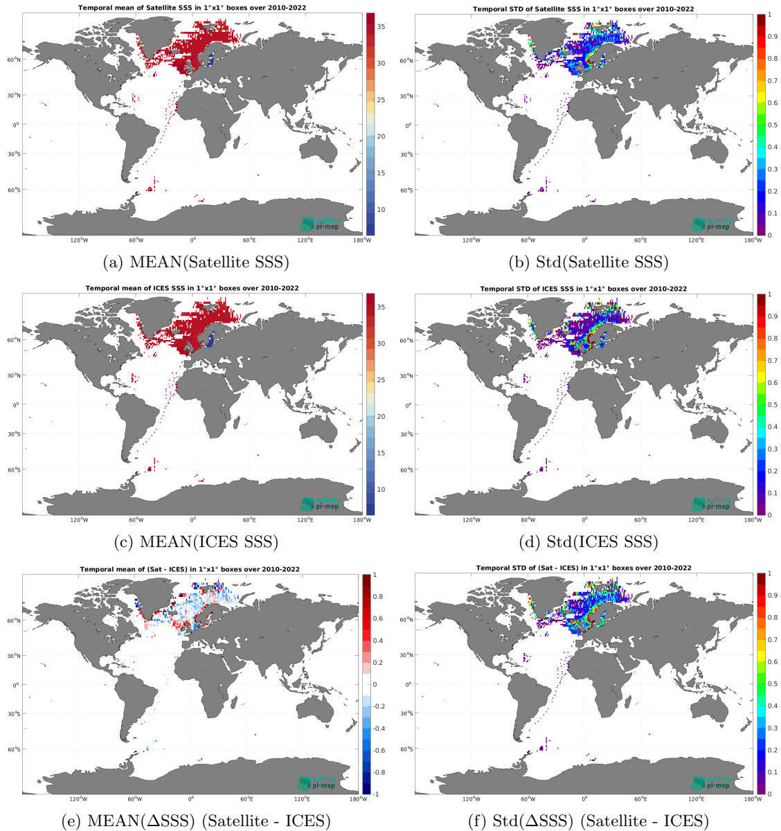
Figure 6: Temporal mean (left) and Std (right) of SSS from SMOS SSS L3 v8 - 18 Days (CATDS-CEC-LOCEAN) (top), ICES (middle), and of \Delta SSS (Satellite - ICES). Only match-up pairs are used to generate these maps.
