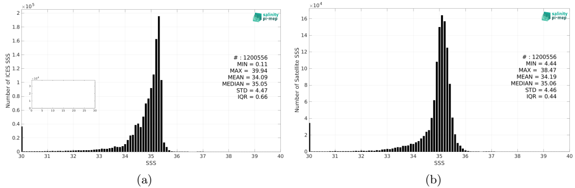
Figure 2: Histograms of SSS from ICES (a) and SMOS SSS L3 v8 - 18 Days (CATDS-CEC-LOCEAN) (b) considering all match-up pairs per bins of 0.1 over the Global Ocean Pi-MEP region and for the full satellite product period.
