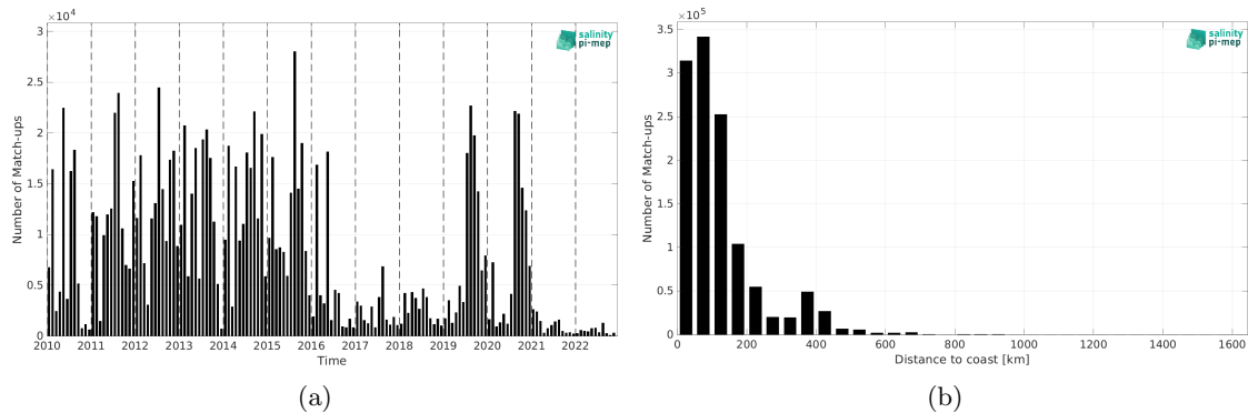
Figure 1: Number of match-ups between ICES and SMOS SSS L3 v8 - 18 Days (CATDS-CEC-LOCEAN) SSS as a function of time (a) and as function of the distance to coast (b) over the Global Ocean Pi-MEP region and for the full satellite product period.
