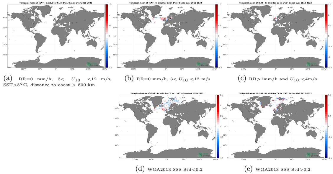
Figure 12: Temporal mean gridded over spatial boxes of size 1^\circ \times 1^\circ of \Delta SSS (SMOS SSS L3 v8 - 18 Days (CATDS-CECOS-LOCEAN) - ICES) for 5 different subdatasets corresponding to:RR=0 mm/h, 3 < U_{10} < 12 m/s, SST > 5^\circ\text{C} , distance to coast > 800 km (a), RR=0 mm/h, 3 < U_{10} < 12 m/s (b), RR > 1 mm/h and U_{10} < 4 m/s (c), WOA2013 SSS Std < 0.2 (d), WOA2013 SSS Std > 0.2 (e).
