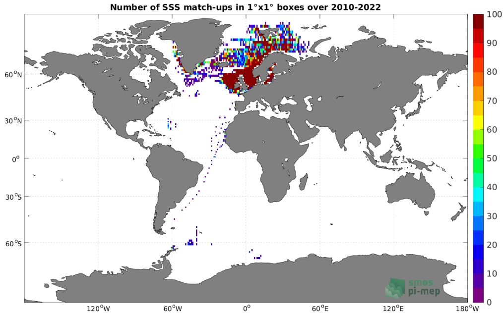
Figure 4: Number of SSS match-ups between ICES SSS and the SMOS SSS L3 v8 - 18 Days (CATDS-CECOS-LOCEAN) SSS product for the Global Ocean Pi-MEP region over 1^\circ \times 1^\circ boxes and for the full satellite product period.
