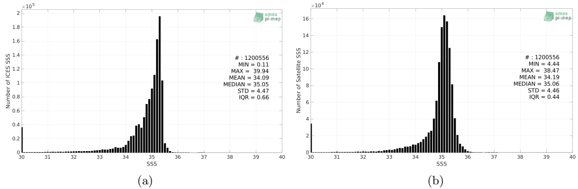
Figure 2: Histograms of SSS from ICES (a) and SMOS SSS L3 v8 - 18 Days (CATDS-CECOS-LOCEAN) (b) considering all match-up pairs per bins of 0.1 over the Global Ocean Pi-MEP region and for the full satellite product period.
