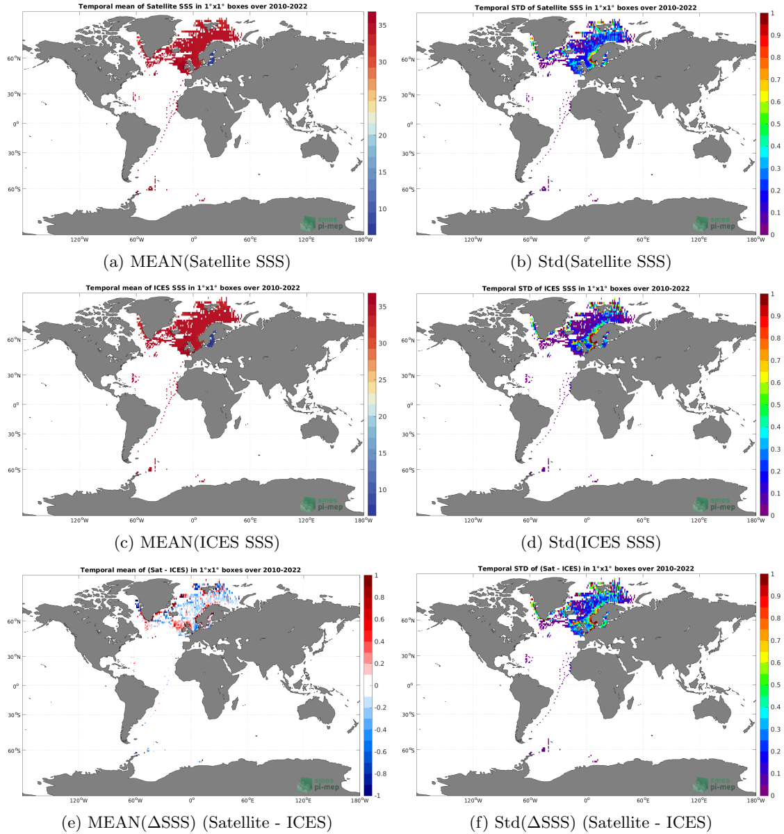
Figure 6: Temporal mean (left) and Std (right) of SSS from SMOS SSS L3 v8 - 18 Days (CATDS-CECOS-LOCEAN) (top), ICES (middle), and of \Delta SSS (Satellite - ICES). Only match-up pairs are used to generate these maps.
