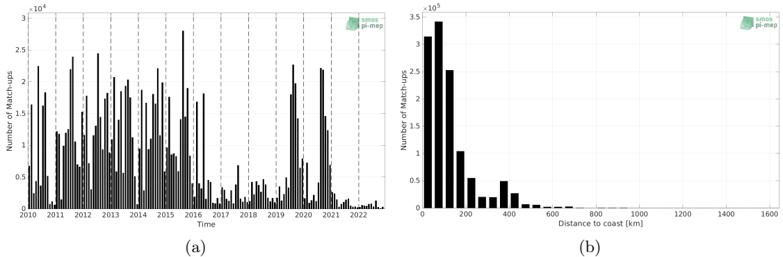
Figure 1: Number of match-ups between ICES and SMOS SSS L3 v8 - 18 Days (CATDS-CECOS-LOCEAN) SSS as a function of time (a) and as function of the distance to coast (b) over the Global Ocean Pi-MEP region and for the full satellite product period.
