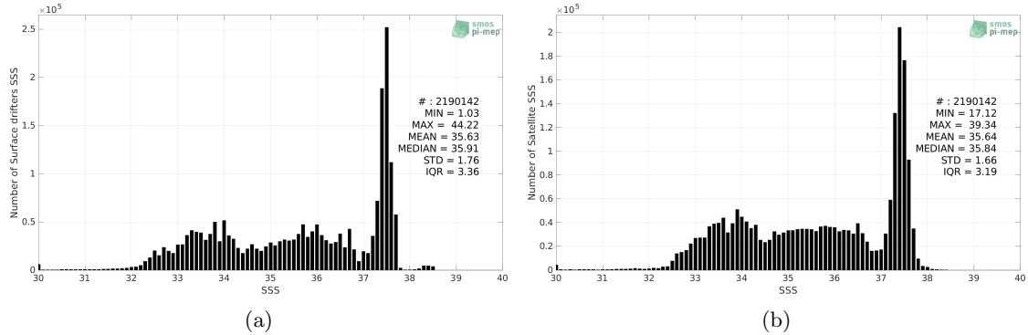
Figure 2: Histograms of SSS from Surface drifters (a) and SMOS SSS L3 v8 - 18 Days (CATDS-CECOS-LOCEAN) (b) considering all match-up pairs per bins of 0.1 over the Global Ocean Pi-MEP region and for the full satellite product period.
