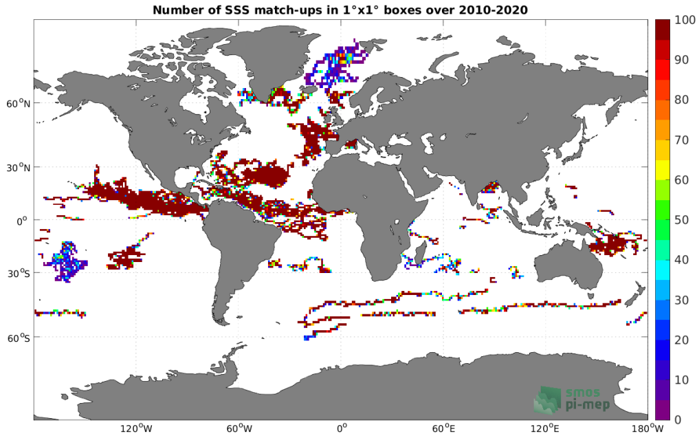
Figure 3: Number of SSS match-ups between Surface drifters SSS and the SMOS SSS L3 v8 - 18 Days (CATDS-CECOS-LOCEAN) SSS product for the Global Ocean Pi-MEP region over 1^\circ \times 1^\circ boxes and for the full satellite product period.
