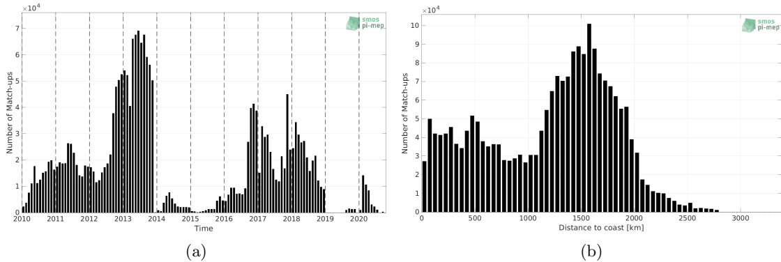
Figure 1: Number of match-ups between Surface drifters and SMOS SSS L3 v8 - 18 Days (CATDS-CECOS-LOCEAN) SSS as a function of time (a) and as function of the distance to coast (b) over the Global Ocean Pi-MEP region and for the full satellite product period.
