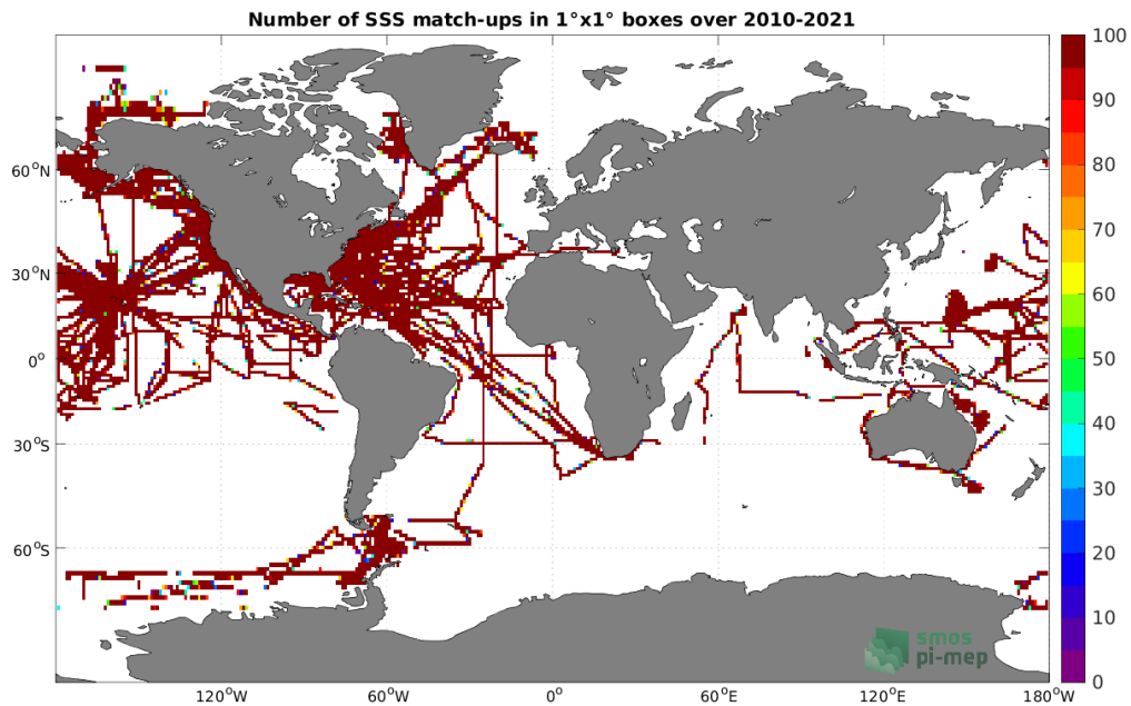
Figure 3: Number of SSS match-ups between TSG (SAMOS) SSS and the SMOS SSS L3 v7 - 9 Days (CATDS-CECOS-LOCEAN) SSS product for the Global Ocean Pi-MEP region over 1^\circ \times 1^\circ boxes and for the full satellite product period.
