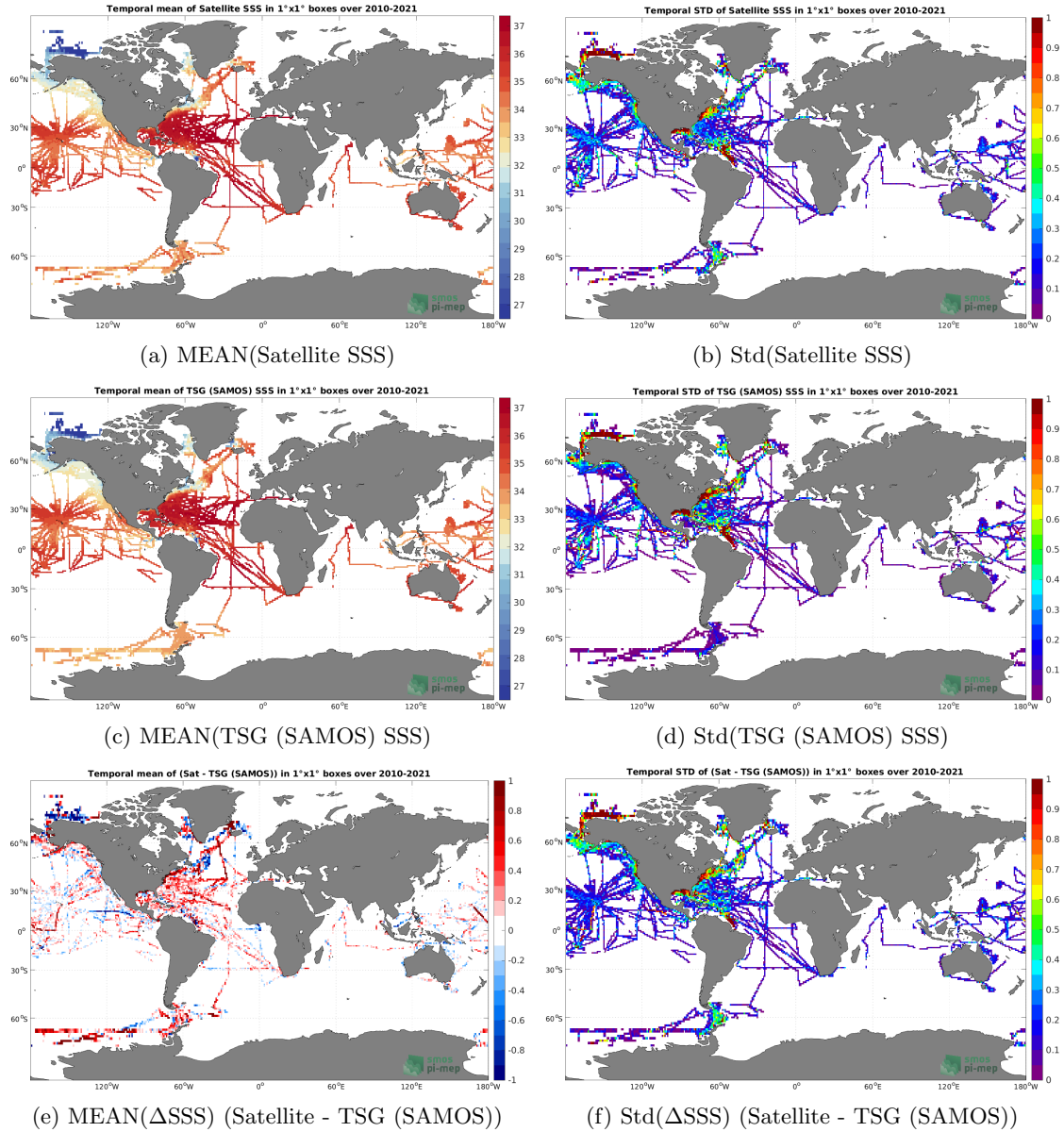
Figure 5: Temporal mean (left) and Std (right) of SSS from SMOS SSS L3 v7 - 9 Days (CATDS-CECOS-LOCEAN) (top), TSG (SAMOS) (middle), and of \Delta SSS (Satellite - TSG (SAMOS)). Only match-up pairs are used to generate these maps.
