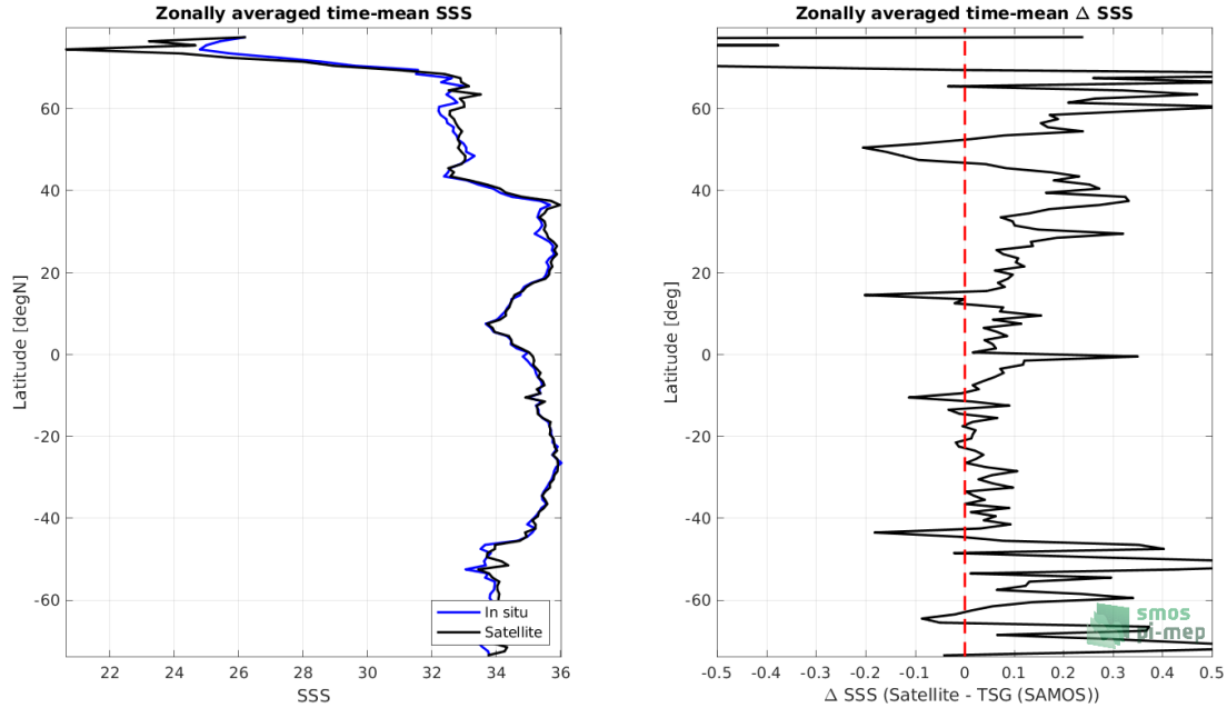
Figure 7: Left panel: Zonal mean SSS from SMOS SSS L3 v7 - 9 Days (CATDS-CECOS-LOCEAN) satellite product (black) and from TSG (SAMOS) (blue). Right panel: Zonal mean of \Delta SSS (Satellite - TSG (SAMOS)) for all the collected Pi-MEP match-up pairs estimated over the full satellite product period.
