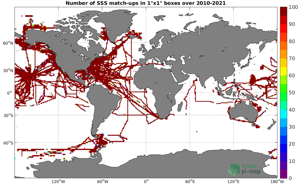
Figure 4: Number of SSS match-ups between TSG (SAMOS) SSS and the SMOS SSS L3 v7 - 9 Days (CATDS-CECOS-LOCEAN) SSS product for the Global Ocean Pi-MEP region over 1^\circ \times 1^\circ boxes and for the full satellite product period.
