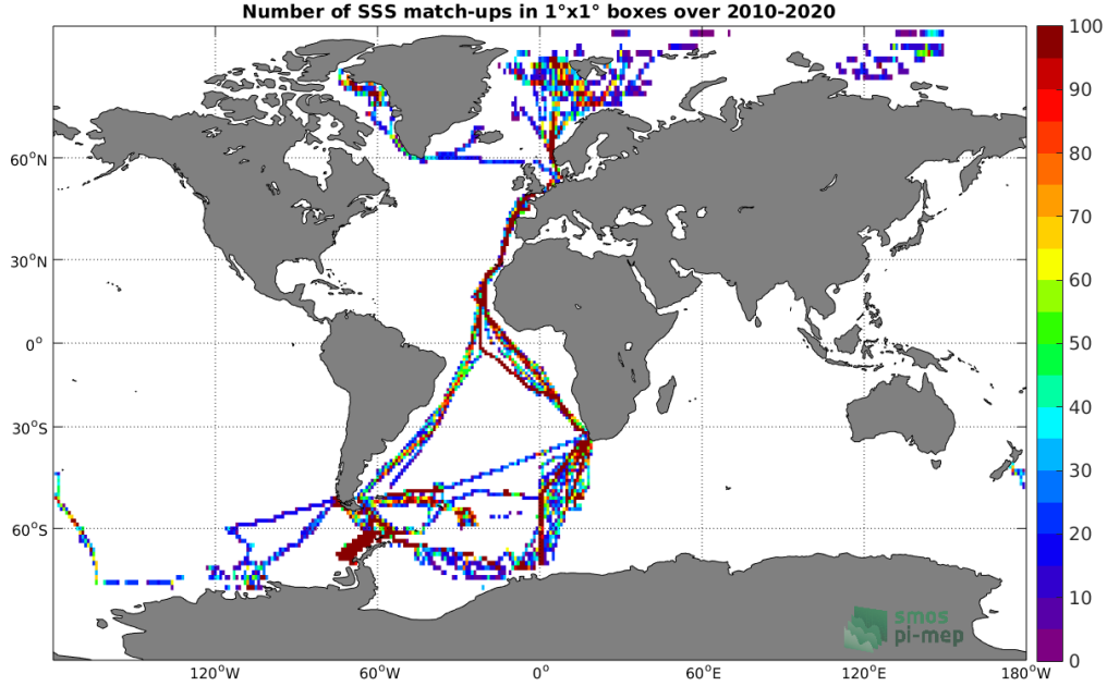
Figure 4: Number of SSS match-ups between TSG (Polarstern) SSS and the SMOS SSS L3 v7 - 9 Days (CATDS-CECOS-LOCEAN) SSS product for the Global Ocean Pi-MEP region over 1^\circ \times 1^\circ boxes and for the full satellite product period.
