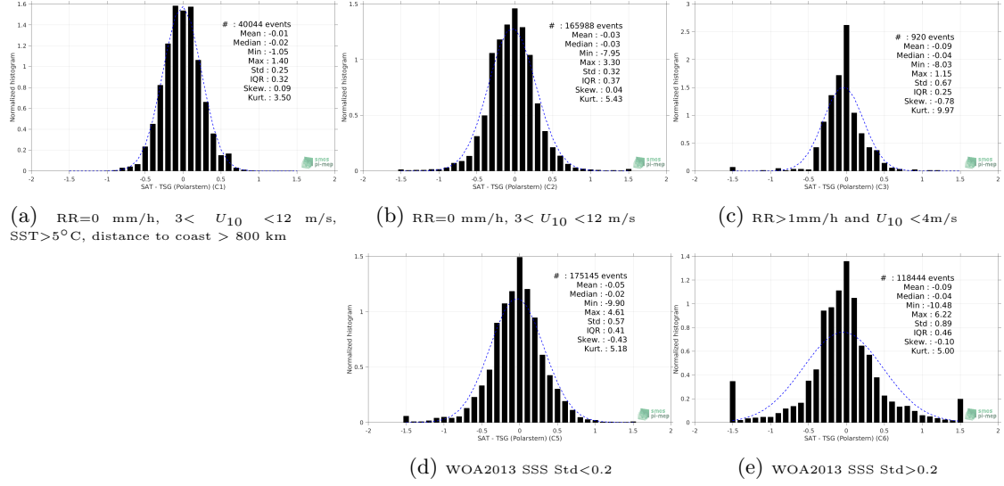
Figure 13: Normalized histogram of \Delta SSS (SMOS SSS L3 v7 - 9 Days (CATDS-CECOS-LOCEAN) - TSG (Polarstern)) for 5 different subdatasets corresponding to: RR=0 mm/h, 3 < U_{10} < 12 m/s, SST>5°C, distance to coast > 800 km (a), RR=0 mm/h, 3 < U_{10} < 12 m/s (b), RR>1mm/h and U_{10} < 4 m/s (c), WOA2013 SSS Std<0.2 (d), WOA2013 SSS Std>0.2 (e).
