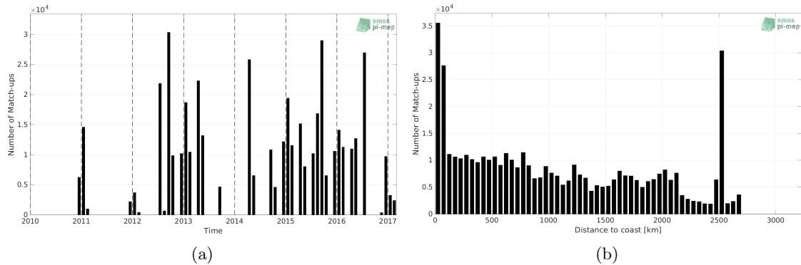
Figure 1: Number of match-ups between TSG (NCEI-0170743) and SMOS SSS L3 v7 - 9 Days (CATDS-CECOS-LOCEAN) SSS as a function of time (a) and as function of the distance to coast (b) over the Global Ocean Pi-MEP region and for the full satellite product period.
