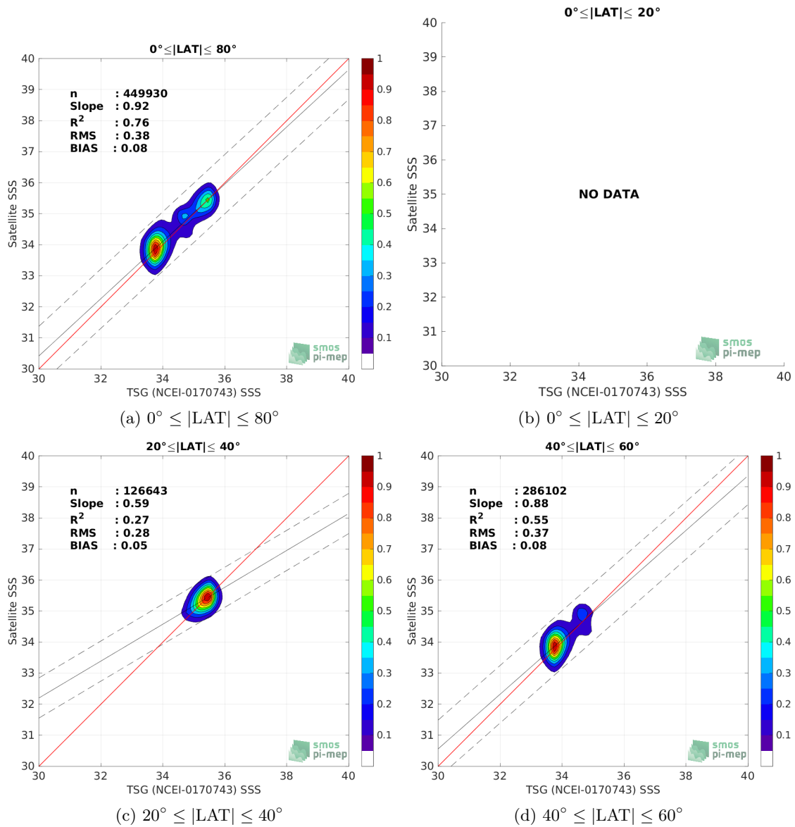
Figure 9: Contour maps of the concentration of SMOS SSS L3 v7 - 9 Days (CATDS-CECOS-LOCEAN) SSS (y-axis) versus TSG (NCEI-0170743) SSS (x-axis) at match-up pairs for different latitude bands. For each plot, the red line shows x=y . The black thin and dashed lines indicate a linear fit through the data cloud and the \pm 95\% confidence levels, respectively. The number match-up pairs n , the slope and R^2 coefficient of the linear fit, the root mean square (RMS) and the mean bias between satellite and in situ data are indicated for each latitude band in each plots.
