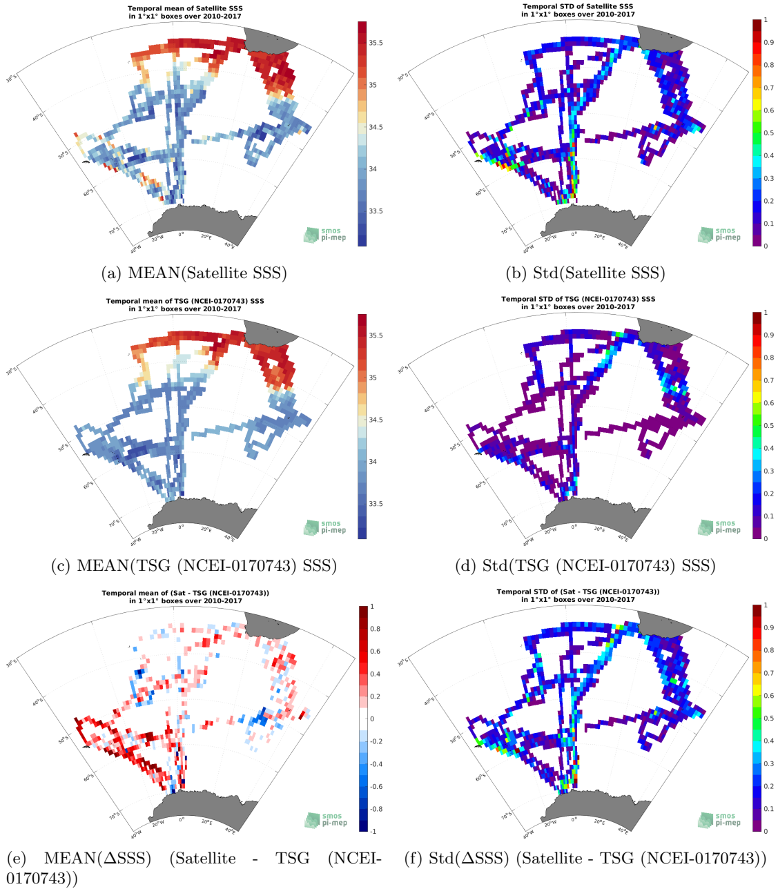
Figure 6: Temporal mean (left) and Std (right) of SSS from SMOS SSS L3 v7 - 9 Days (CATDS-CECOS-LOCEAN) (top), TSG (NCEI-0170743) (middle), and of \Delta SSS (Satellite - TSG (NCEI-0170743)). Only match-up pairs are used to generate these maps.
