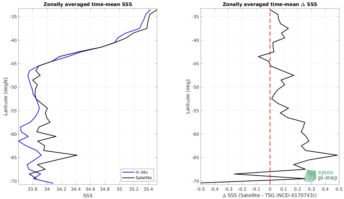
Figure 8: Left panel: Zonal mean SSS from SMOS SSS L3 v7 - 9 Days (CATDS-CECOS-LOCEAN) satellite product (black) and from TSG (NCEI-0170743) (blue). Right panel: Zonal mean of \Delta SSS (Satellite - TSG (NCEI-0170743)) for all the collected Pi-MEP match-up pairs estimated over the full satellite product period.
