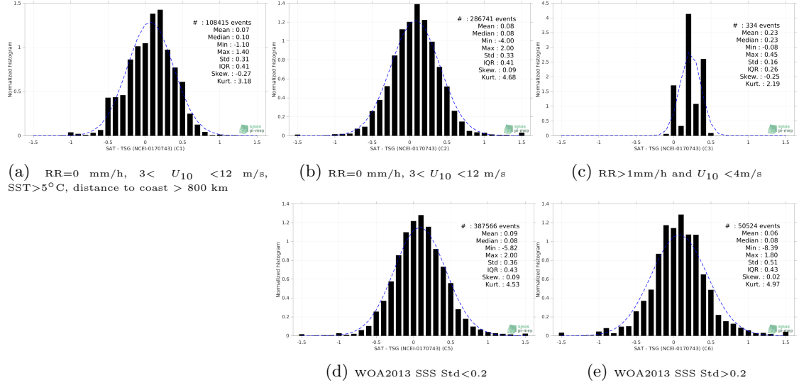
Figure 13: Normalized histogram of \Delta SSS (SMOS SSS L3 v7 - 9 Days (CATDS-CECOS-LOCEAN) - TSG (NCEI-0170743)) for 5 different subdatasets corresponding to: RR=0 mm/h, 3 < U_{10} < 12 m/s, SST>5°C, distance to coast > 800 km (a), RR=0 mm/h, 3 < U_{10} < 12 m/s (b), RR>1mm/h and U_{10} < 4 m/s (c), WOA2013 SSS Std<0.2 (d), WOA2013 SSS Std>0.2 (e).
