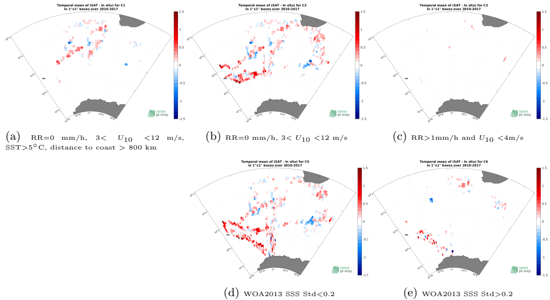
Figure 12: Temporal mean gridded over spatial boxes of size 1^{\circ}\times 1^{\circ} of \Delta\text{SSS} (SMOS SSS L3 v7 - 9 Days (CATDS-CECOS-LOCEAN) - TSG (NCEI-0170743)) for 5 different subdatasets corresponding to:RR=0 mm/h, 3 < U_{10} < 12 m/s, SST >5^{\circ}\text{C} , distance to coast > 800 km (a), RR=0 mm/h, 3 < U_{10} < 12 m/s (b), RR >1 mm/h and U_{10} < 4 m/s (c), WOA2013 SSS Std <0.2 (d), WOA2013 SSS Std >0.2 (e).
