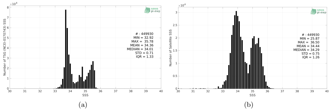
Figure 2: Histograms of SSS from TSG (NCEI-0170743) (a) and SMOS SSS L3 v7 - 9 Days (CATDS-CECOS-LOCEAN) (b) considering all match-up pairs per bins of 0.1 over the Global Ocean Pi-MEP region and for the full satellite product period.
