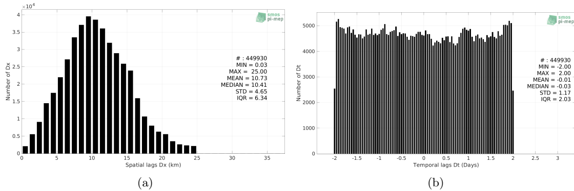
Figure 5: Histograms of the spatial (a) and temporal (b) lags between the location/time of the TSG (NCEI-0170743) measurement and the date of the corresponding SMOS SSS L3 v7 - 9 Days (CATDS-CECOS-LOCEAN) SSS pixel.
