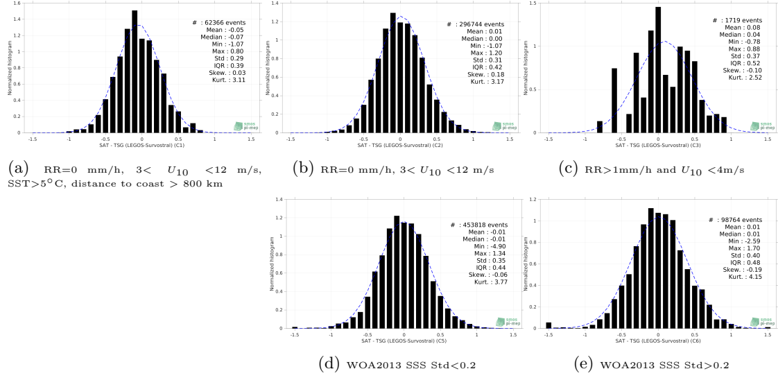
Figure 13: Normalized histogram of \Delta SSS (SMOS SSS L3 v7 - 9 Days (CATDS-CECOS-LOCEAN) - TSG (LEGOS-Survostral)) for 5 different subdatasets corresponding to: RR=0 mm/h, 3 < U_{10} < 12 m/s, SST>5°C, distance to coast > 800 km (a), RR=0 mm/h, 3 < U_{10} < 12 m/s (b), RR>1mm/h and U_{10} < 4 m/s (c), WOA2013 SSS Std<0.2 (d), WOA2013 SSS Std>0.2 (e).
