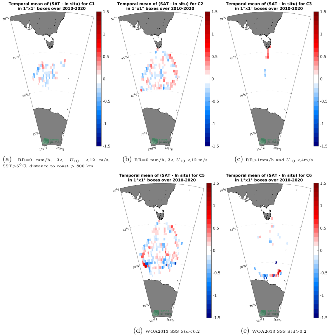
Figure 12: Temporal mean gridded over spatial boxes of size 1^\circ \times 1^\circ of \Delta SSS (SMOS SSS L3 v7 - 9 Days (CATDS-CECOS-LOCEAN) - TSG (LEGOS-Survostral)) for 5 different subdatasets corresponding to:RR=0 mm/h, 3 < U_{10} < 12 m/s, SST>5°C, distance to coast > 800 km (a), RR=0 mm/h, 3 < U_{10} < 12 m/s (b), RR>1mm/h and U_{10} < 4 m/s (c), WOA2013 SSS Std<0.2 (d), WOA2013 SSS Std>0.2 (e).
