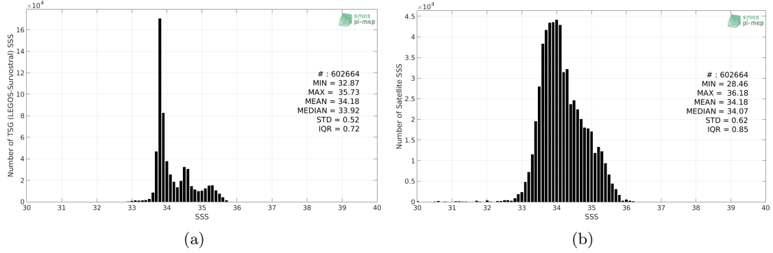
Figure 2: Histograms of SSS from TSG (LEGOS-Survostral) (a) and SMOS SSS L3 v7 - 9 Days (CATDS-CECOS-LOCEAN) (b) considering all match-up pairs per bins of 0.1 over the Global Ocean Pi-MEP region and for the full satellite product period.
