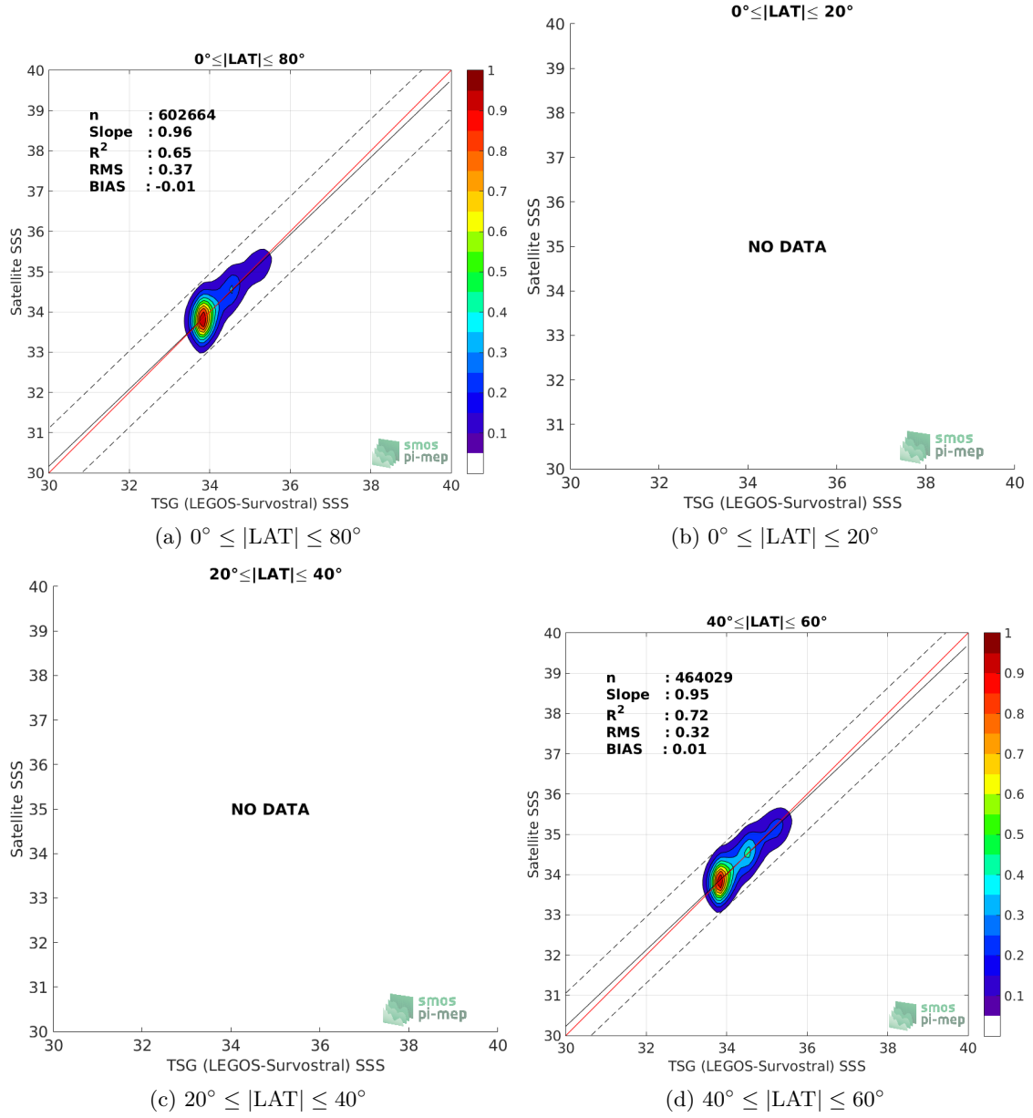
Figure 9: Contour maps of the concentration of SMOS SSS L3 v7 - 9 Days (CATDS-CECOS-LOCEAN) SSS (y-axis) versus TSG (LEGOS-Survostral) SSS (x-axis) at match-up pairs for different latitude bands. For each plot, the red line shows x=y . The black thin and dashed lines indicate a linear fit through the data cloud and the \pm 95\% confidence levels, respectively. The number match-up pairs n , the slope and R^2 coefficient of the linear fit, the root mean square (RMS) and the mean bias between satellite and in situ data are indicated for each latitude band in each plots.
