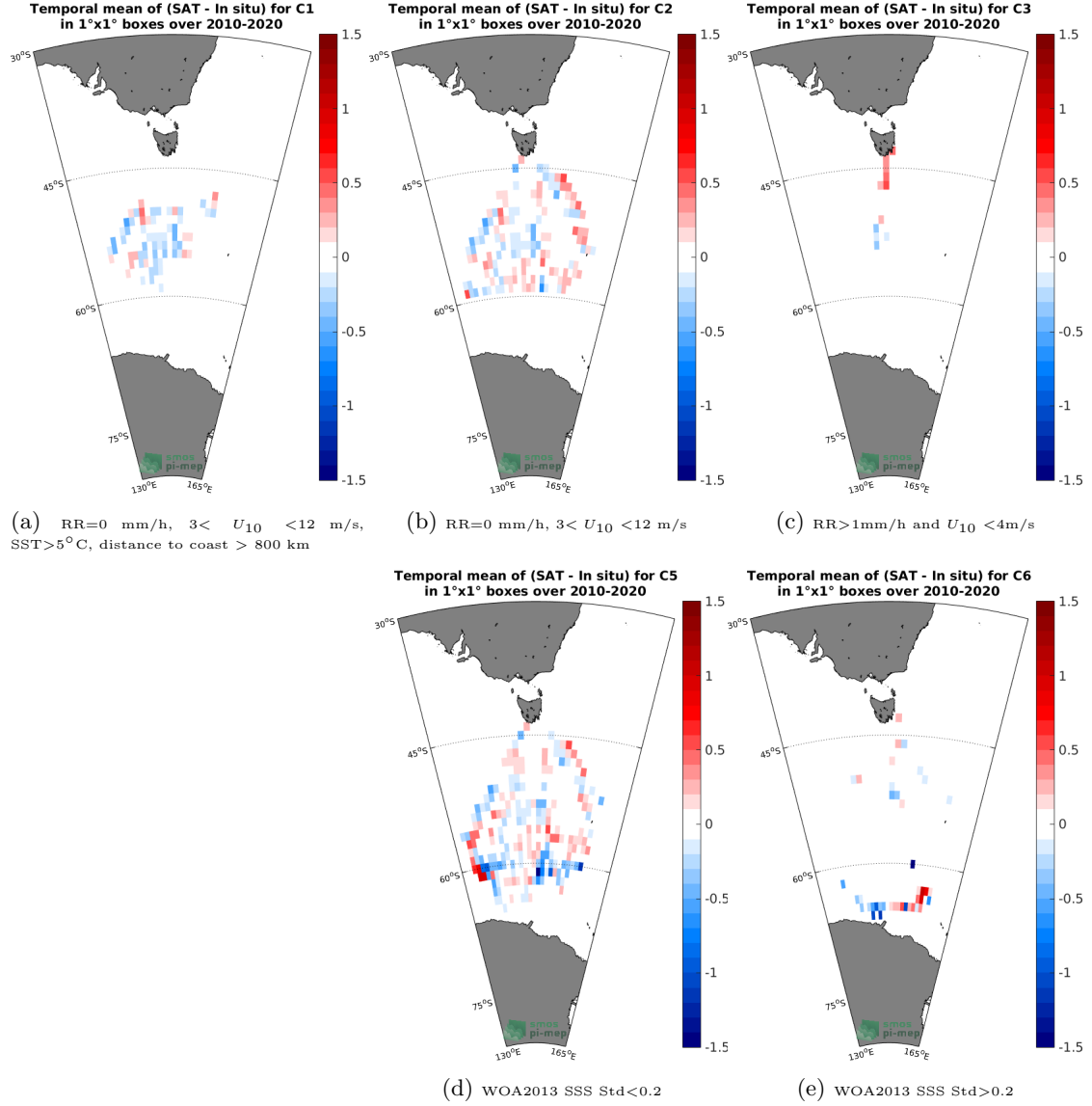
Figure 12: Temporal mean gridded over spatial boxes of size 1^\circ \times 1^\circ of \Delta\text{SSS} (SMOS SSS L3 v7 - 9 Days (CATDS-CECOS-LOCEAN) - TSG (LEGOS-Survostral)) for 5 different subdatasets corresponding to: RR=0 mm/h, 3 < U_{10} < 12 m/s, SST > 5^\circ\text{C} , distance to coast > 800 km (a), RR=0 mm/h, 3 < U_{10} < 12 m/s (b), RR > 1 mm/h and U_{10} < 4 m/s (c), WOA2013 SSS Std < 0.2 (d), WOA2013 SSS Std > 0.2 (e).
