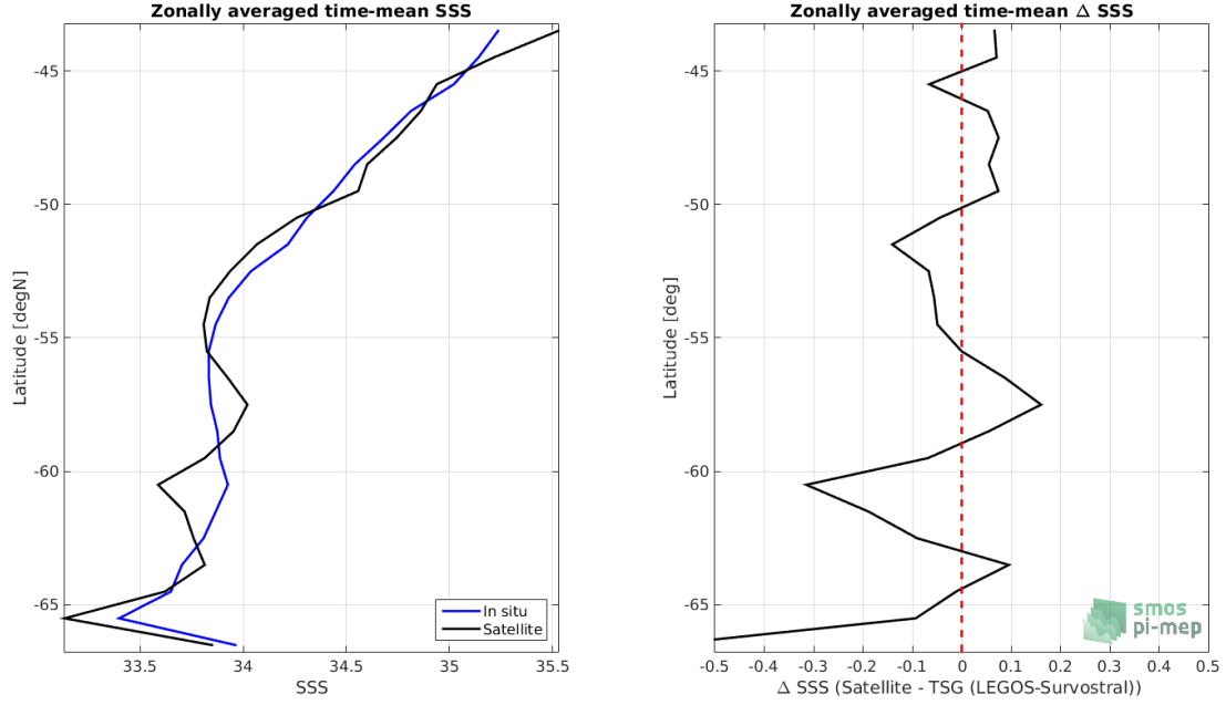
Figure 8: Left panel: Zonal mean SSS from SMOS SSS L3 v7 - 9 Days (CATDS-CECOS-LOCEAN) satellite product (black) and from TSG (LEGOS-Survostral) (blue). Right panel: Zonal mean of \Delta SSS (Satellite - TSG (LEGOS-Survostral)) for all the collected Pi-MEP match-up pairs estimated over the full satellite product period.
