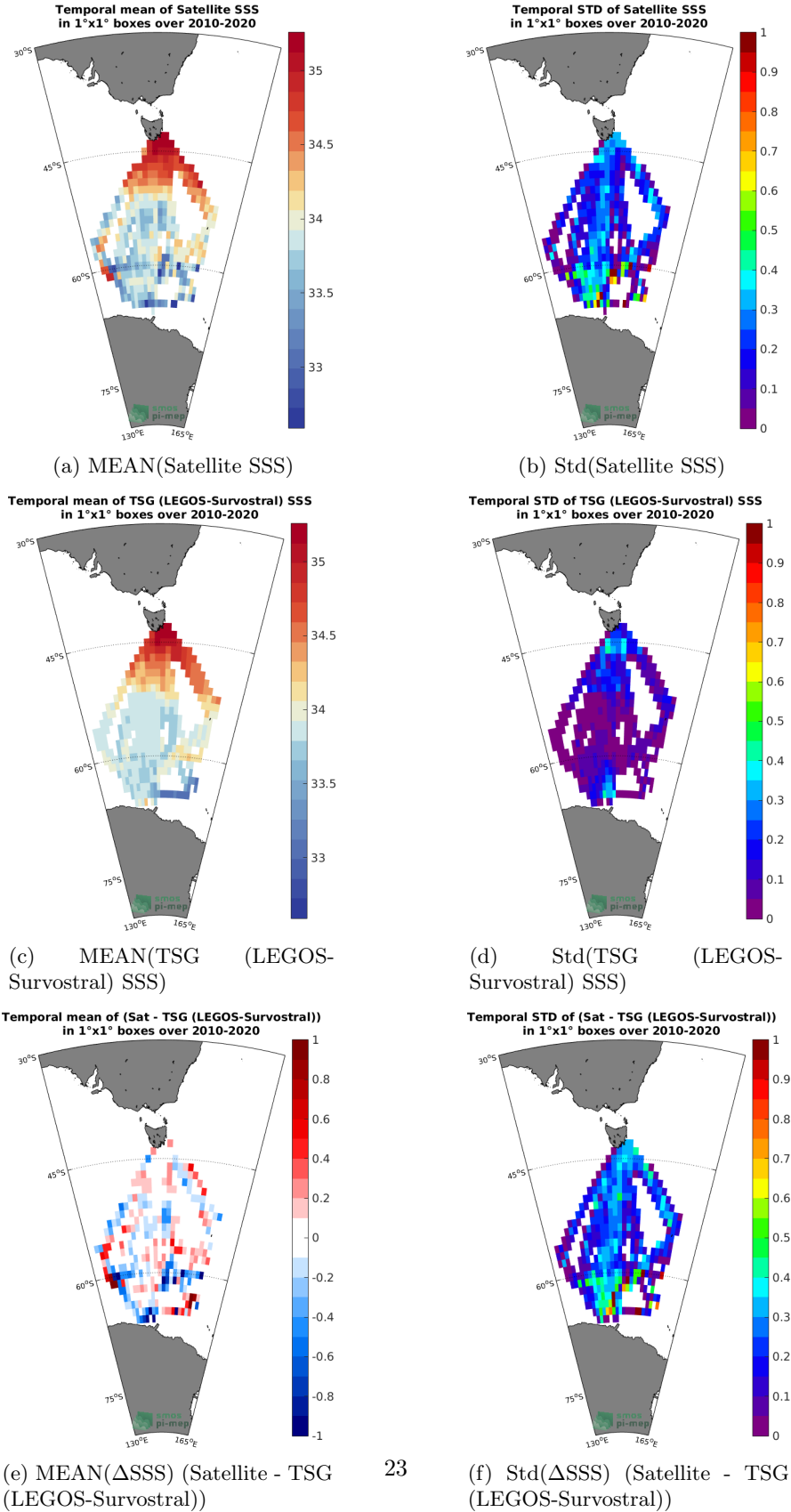
Figure 6: Temporal mean (left) and Std (right) of SSS from SMOS SSS L3 v7 - 9 Days (CATDS-CECOS-LOCEAN) (top), TSG (LEGOS-Survostral) (middle), and of \Delta SSS (Satellite - TSG (LEGOS-Survostral)). Only match-up pairs are used to generate these maps.
