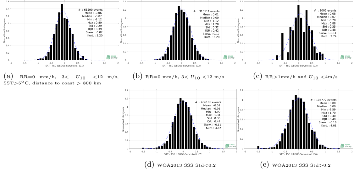
Figure 13: Normalized histogram of \Delta\text{SSS} (SMOS SSS L3 v7 - 9 Days (CATDS-CECOS-LOCEAN) - TSG (LEGOS-Survostral)) for 5 different subdatasets corresponding to: RR=0 mm/h, 3 < U_{10} < 12 m/s, SST > 5^\circ\text{C} , distance to coast > 800 km (a), RR=0 mm/h, 3 < U_{10} < 12 m/s (b), RR > 1\text{mm/h} and U_{10} < 4\text{m/s} (c), WOA2013 SSS Std <0.2 (d), WOA2013 SSS Std >0.2 (e).
