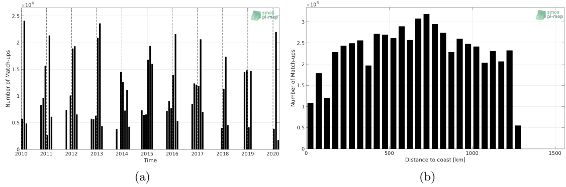
Figure 1: Number of match-ups between TSG (LEGOS-Survostral) and SMOS SSS L3 v7 - 9 Days (CATDS-CECOS-LOCEAN) SSS as a function of time (a) and as function of the distance to coast (b) over the Global Ocean Pi-MEP region and for the full satellite product period.
