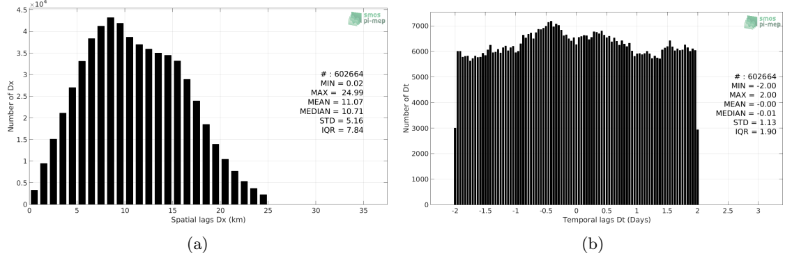
Figure 5: Histograms of the spatial (a) and temporal (b) lags between the location/time of the TSG (LEGOS-Survostral) measurement and the date of the corresponding SMOS SSS L3 v7 - 9 Days (CATDS-CECOS-LOCEAN) SSS pixel.
