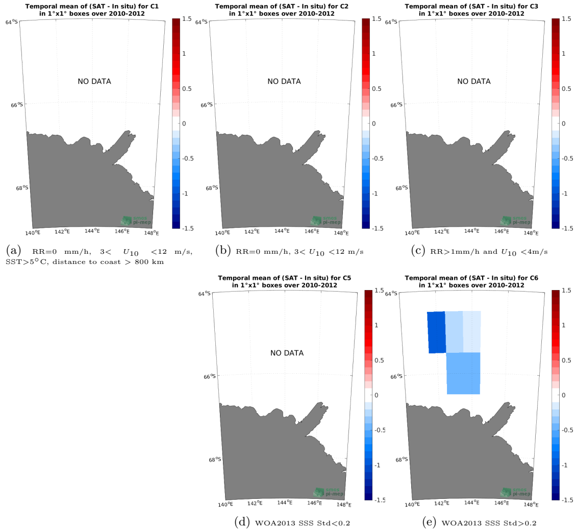
Figure 12: Temporal mean gridded over spatial boxes of size 1^\circ \times 1^\circ of \Delta SSS (SMOS SSS L3 v7 - 9 Days (CATDS-CECOS-LOCEAN) - TSG (LEGOS-Surv-Adel)) for 5 different subdatasets corresponding to: RR=0 mm/h, 3 < U_{10} < 12 m/s, SST>5°C, distance to coast > 800 km (a), RR=0 mm/h, 3 < U_{10} < 12 m/s (b), RR>1mm/h and U_{10} < 4 m/s (c), WOA2013 SSS Std<0.2 (d), WOA2013 SSS Std>0.2 (e).
