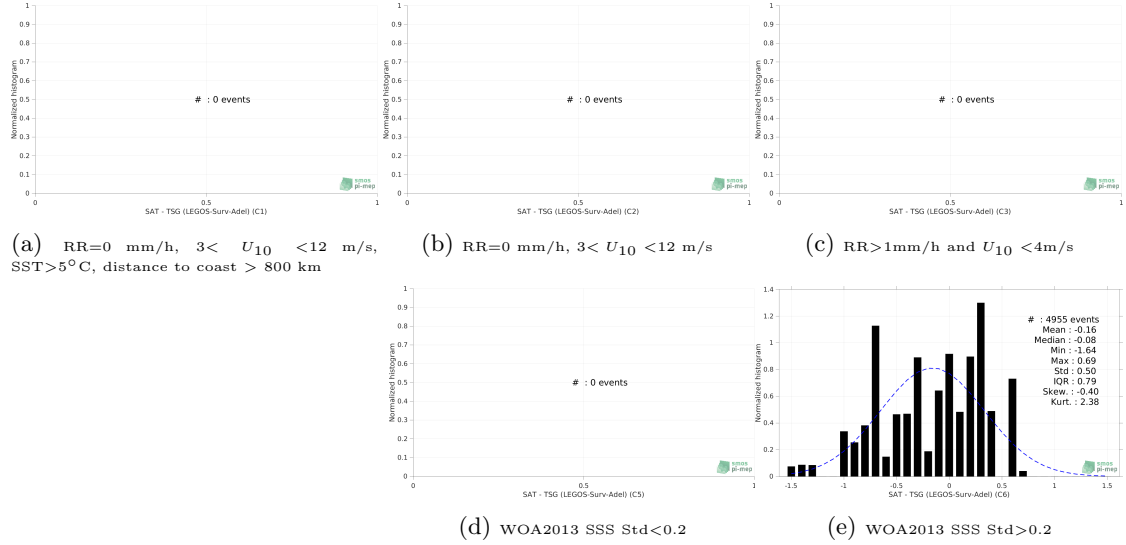
Figure 13: Normalized histogram of \Delta SSS (SMOS SSS L3 v7 - 9 Days (CATDS-CECOS-LOCEAN) - TSG (LEGOS-Surv-Adel)) for 5 different subdatasets corresponding to: RR=0 mm/h, 3 < U_{10} < 12 m/s, SST > 5°C, distance to coast > 800 km (a), RR=0 mm/h, 3 < U_{10} < 12 m/s (b), RR > 1mm/h and U_{10} < 4 m/s (c), WOA2013 SSS Std < 0.2 (d), WOA2013 SSS Std > 0.2 (e).
