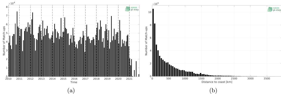
Figure 1: Number of match-ups between TSG (LEGOS-DM) and SMOS SSS L3 v7 - 9 Days (CATDS-CECOS-LOCEAN) SSS as a function of time (a) and as function of the distance to coast (b) over the Global Ocean Pi-MEP region and for the full satellite product period.
