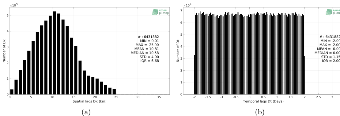
Figure 5: Histograms of the spatial (a) and temporal (b) lags between the location/time of the TSG (LEGOS-DM) measurement and the date of the corresponding SMOS SSS L3 v7 - 9 Days (CATDS-CECOS-LOCEAN) SSS pixel.
