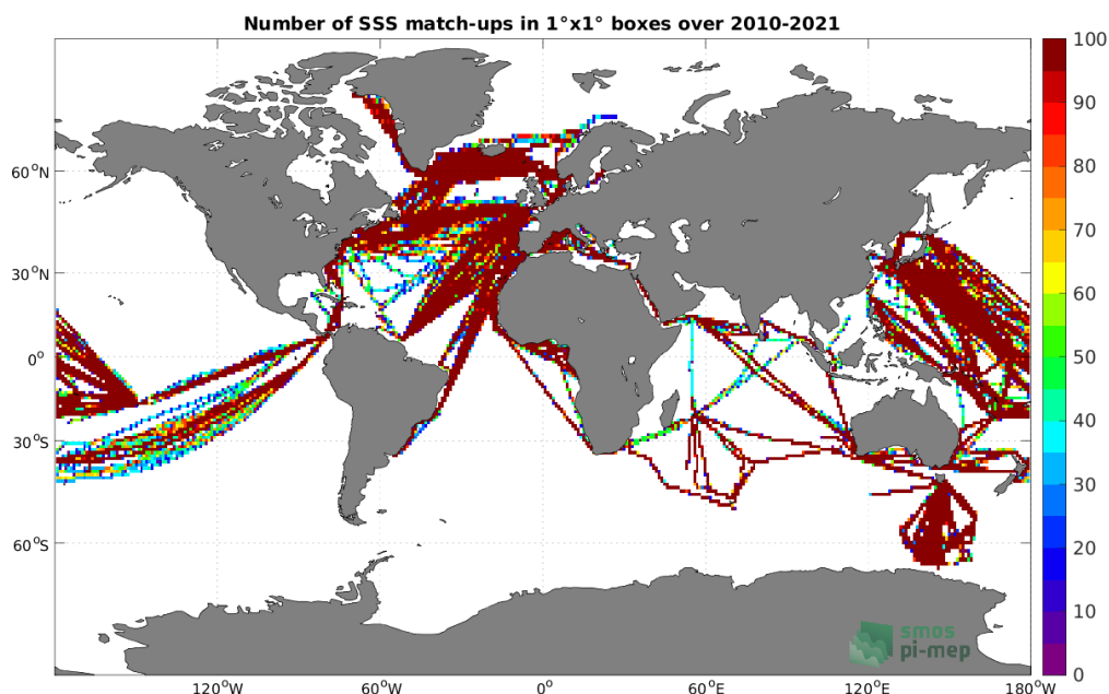
Figure 4: Number of SSS match-ups between TSG (LEGOS-DM) SSS and the SMOS SSS L3 v7 - 9 Days (CATDS-CECOS-LOCEAN) SSS product for the Global Ocean Pi-MEP region over 1^\circ \times 1^\circ boxes and for the full satellite product period.
