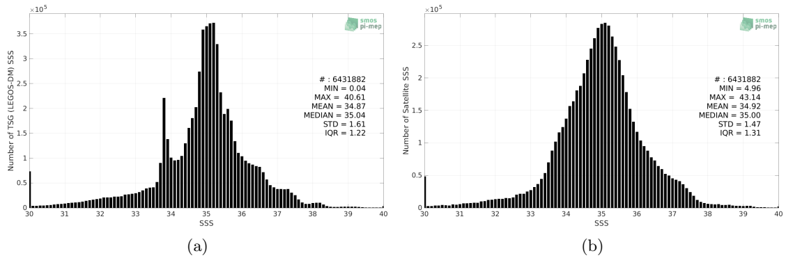
Figure 2: Histograms of SSS from TSG (LEGOS-DM) (a) and SMOS SSS L3 v7 - 9 Days (CATDS-CECOS-LOCEAN) (b) considering all match-up pairs per bins of 0.1 over the Global Ocean Pi-MEP region and for the full satellite product period.
