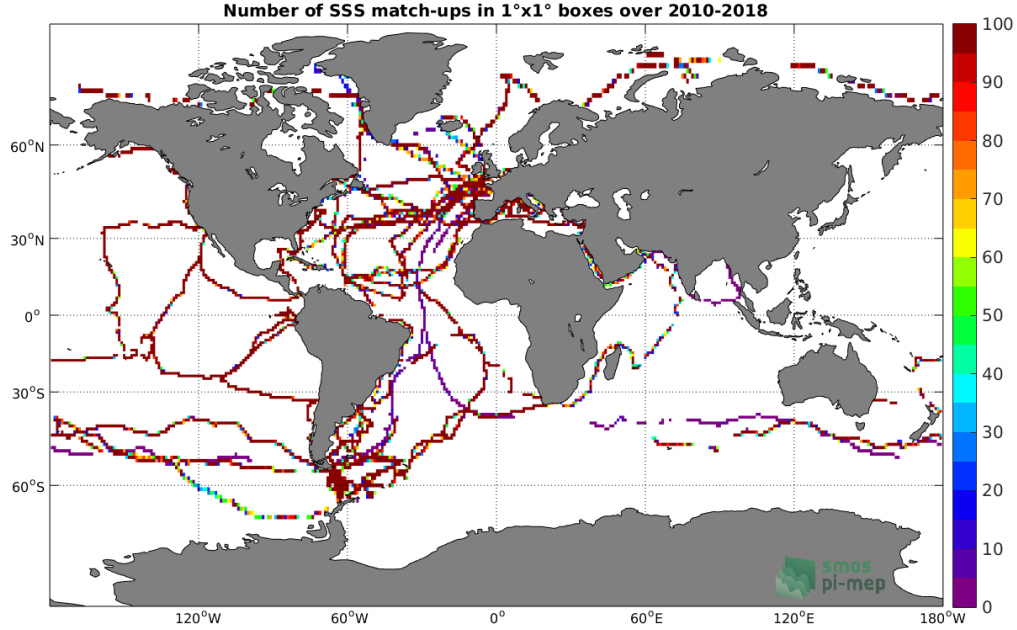
Figure 4: Number of SSS match-ups between TSG (GOSUD-Sailing-ship) SSS and the SMOS SSS L3 v7 - 9 Days (CATDS-CECOS-LOCEAN) SSS product for the Global Ocean Pi-MEP region over 1^\circ \times 1^\circ boxes and for the full satellite product period.
