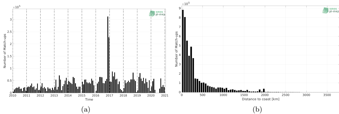
Figure 1: Number of match-ups between TSG (GOSUD-Research-vessel) and SMOS SSS L3 v7 - 9 Days (CATDS-CECOS-LOCEAN) SSS as a function of time (a) and as function of the distance to coast (b) over the Global Ocean Pi-MEP region and for the full satellite product period.
