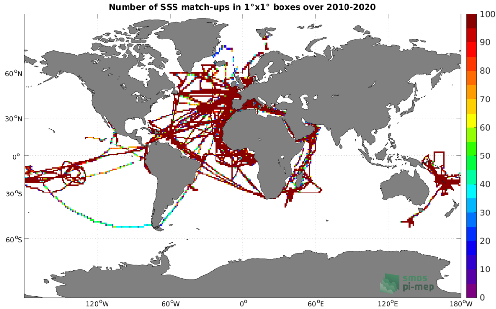
Figure 4: Number of SSS match-ups between TSG (GOSUD-Research-vessel) SSS and the SMOS SSS L3 v7 - 9 Days (CATDS-CECOS-LOCEAN) SSS product for the Global Ocean Pi-MEP region over 1^\circ \times 1^\circ boxes and for the full satellite product period.
