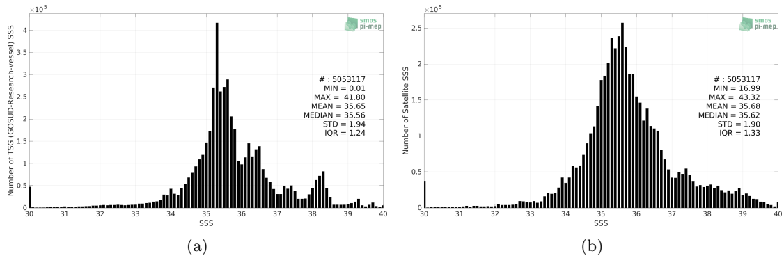
Figure 2: Histograms of SSS from TSG (GOSUD-Research-vessel) (a) and SMOS SSS L3 v7 - 9 Days (CATDS-CECOS-LOCEAN) (b) considering all match-up pairs per bins of 0.1 over the Global Ocean Pi-MEP region and for the full satellite product period.
