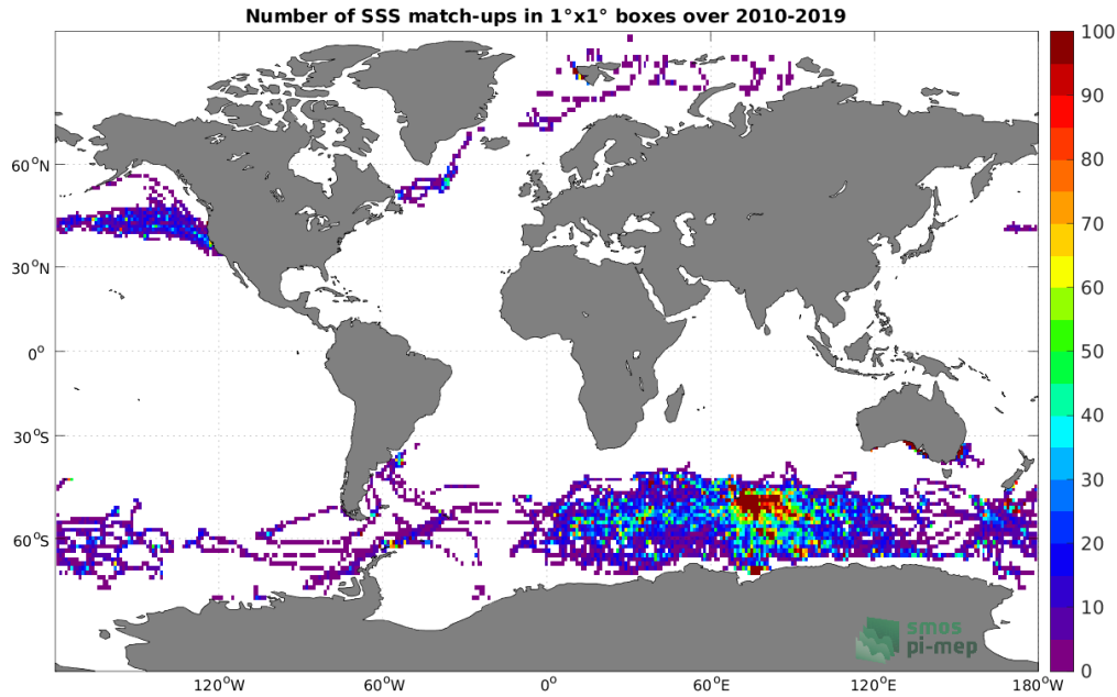
Figure 4: Number of SSS match-ups between Marine mammals SSS and the SMOS SSS L3 v7 - 9 Days (CATDS-CECOS-LOCEAN) SSS product for the Global Ocean Pi-MEP region over 1^\circ \times 1^\circ boxes and for the full satellite product period.
