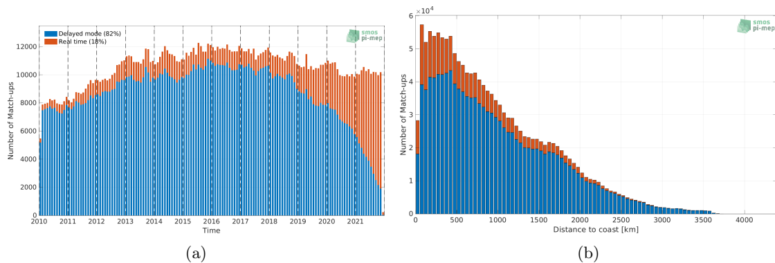
Figure 1: Number of match-ups between Argo and SMOS SSS L3 v7 - 9 Days (CATDS-CECOS-LOCEAN) SSS as a function of time (a) and as function of the distance to coast (b) over the Global Ocean Pi-MEP region and for the full satellite product period.
