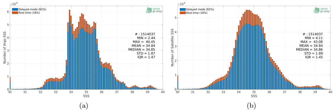
Figure 2: Histograms of SSS from Argo (a) and SMOS SSS L3 v7 - 9 Days (CATDS-CECOS-LOCEAN) (b) considering all match-up pairs per bins of 0.1 over the Global Ocean Pi-MEP region and for the full satellite product period.
