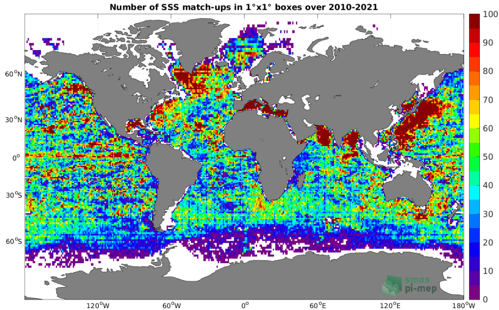
Figure 4: Number of SSS match-ups between Argo SSS and the SMOS SSS L3 v7 - 9 Days (CATDS-CECOS-LOCEAN) SSS product for the Global Ocean Pi-MEP region over 1^\circ \times 1^\circ boxes and for the full satellite product period.
