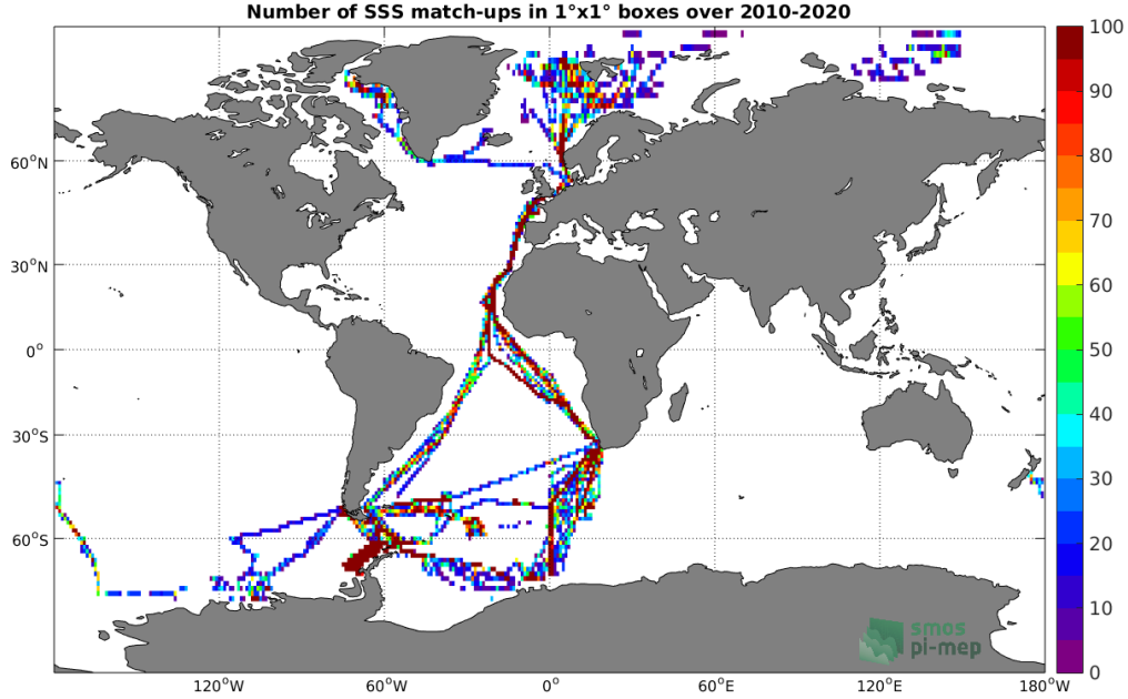
Figure 4: Number of SSS match-ups between TSG (Polarstern) SSS and the SMOS SSS L3 v7 - 18 Days (CATDS-CECOS-LOCEAN) SSS product for the Global Ocean Pi-MEP region over 1^\circ \times 1^\circ boxes and for the full satellite product period.
