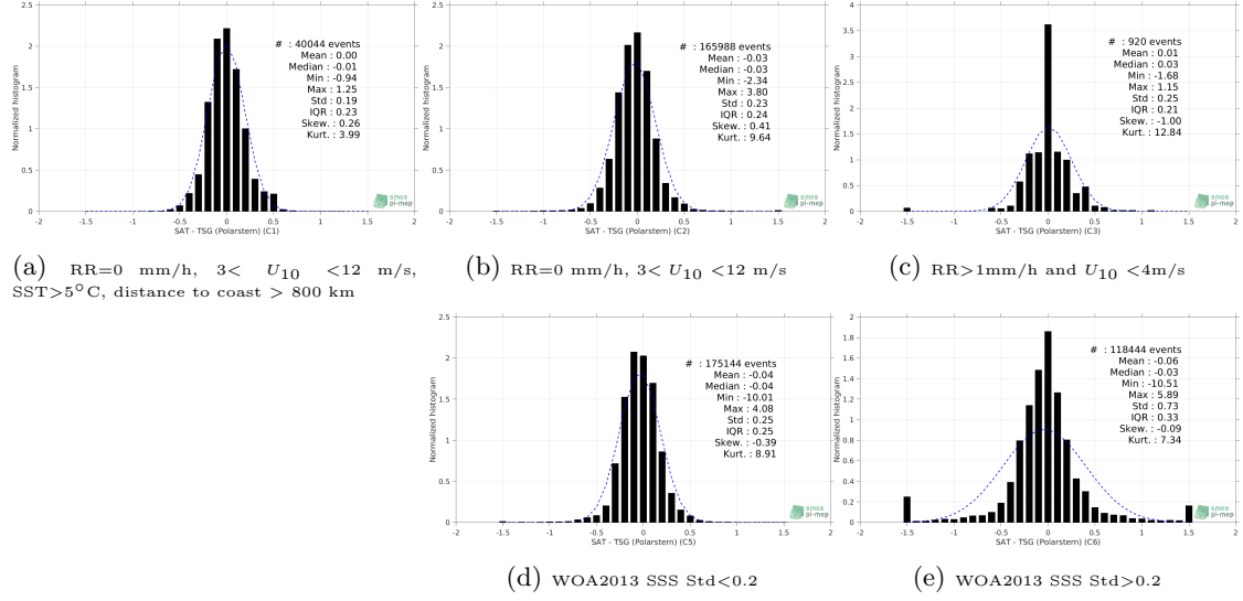
Figure 13: Normalized histogram of \Delta SSS (SMOS SSS L3 v7 - 18 Days (CATDS-CECOS-LOCEAN) - TSG (Polarstern)) for 5 different subdatasets corresponding to: RR=0 mm/h, 3 < U_{10} < 12 m/s, SST>5°C, distance to coast > 800 km (a), RR=0 mm/h, 3 < U_{10} < 12 m/s (b), RR>1mm/h and U_{10} < 4 m/s (c), WOA2013 SSS Std<0.2 (d), WOA2013 SSS Std>0.2 (e).
