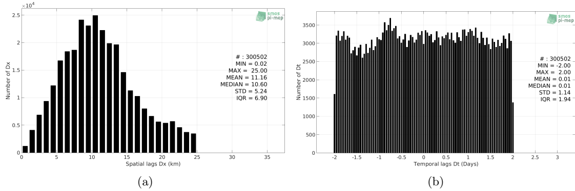
Figure 5: Histograms of the spatial (a) and temporal (b) lags between the location/time of the TSG (Polarstern) measurement and the date of the corresponding SMOS SSS L3 v7 - 18 Days (CATDS-CECOS-LOCEAN) SSS pixel.
