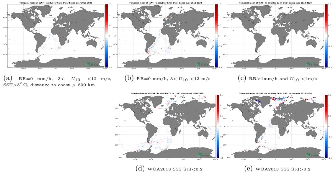
Figure 12: Temporal mean gridded over spatial boxes of size 1^\circ \times 1^\circ of \Delta SSS (SMOS SSS L3 v7 - 18 Days (CATDS-CECOS-LOCEAN) - TSG (Polarstern)) for 5 different subdatasets corresponding to:RR=0 mm/h, 3 < U_{10} < 12 m/s, SST >5^\circ\text{C} , distance to coast > 800 km (a), RR=0 mm/h, 3 < U_{10} < 12 m/s (b), RR >1 mm/h and U_{10} < 4 m/s (c), WOA2013 SSS Std <0.2 (d), WOA2013 SSS Std >0.2 (e).
