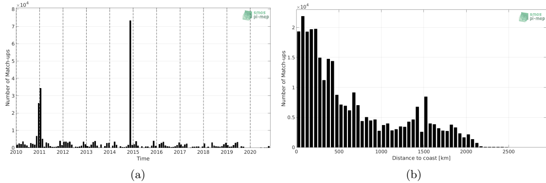
Figure 1: Number of match-ups between TSG (Polarstern) and SMOS SSS L3 v7 - 18 Days (CATDS-CECOS-LOCEAN) SSS as a function of time (a) and as function of the distance to coast (b) over the Global Ocean Pi-MEP region and for the full satellite product period.
