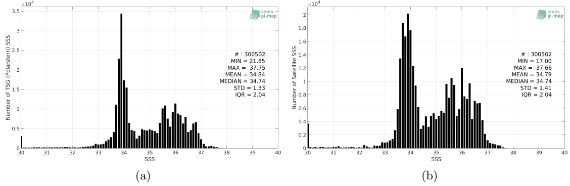
Figure 2: Histograms of SSS from TSG (Polarstern) (a) and SMOS SSS L3 v7 - 18 Days (CATDS-CECOS-LOCEAN) (b) considering all match-up pairs per bins of 0.1 over the Global Ocean Pi-MEP region and for the full satellite product period.
