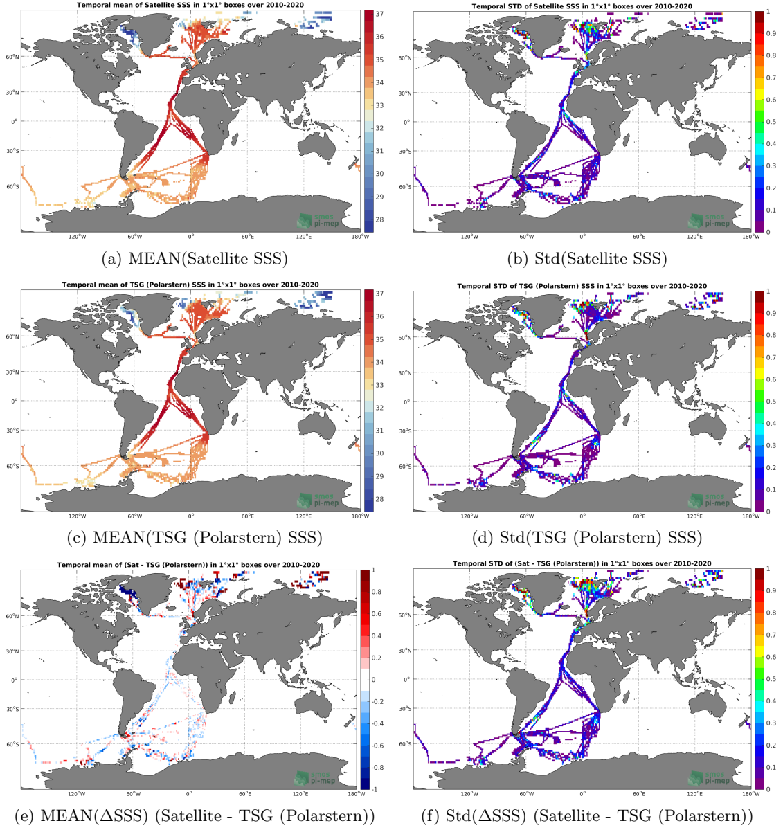
Figure 6: Temporal mean (left) and Std (right) of SSS from SMOS SSS L3 v7 - 18 Days (CATDS-CECOS-LOCEAN) (top), TSG (Polarstern) (middle), and of \Delta SSS (Satellite - TSG (Polarstern)). Only match-up pairs are used to generate these maps.
