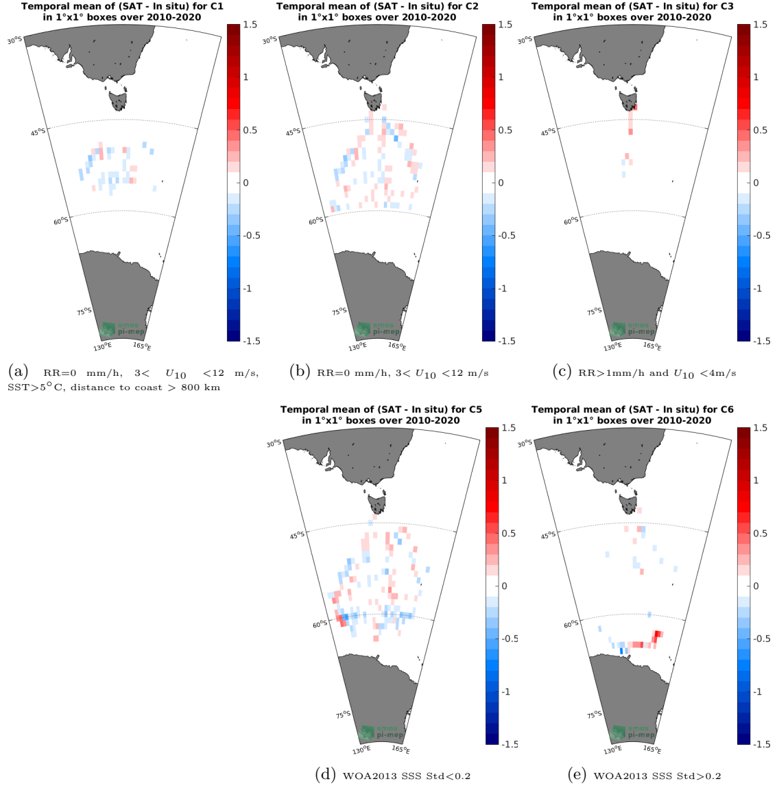
Figure 12: Temporal mean gridded over spatial boxes of size 1^\circ \times 1^\circ of \Delta\text{SSS} (SMOS SSS L3 v7 - 18 Days (CATDS-CECOS-LOCEAN) - TSG (LEGOS-Survostral)) for 5 different subdatasets corresponding to: RR=0 mm/h, 3 < U_{10} < 12 m/s, SST > 5^\circ\text{C} , distance to coast > 800 km (a), RR=0 mm/h, 3 < U_{10} < 12 m/s (b), RR > 1 mm/h and U_{10} < 4 m/s (c), WOA2013 SSS Std < 0.2 (d), WOA2013 SSS Std > 0.2 (e).
