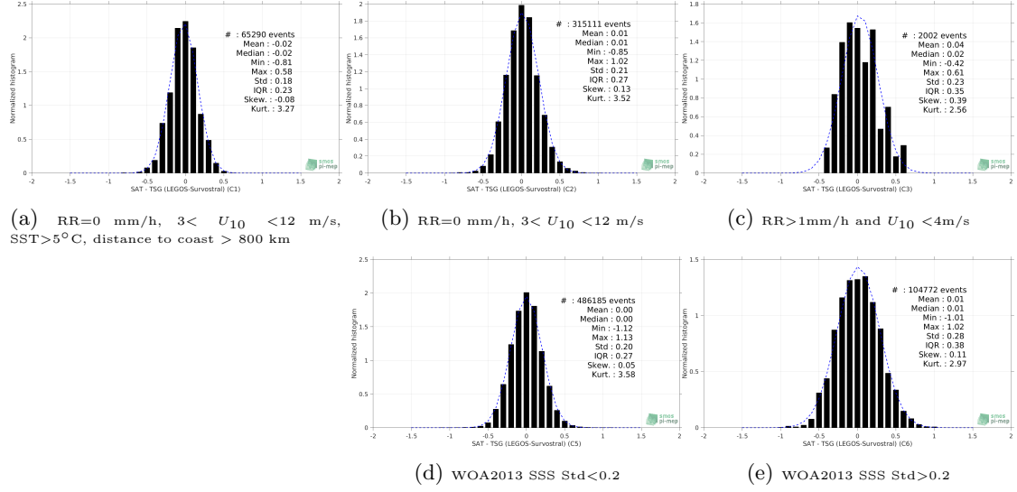
Figure 13: Normalized histogram of \Delta SSS (SMOS SSS L3 v7 - 18 Days (CATDS-CECOS-LOCEAN) - TSG (LEGOS-Survostral)) for 5 different subdatasets corresponding to: RR=0 mm/h, 3 < U_{10} < 12 m/s, SST>5°C, distance to coast > 800 km (a), RR=0 mm/h, 3 < U_{10} < 12 m/s (b), RR>1mm/h and U_{10} < 4 m/s (c), WOA2013 SSS Std<0.2 (d), WOA2013 SSS Std>0.2 (e).
