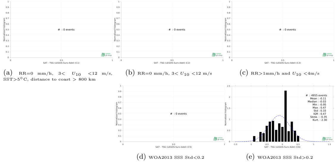
Figure 13: Normalized histogram of \Delta SSS (SMOS SSS L3 v7 - 18 Days (CATDS-CECOS-LOCEAN) - TSG (LEGOS-Surv-Adel)) for 5 different subdatasets corresponding to: RR=0 mm/h, 3 < U_{10} < 12 m/s, SST>5°C, distance to coast > 800 km (a), RR=0 mm/h, 3 < U_{10} < 12 m/s (b), RR>1mm/h and U_{10} < 4 m/s (c), WOA2013 SSS Std<0.2 (d), WOA2013 SSS Std>0.2 (e).
