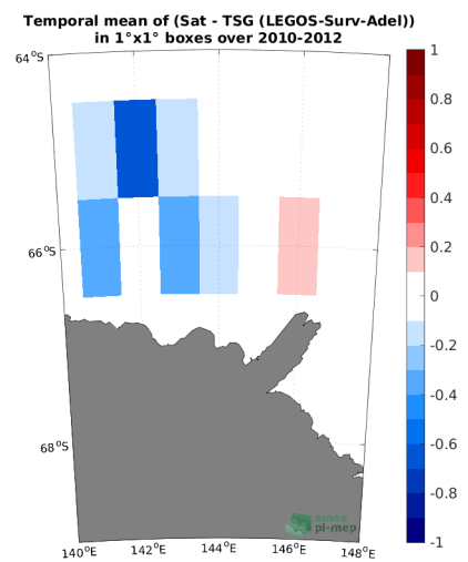
(e) MEAN( \Delta SSS) (Satellite - TSG (LEGOS-Surv-Adel))
