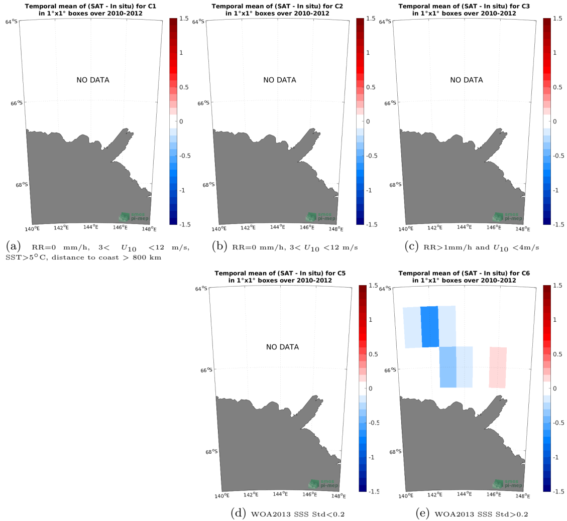
Figure 12: Temporal mean gridded over spatial boxes of size 1^\circ \times 1^\circ of \Delta SSS (SMOS SSS L3 v7 - 18 Days (CATDS-CECOS-LOCEAN) - TSG (LEGOS-Surv-Adel)) for 5 different subdatasets corresponding to: RR=0 mm/h, 3 < U_{10} < 12 m/s, SST>5°C, distance to coast > 800 km (a), RR=0 mm/h, 3 < U_{10} < 12 m/s (b), RR>1mm/h and U_{10} < 4 m/s (c), WOA2013 SSS Std<0.2 (d), WOA2013 SSS Std>0.2 (e).
