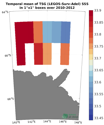
(c) MEAN(TSG (LEGOS-Surv-Adel) SSS)
