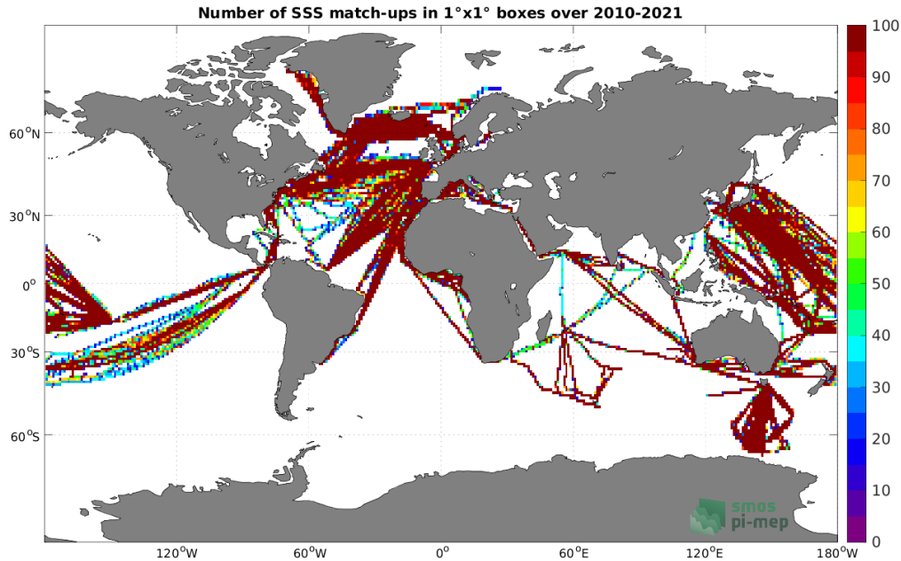
Figure 4: Number of SSS match-ups between TSG (LEGOS-DM) SSS and the SMOS SSS L3 v7 - 18 Days (CATDS-CECOS-LOCEAN) SSS product for the Global Ocean Pi-MEP region over 1^\circ \times 1^\circ boxes and for the full satellite product period.
