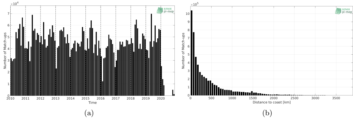
Figure 1: Number of match-ups between TSG (LEGOS-DM) and SMOS SSS L3 v7 - 18 Days (CATDS-CECOS-LOCEAN) SSS as a function of time (a) and as function of the distance to coast (b) over the Global Ocean Pi-MEP region and for the full satellite product period.
