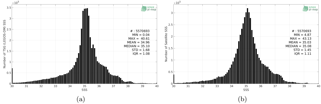
Figure 2: Histograms of SSS from TSG (LEGOS-DM) (a) and SMOS SSS L3 v7 - 18 Days (CATDS-CECOS-LOCEAN) (b) considering all match-up pairs per bins of 0.1 over the Global Ocean Pi-MEP region and for the full satellite product period.
