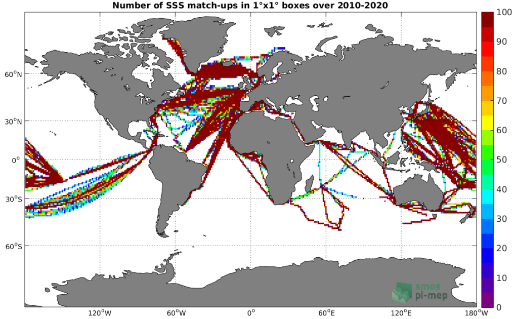
Figure 4: Number of SSS match-ups between TSG (LEGOS-DM) SSS and the SMOS SSS L3 v7 - 18 Days (CATDS-CECOS-LOCEAN) SSS product for the Global Ocean Pi-MEP region over 1^\circ \times 1^\circ boxes and for the full satellite product period.
