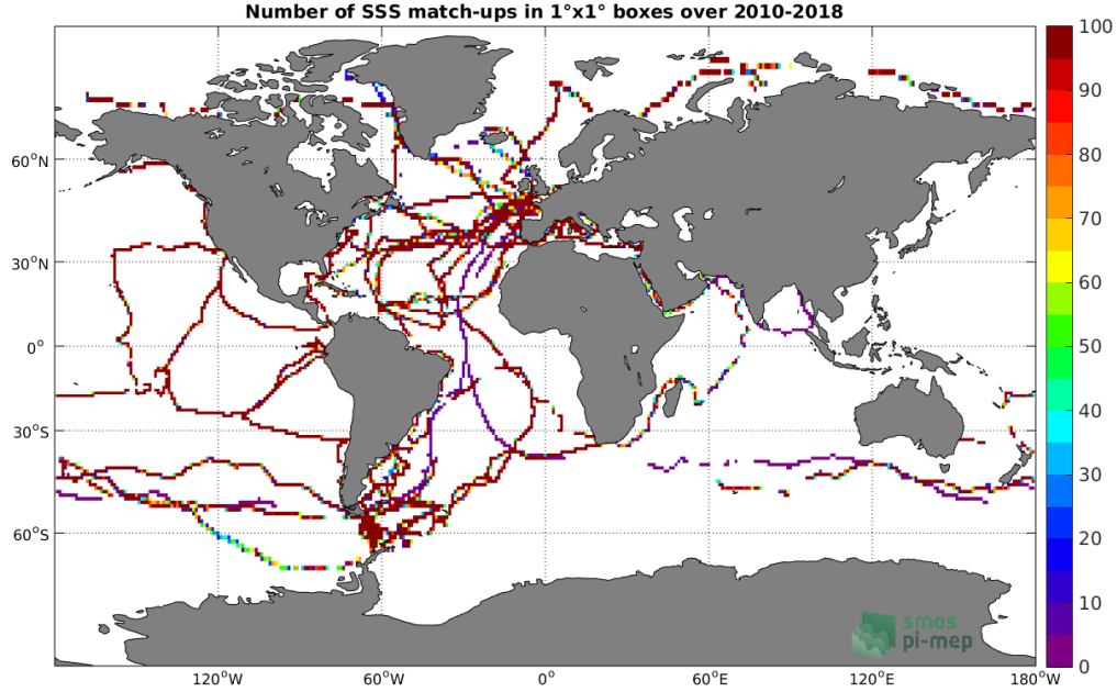
Figure 4: Number of SSS match-ups between TSG (GOSUD-Sailing-ship) SSS and the SMOS SSS L3 v7 - 18 Days (CATDS-CECOS-LOCEAN) SSS product for the Global Ocean Pi-MEP region over 1^\circ \times 1^\circ boxes and for the full satellite product period.
