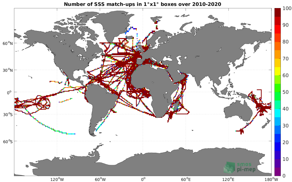
Figure 4: Number of SSS match-ups between TSG (GOSUD-Research-vessel) SSS and the SMOS SSS L3 v7 - 18 Days (CATDS-CECOS-LOCEAN) SSS product for the Global Ocean Pi-MEP region over 1^\circ \times 1^\circ boxes and for the full satellite product period.
