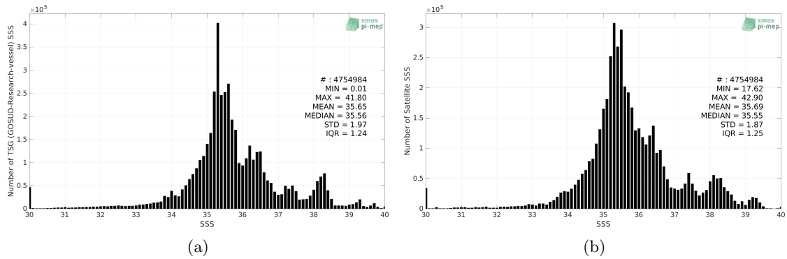
Figure 2: Histograms of SSS from TSG (GOSUD-Research-vessel) (a) and SMOS SSS L3 v7 - 18 Days (CATDS-CECOS-LOCEAN) (b) considering all match-up pairs per bins of 0.1 over the Global Ocean Pi-MEP region and for the full satellite product period.
