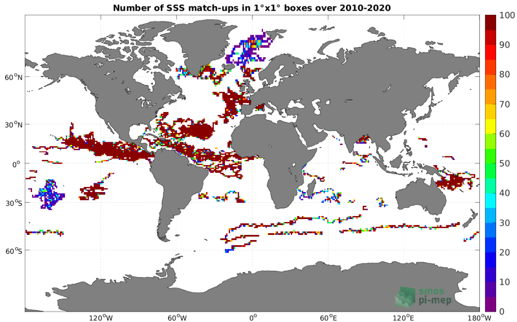
Figure 3: Number of SSS match-ups between Surface drifters SSS and the SMOS SSS L3 v7 - 18 Days (CATDS-CECOS-LOCEAN) SSS product for the Global Ocean Pi-MEP region over 1^\circ \times 1^\circ boxes and for the full satellite product period.
