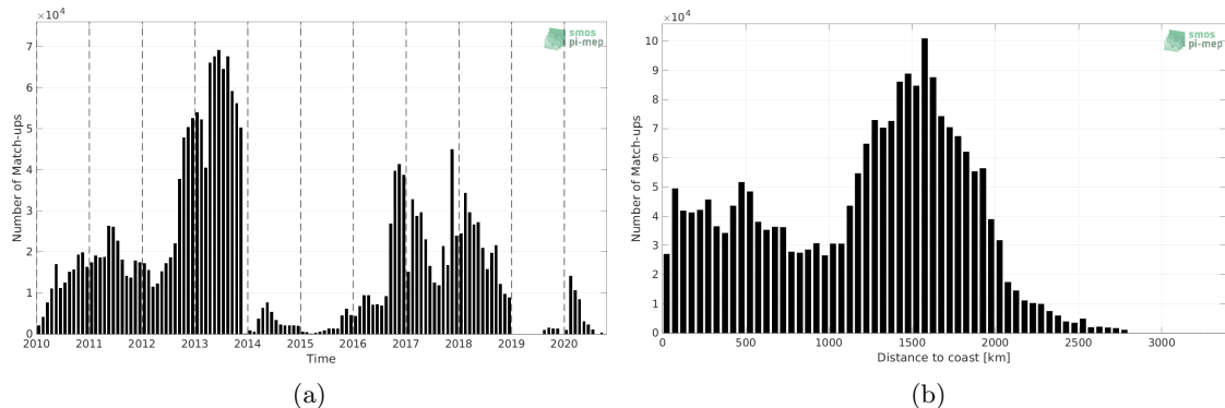
Figure 1: Number of match-ups between Surface drifters and SMOS SSS L3 v7 - 18 Days (CATDS-CECOS-LOCEAN) SSS as a function of time (a) and as function of the distance to coast (b) over the Global Ocean Pi-MEP region and for the full satellite product period.
