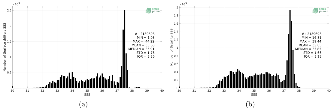
Figure 2: Histograms of SSS from Surface drifters (a) and SMOS SSS L3 v7 - 18 Days (CATDS-CECOS-LOCEAN) (b) considering all match-up pairs per bins of 0.1 over the Global Ocean Pi-MEP region and for the full satellite product period.
