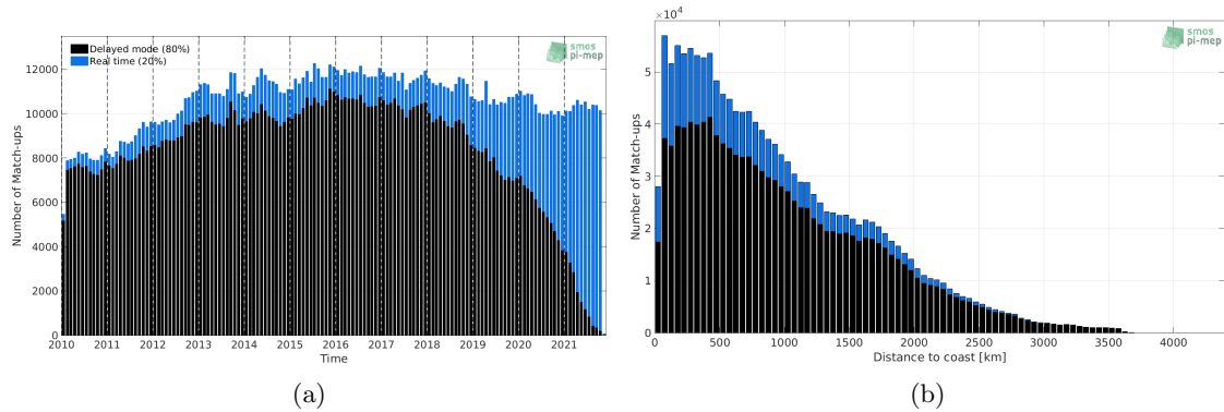
Figure 1: Number of match-ups between Argo and SMOS SSS L3 v7 - 18 Days (CATDS-CECOS-LOCEAN) SSS as a function of time (a) and as function of the distance to coast (b) over the Global Ocean Pi-MEP region and for the full satellite product period.
