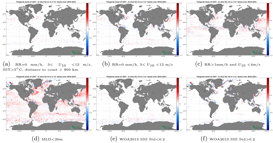
Figure 12: Temporal mean gridded over spatial boxes of size 1^\circ \times 1^\circ of \Delta SSS (SMOS SSS L3 v7 - 18 Days (CATDS-CECOS-LOCEAN) - Argo) for 6 different subdatasets corresponding to: RR=0 mm/h, 3 < U_{10} < 12 m/s, SST >5^\circ C, distance to coast > 800 km (a), RR=0 mm/h, 3 < U_{10} < 12 m/s (b), RR >1 mm/h and U_{10} < 4 m/s (c),MLD <20 m (d),WOA2013 SSS Std <0.2 (e),WOA2013 SSS Std >0.2 (f).
