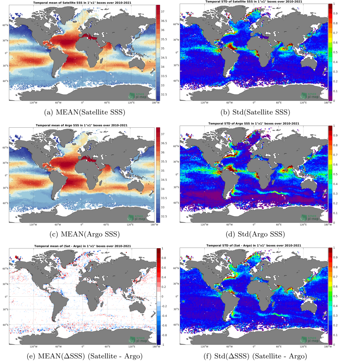
Figure 6: Temporal mean (left) and Std (right) of SSS from SMOS SSS L3 v7 - 18 Days (CATDS-CECOS-LOCEAN) (top), Argo (middle), and of \Delta SSS (Satellite - Argo). Only match-up pairs are used to generate these maps.
