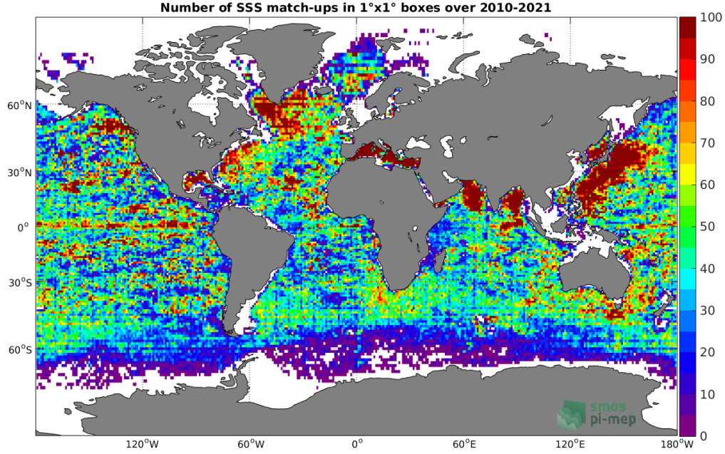
Figure 4: Number of SSS match-ups between Argo SSS and the SMOS SSS L3 v7 - 18 Days (CATDS-CECOS-LOCEAN) SSS product for the Global Ocean Pi-MEP region over 1^\circ \times 1^\circ boxes and for the full satellite product period.
