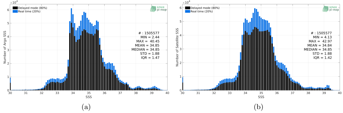
Figure 2: Histograms of SSS from Argo (a) and SMOS SSS L3 v7 - 18 Days (CATDS-CECOS-LOCEAN) (b) considering all match-up pairs per bins of 0.1 over the Global Ocean Pi-MEP region and for the full satellite product period.
