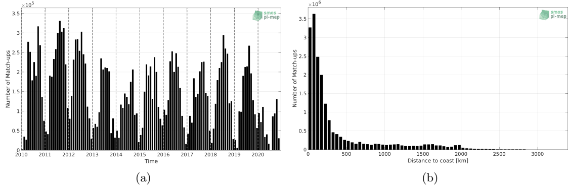
Figure 1: Number of match-ups between TSG (SAMOS) and SMOS SSS L3 v5 - 9 Days (CATDS-CECOS-LOCEAN) SSS as a function of time (a) and as function of the distance to coast (b) over the Global Ocean Pi-MEP region and for the full satellite product period.
