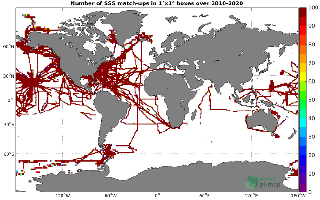
Figure 4: Number of SSS match-ups between TSG (SAMOS) SSS and the SMOS SSS L3 v5 - 9 Days (CATDS-CECOS-LOCEAN) SSS product for the Global Ocean Pi-MEP region over 1^\circ \times 1^\circ boxes and for the full satellite product period.
