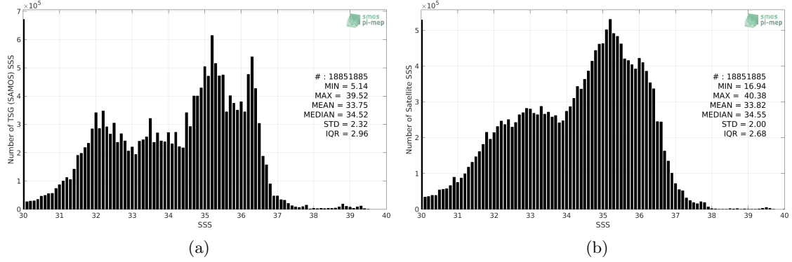
Figure 2: Histograms of SSS from TSG (SAMOS) (a) and SMOS SSS L3 v5 - 9 Days (CATDS-CECOS-LOCEAN) (b) considering all match-up pairs per bins of 0.1 over the Global Ocean Pi-MEP region and for the full satellite product period.
