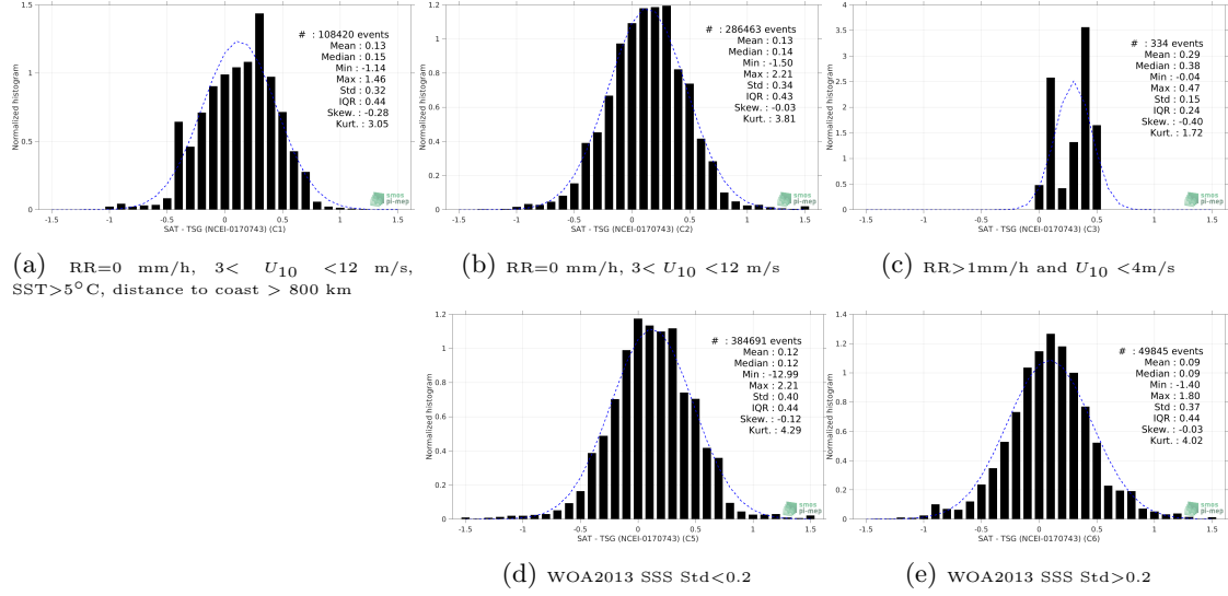
Figure 13: Normalized histogram of \Delta SSS (SMOS SSS L3 v5 - 9 Days (CATDS-CECOS-LOCEAN) - TSG (NCEI-0170743)) for 5 different subdatasets corresponding to: RR=0 mm/h, 3 < U_{10} < 12 m/s, SST>5°C, distance to coast > 800 km (a), RR=0 mm/h, 3 < U_{10} < 12 m/s (b), RR>1mm/h and U_{10} < 4 m/s (c), WOA2013 SSS Std<0.2 (d), WOA2013 SSS Std>0.2 (e).
