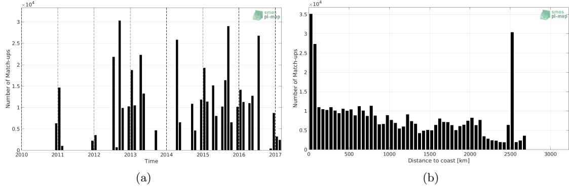
Figure 1: Number of match-ups between TSG (NCEI-0170743) and SMOS SSS L3 v5 - 9 Days (CATDS-CECOS-LOCEAN) SSS as a function of time (a) and as function of the distance to coast (b) over the Global Ocean Pi-MEP region and for the full satellite product period.
