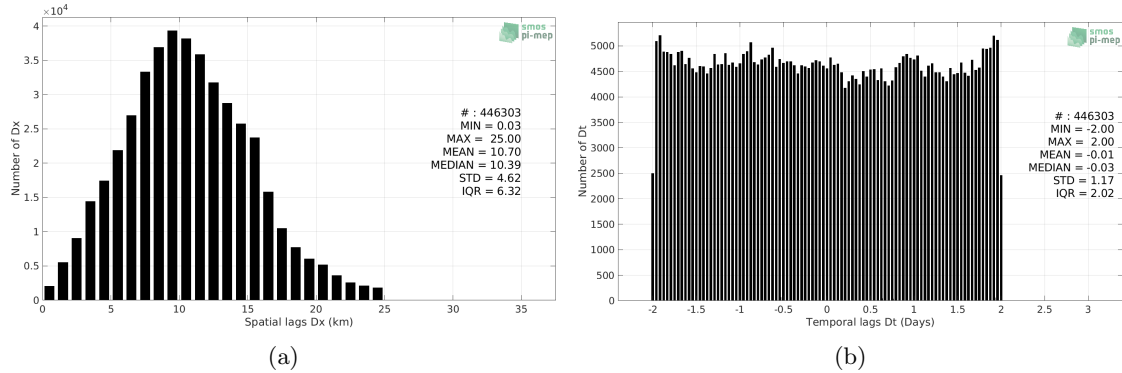
Figure 5: Histograms of the spatial (a) and temporal (b) lags between the location/time of the TSG (NCEI-0170743) measurement and the date of the corresponding SMOS SSS L3 v5 - 9 Days (CATDS-CECOS-LOCEAN) SSS pixel.
