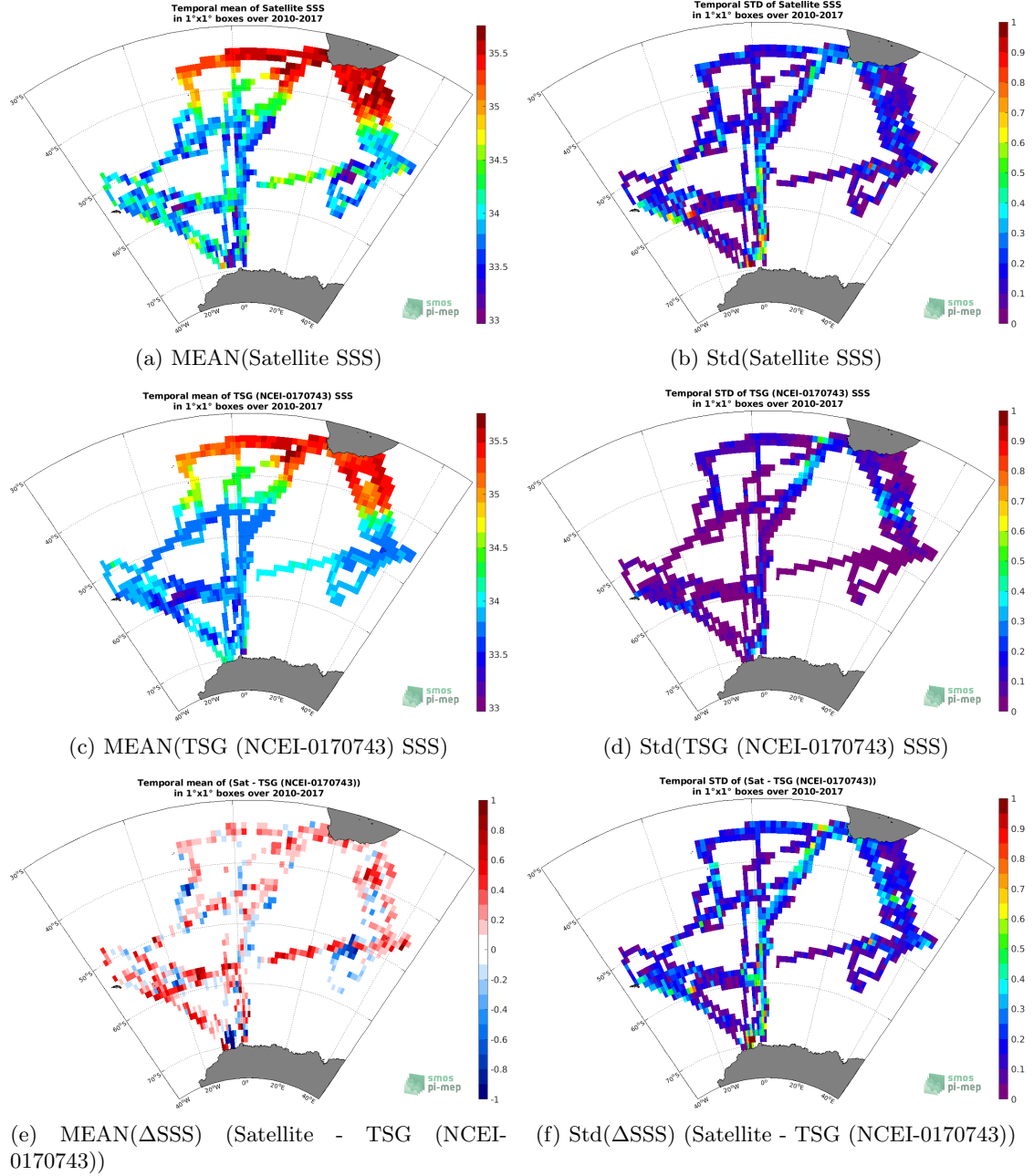
Figure 6: Temporal mean (left) and Std (right) of SSS from SMOS SSS L3 v5 - 9 Days (CATDS-CECOS-LOCEAN) (top), TSG (NCEI-0170743) (middle), and of \Delta SSS (Satellite - TSG (NCEI-0170743)). Only match-up pairs are used to generate these maps.
