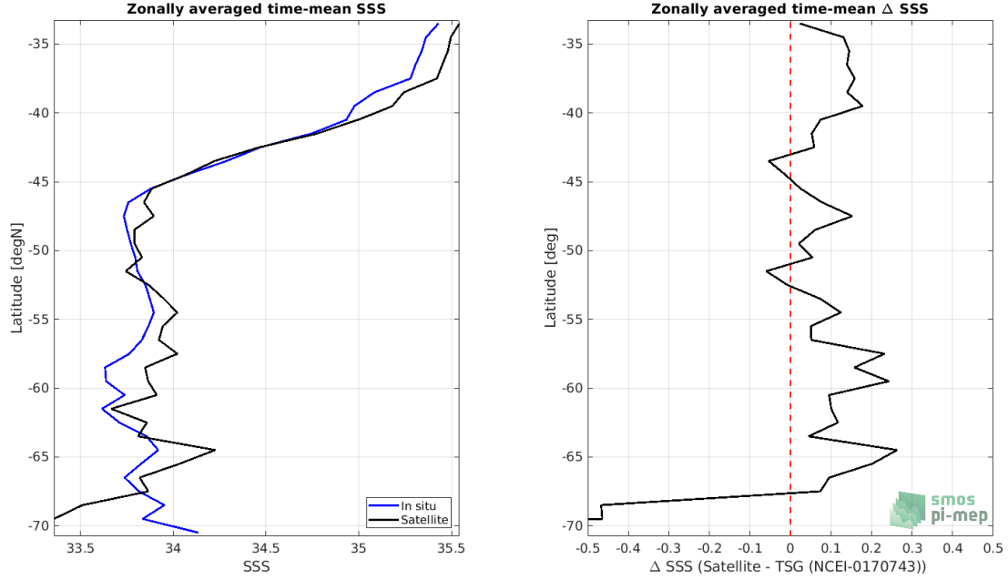
Figure 8: Left panel: Zonal mean SSS from SMOS SSS L3 v5 - 9 Days (CATDS-CECOS-LOCEAN) satellite product (black) and from TSG (NCEI-0170743) (blue). Right panel: Zonal mean of \Delta SSS (Satellite - TSG (NCEI-0170743)) for all the collected Pi-MEP match-up pairs estimated over the full satellite product period.
