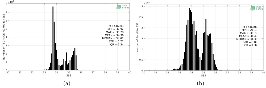
Figure 2: Histograms of SSS from TSG (NCEI-0170743) (a) and SMOS SSS L3 v5 - 9 Days (CATDS-CECOS-LOCEAN) (b) considering all match-up pairs per bins of 0.1 over the Global Ocean Pi-MEP region and for the full satellite product period.
