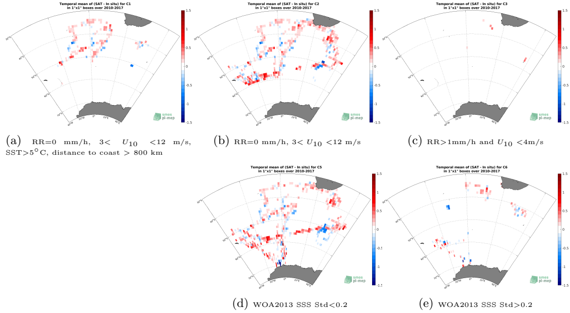
Figure 12: Temporal mean gridded over spatial boxes of size 1^{\circ}\times 1^{\circ} of \Delta\text{SSS} (SMOS SSS L3 v5 - 9 Days (CATDS-CECOS-LOCEAN) - TSG (NCEI-0170743)) for 5 different subdatasets corresponding to: \text{RR}=0 mm/h, 3 < U_{10} < 12 m/s, \text{SST} > 5^{\circ}\text{C} , distance to coast > 800 km (a), \text{RR}=0 mm/h, 3 < U_{10} < 12 m/s (b), \text{RR} > 1 mm/h and U_{10} < 4 m/s (c), WOA2013 SSS Std < 0.2 (d), WOA2013 SSS Std > 0.2 (e).
