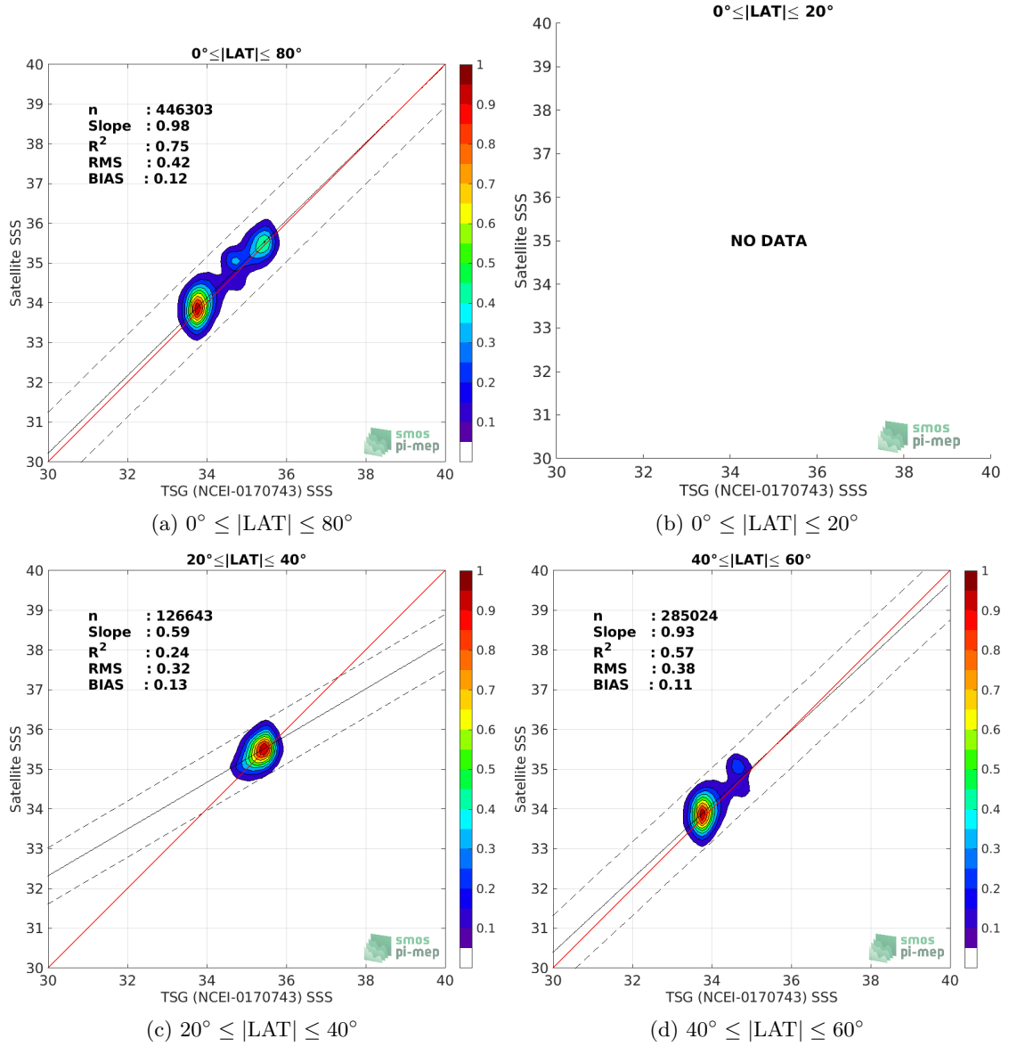
Figure 9: Contour maps of the concentration of SMOS SSS L3 v5 - 9 Days (CATDS-CECOS-LOCEAN) SSS (y-axis) versus TSG (NCEI-0170743) SSS (x-axis) at match-up pairs for different latitude bands. For each plot, the red line shows x=y . The black thin and dashed lines indicate a linear fit through the data cloud and the \pm 95\% confidence levels, respectively. The number match-up pairs n , the slope and R^2 coefficient of the linear fit, the root mean square (RMS) and the mean bias between satellite and in situ data are indicated for each latitude band in each plots.
