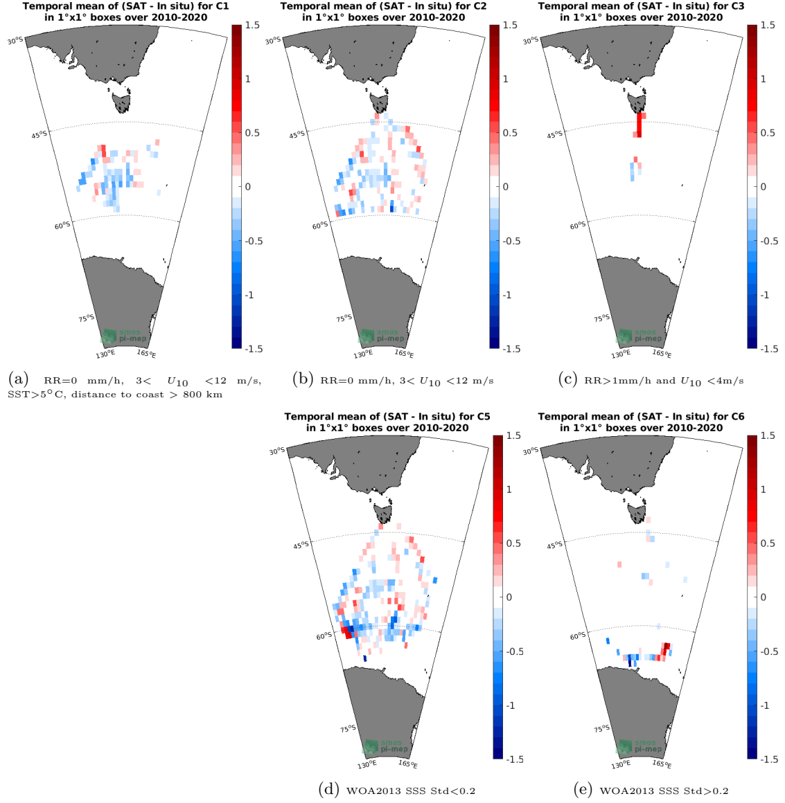
Figure 12: Temporal mean gridded over spatial boxes of size 1°x1° of \Delta\text{SSS} (SMOS SSS L3 v5 - 9 Days (CATDS-CECOS-LOCEAN) - TSG (LEGOS-Survostral)) for 5 different subdatasets corresponding to: RR=0 mm/h, 3 < U_{10} < 12 m/s, SST > 5^\circ\text{C} , distance to coast > 800 km (a), RR=0 mm/h, 3 < U_{10} < 12 m/s (b), RR > 1 mm/h and U_{10} < 4 m/s (c), WOA2013 SSS Std < 0.2 (d), WOA2013 SSS Std > 0.2 (e).
