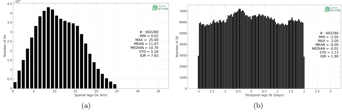
Figure 5: Histograms of the spatial (a) and temporal (b) lags between the time of the TSG (LEGOS-Survostral) measurements and the date of the corresponding SMOS SSS L3 v5 - 9 Days (CATDS-CECOS-LOCEAN) SSS product.
