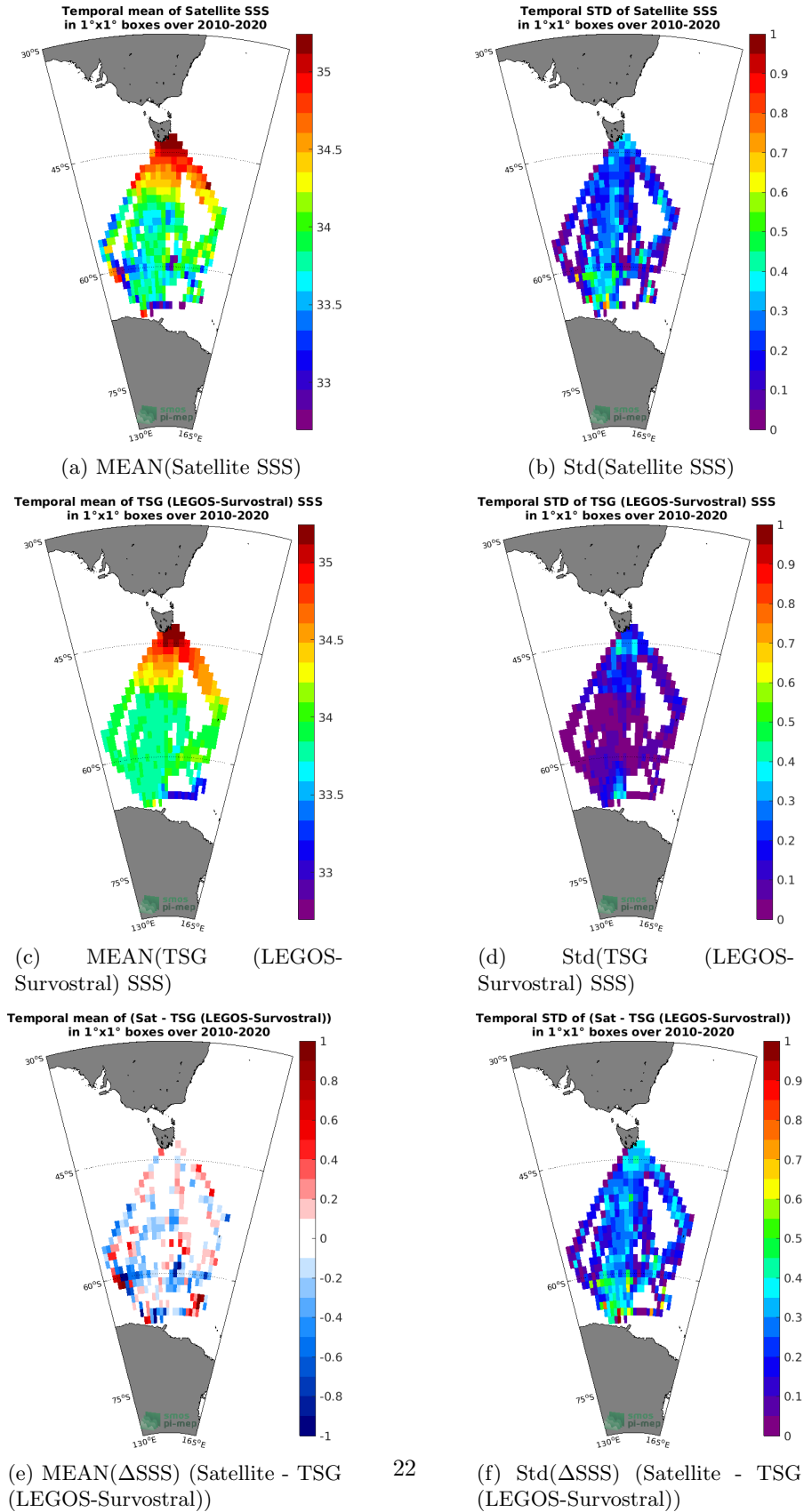
Figure 6: Temporal mean (left) and Std (right) of SSS from SMOS SSS L3 v5 - 9 Days (CATDS-CECOS-LOCEAN) (top), TSG (LEGOS-Survostral) (middle), and of \Delta SSS (Satellite - TSG (LEGOS-Survostral)). Only match-up pairs are used to generate these maps.
