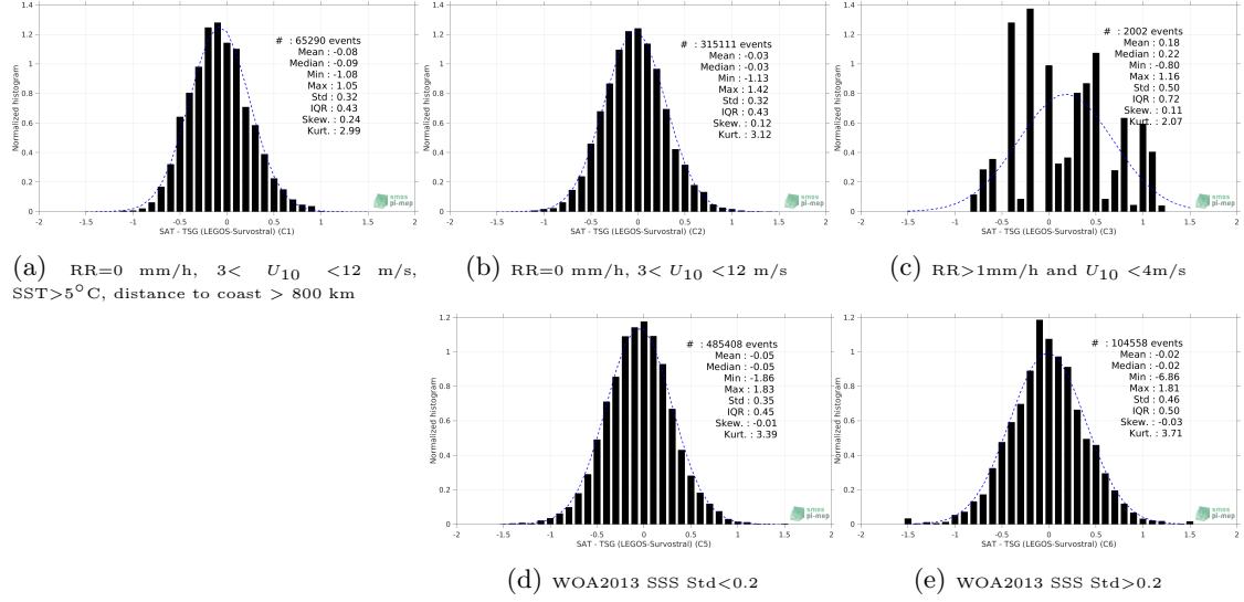
Figure 13: Normalized histogram of \Delta\text{SSS} (SMOS SSS L3 v5 - 9 Days (CATDS-CECOS-LOCEAN) - TSG (LEGOS-Survostral)) for 5 different subdatasets corresponding to: RR=0 mm/h, 3 < U_{10} < 12 m/s, SST > 5^\circ\text{C} , distance to coast > 800 km (a), RR=0 mm/h, 3 < U_{10} < 12 m/s (b), RR > 1\text{mm/h} and U_{10} < 4\text{m/s} (c), WOA2013 SSS Std <0.2 (d), WOA2013 SSS Std >0.2 (e).
