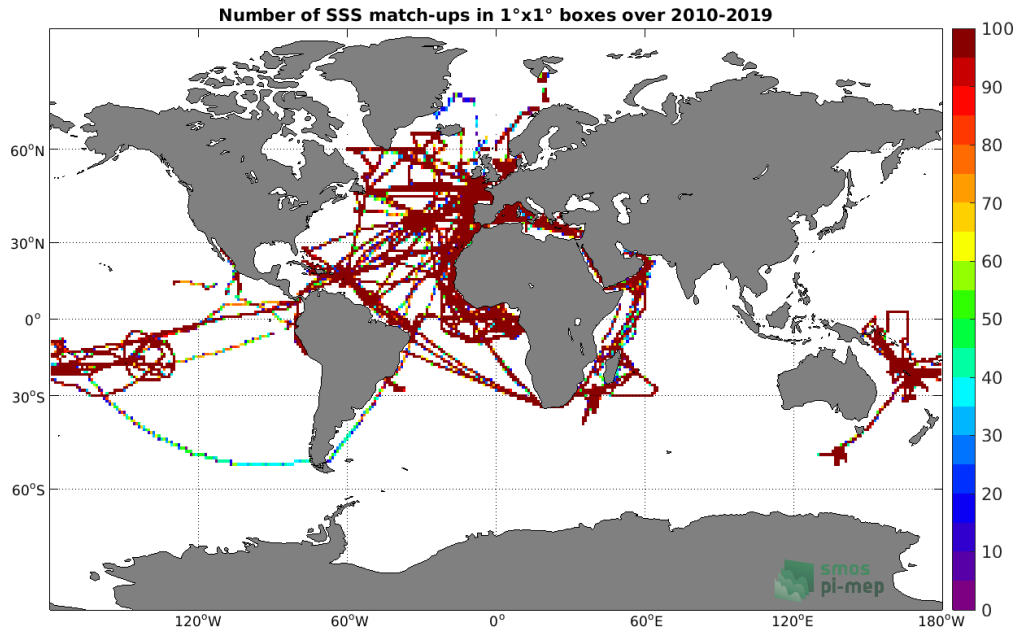
Figure 4: Number of SSS match-ups between TSG (GOSUD-Research-vessel) SSS and the SMOS SSS L3 v5 - 9 Days (CATDS-CECOS-LOCEAN) SSS product for the Global Ocean Pi-MEP region over 1^\circ \times 1^\circ boxes and for the full satellite product period.
