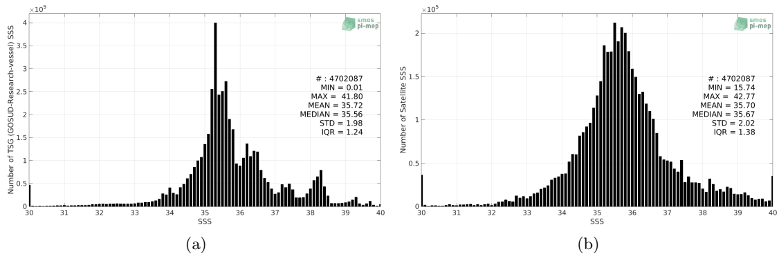
Figure 2: Histograms of SSS from TSG (GOSUD-Research-vessel) (a) and SMOS SSS L3 v5 - 9 Days (CATDS-CECOS-LOCEAN) (b) considering all match-up pairs per bins of 0.1 over the Global Ocean Pi-MEP region and for the full satellite product period.
