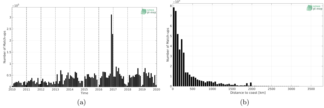
Figure 1: Number of match-ups between TSG (GOSUD-Research-vessel) and SMOS SSS L3 v5 - 9 Days (CATDS-CECOS-LOCEAN) SSS as a function of time (a) and as function of the distance to coast (b) over the Global Ocean Pi-MEP region and for the full satellite product period.
