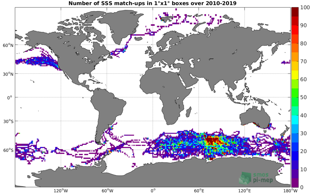
Figure 4: Number of SSS match-ups between Marine mammals SSS and the SMOS SSS L3 v5 - 9 Days (CATDS-CECOS-LOCEAN) SSS product for the Global Ocean Pi-MEP region over 1^\circ \times 1^\circ boxes and for the full satellite product period.
