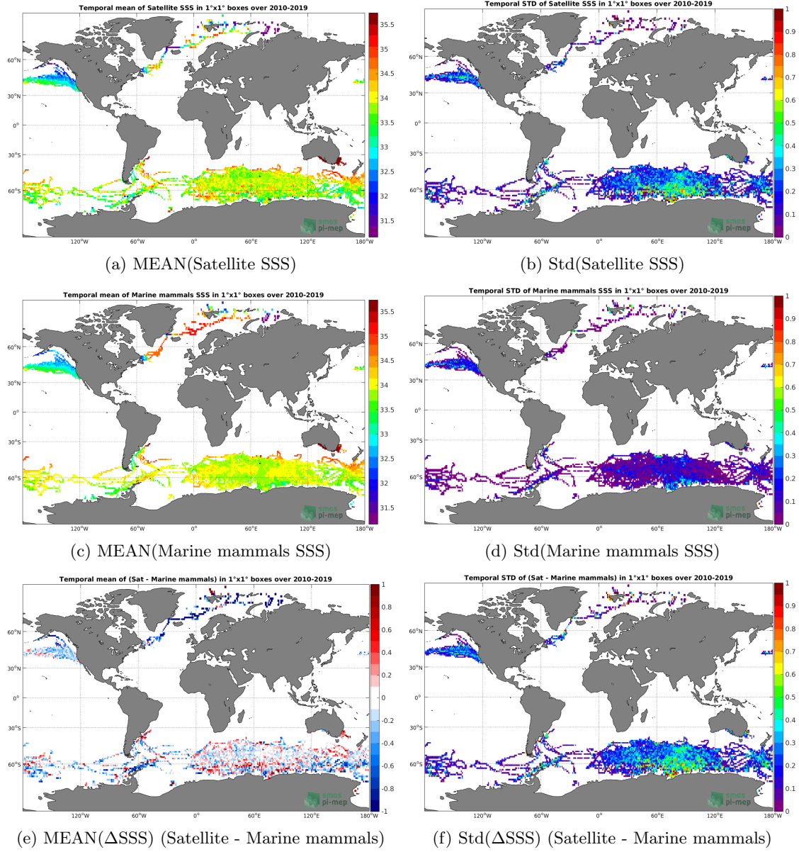
Figure 6: Temporal mean (left) and Std (right) of SSS from SMOS SSS L3 v5 - 9 Days (CATDS-CECOS-LOCEAN) (top), Marine mammals (middle), and of \Delta SSS (Satellite - Marine mammals). Only match-up pairs are used to generate these maps.
