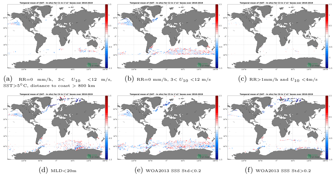
Figure 12: Temporal mean gridded over spatial boxes of size 1^{\circ} \times 1^{\circ} of \Delta\text{SSS} (SMOS SSS L3 v5 - 9 Days (CATDS-CECOS-LOCEAN) - Marine mammals) for 6 different subdatasets corresponding to: RR=0 mm/h, 3 < U_{10} < 12 m/s, SST > 5^{\circ}\text{C} , distance to coast > 800 km (a), RR=0 mm/h, 3 < U_{10} < 12 m/s (b), RR > 1 mm/h and U_{10} < 4 m/s (c), MLD < 20\text{m} (d), WOA2013 SSS Std < 0.2 (e), WOA2013 SSS Std > 0.2 (f).
