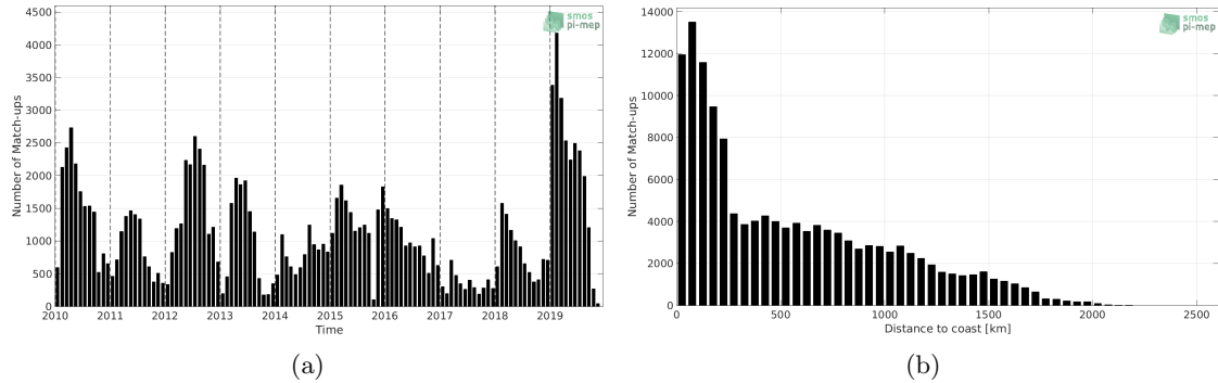
Figure 1: Number of match-ups between Marine mammals and SMOS SSS L3 v5 - 9 Days (CATDS-CECOS-LOCEAN) SSS as a function of time (a) and as function of the distance to coast (b) over the Global Ocean Pi-MEP region and for the full satellite product period.
