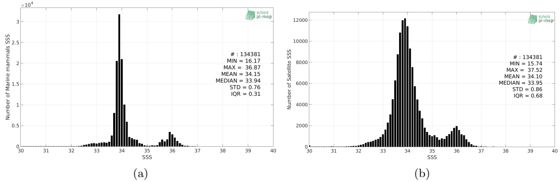
Figure 2: Histograms of SSS from Marine mammals (a) and SMOS SSS L3 v5 - 9 Days (CATDS-CECOS-LOCEAN) (b) considering all match-up pairs per bins of 0.1 over the Global Ocean Pi-MEP region and for the full satellite product period.
