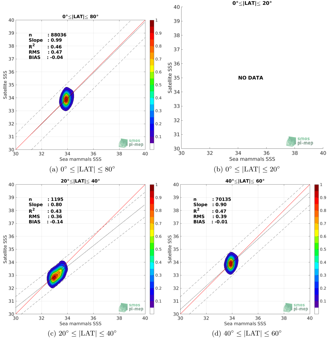
Figure 9: Contour maps of the concentration of SMOS SSS L3 v5 - 9 Days (CATDS-CECOS-LOCEAN) SSS (y-axis) versus Sea mammals SSS (x-axis) at match-up pairs for different latitude bands. For each plot, the red line shows x=y . The black thin and dashed lines indicate a linear fit through the data cloud and the \pm 95\% confidence levels, respectively. The number match-up pairs n , the slope and R^2 coefficient of the linear fit, the root mean square (RMS) and the mean bias between satellite and in situ data are indicated for each latitude band in each plots.
