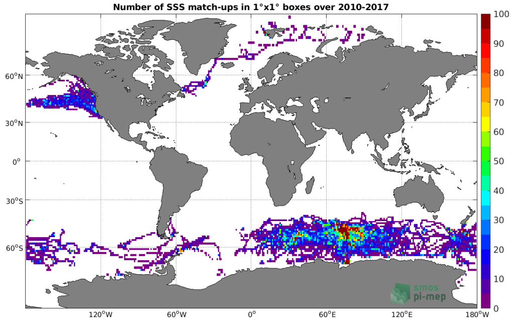
Figure 4: Number of SSS match-ups between Sea mammals SSS and the SMOS SSS L3 v5 - 9 Days (CATDS-CECOS-LOCEAN) SSS product for the Global Ocean Pi-MEP region over 1^\circ \times 1^\circ boxes and for the full satellite product period.
