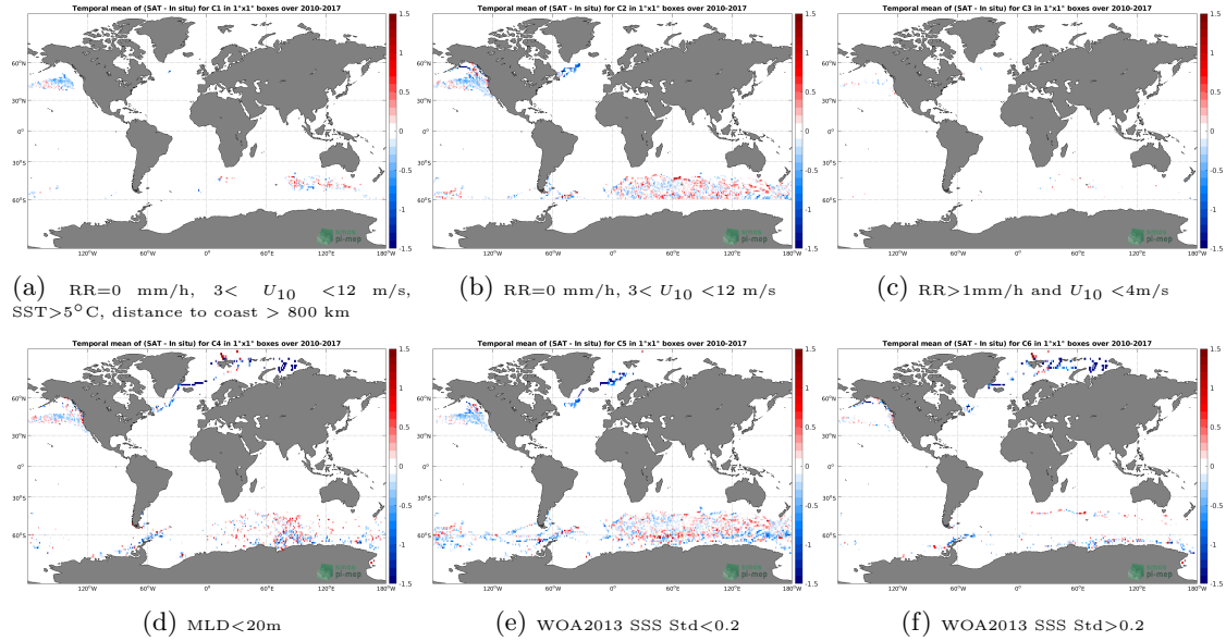
Figure 12: Temporal mean gridded over spatial boxes of size 1^\circ \times 1^\circ of \Delta SSS (SMOS SSS L3 v5 - 9 Days (CATDS-CECOS-LOCEAN) - Sea mammals) for 6 different subdatasets corresponding to: RR=0 mm/h, 3 < U_{10} < 12 m/s, SST > 5^\circ C , distance to coast > 800 km (a), RR=0 mm/h, 3 < U_{10} < 12 m/s (b), RR > 1 mm/h and U_{10} < 4 m/s (c), MLD < 20 m (d), WOA2013 SSS Std < 0.2 (e), WOA2013 SSS Std > 0.2 (f).
