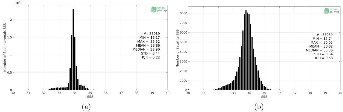
Figure 2: Histograms of SSS from Sea mammals (a) and SMOS SSS L3 v5 - 9 Days (CATDS-CECOS-LOCEAN) (b) considering all match-up pairs per bins of 0.1 over the Global Ocean Pi-MEP region and for the full satellite product period.
