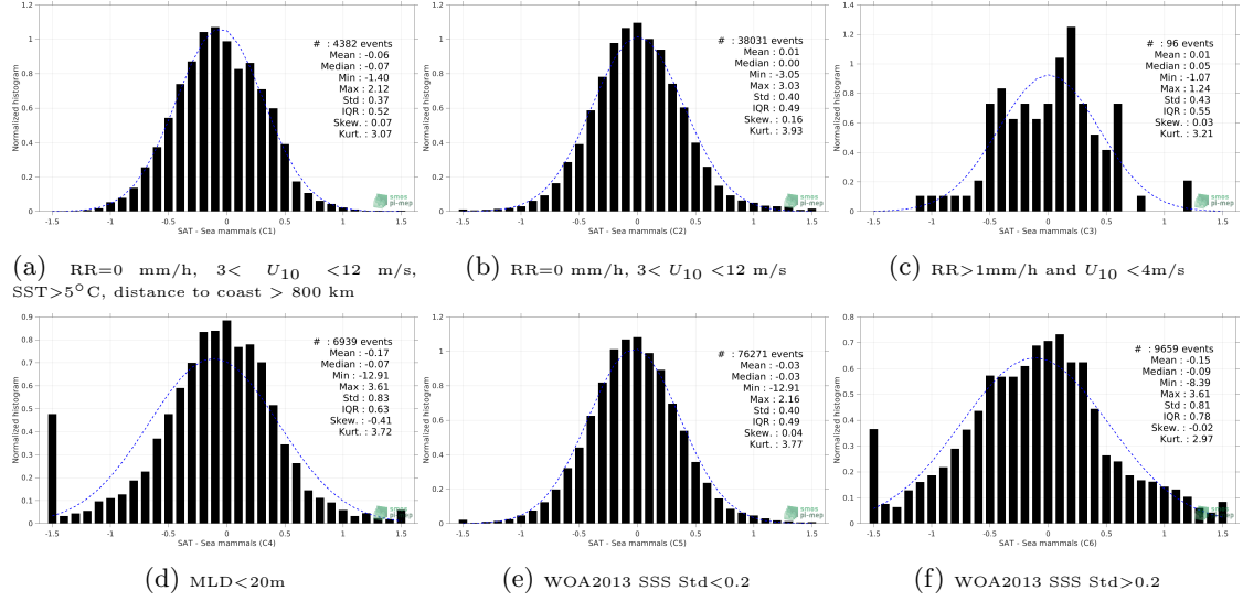
Figure 13: Normalized histogram of \Delta SSS (SMOS SSS L3 v5 - 9 Days (CATDS-CECOS-LOCEAN) - Sea mammals) for 6 different subdatasets corresponding to: RR=0 mm/h, 3 < U_{10} < 12 m/s, SST>5°C, distance to coast > 800 km (a), RR=0 mm/h, 3 < U_{10} < 12 m/s (b), RR>1mm/h and U_{10} < 4 m/s (c), MLD<20m (d), WOA2013 SSS Std<0.2 (e), WOA2013 SSS Std>0.2 (f).
