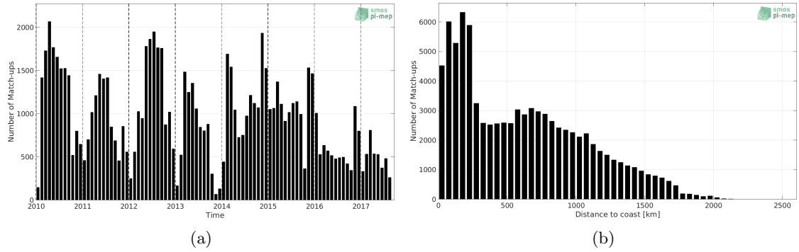
Figure 1: Number of match-ups between Sea mammals and SMOS SSS L3 v5 - 9 Days (CATDS-CECOS-LOCEAN) SSS as a function of time (a) and as function of the distance to coast (b) over the Global Ocean Pi-MEP region and for the full satellite product period.
