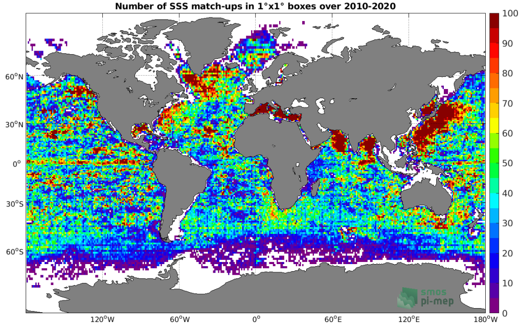
Figure 4: Number of SSS match-ups between Argo SSS and the SMOS SSS L3 v5 - 9 Days (CATDS-CECOS-LOCEAN) SSS product for the Global Ocean Pi-MEP region over 1^\circ \times 1^\circ boxes and for the full satellite product period.
