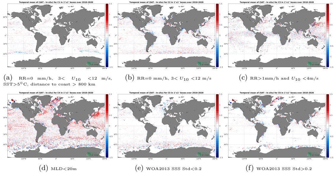
Figure 12: Temporal mean gridded over spatial boxes of size 1^\circ \times 1^\circ of \Delta SSS (SMOS SSS L3 v5 - 9 Days (CATDS-CECOS-LOCEAN) - Argo) for 6 different subdatasets corresponding to: RR=0 mm/h, 3 < U_{10} < 12 m/s, SST > 5^\circ C , distance to coast > 800 km (a), RR=0 mm/h, 3 < U_{10} < 12 m/s (b), RR > 1 mm/h and U_{10} < 4 m/s (c), MLD < 20 m (d), WOA2013 SSS Std < 0.2 (e), WOA2013 SSS Std > 0.2 (f).
