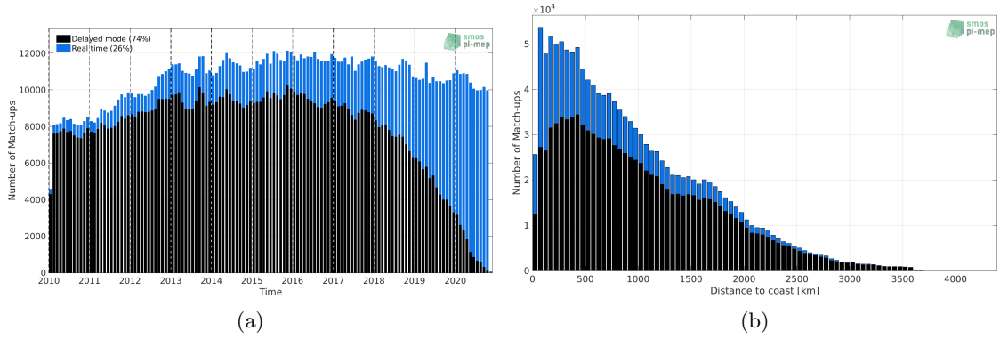
Figure 1: Number of match-ups between Argo and SMOS SSS L3 v5 - 9 Days (CATDS-CECOS-LOCEAN) SSS as a function of time (a) and as function of the distance to coast (b) over the Global Ocean Pi-MEP region and for the full satellite product period.
