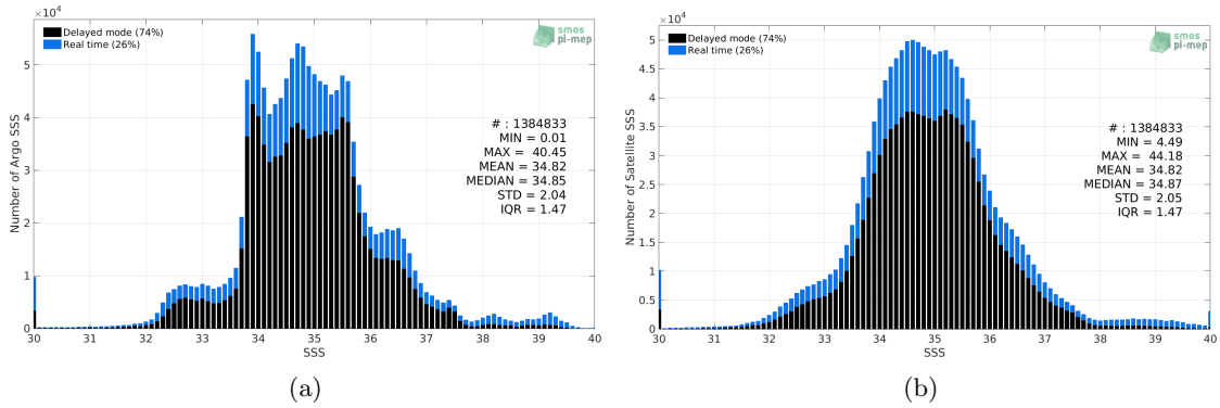
Figure 2: Histograms of SSS from Argo (a) and SMOS SSS L3 v5 - 9 Days (CATDS-CECOS-LOCEAN) (b) considering all match-up pairs per bins of 0.1 over the Global Ocean Pi-MEP region and for the full satellite product period.
