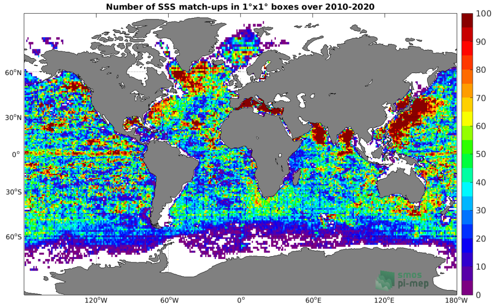
Figure 4: Number of SSS match-ups between Argo SSS and the SMOS SSS L3 v5 - 9 Days (CATDS-CECOS-LOCEAN) SSS product for the Global Ocean Pi-MEP region over 1^\circ \times 1^\circ boxes and for the full satellite product period.
