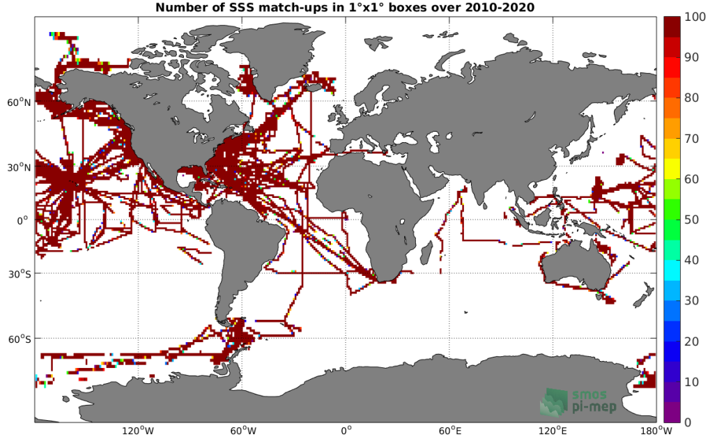
Figure 4: Number of SSS match-ups between TSG (SAMOS) SSS and the SMOS SSS L3 v5 - 18 Days (CATDS-CECOS-LOCEAN) SSS product for the Global Ocean Pi-MEP region over 1^\circ \times 1^\circ boxes and for the full satellite product period.
