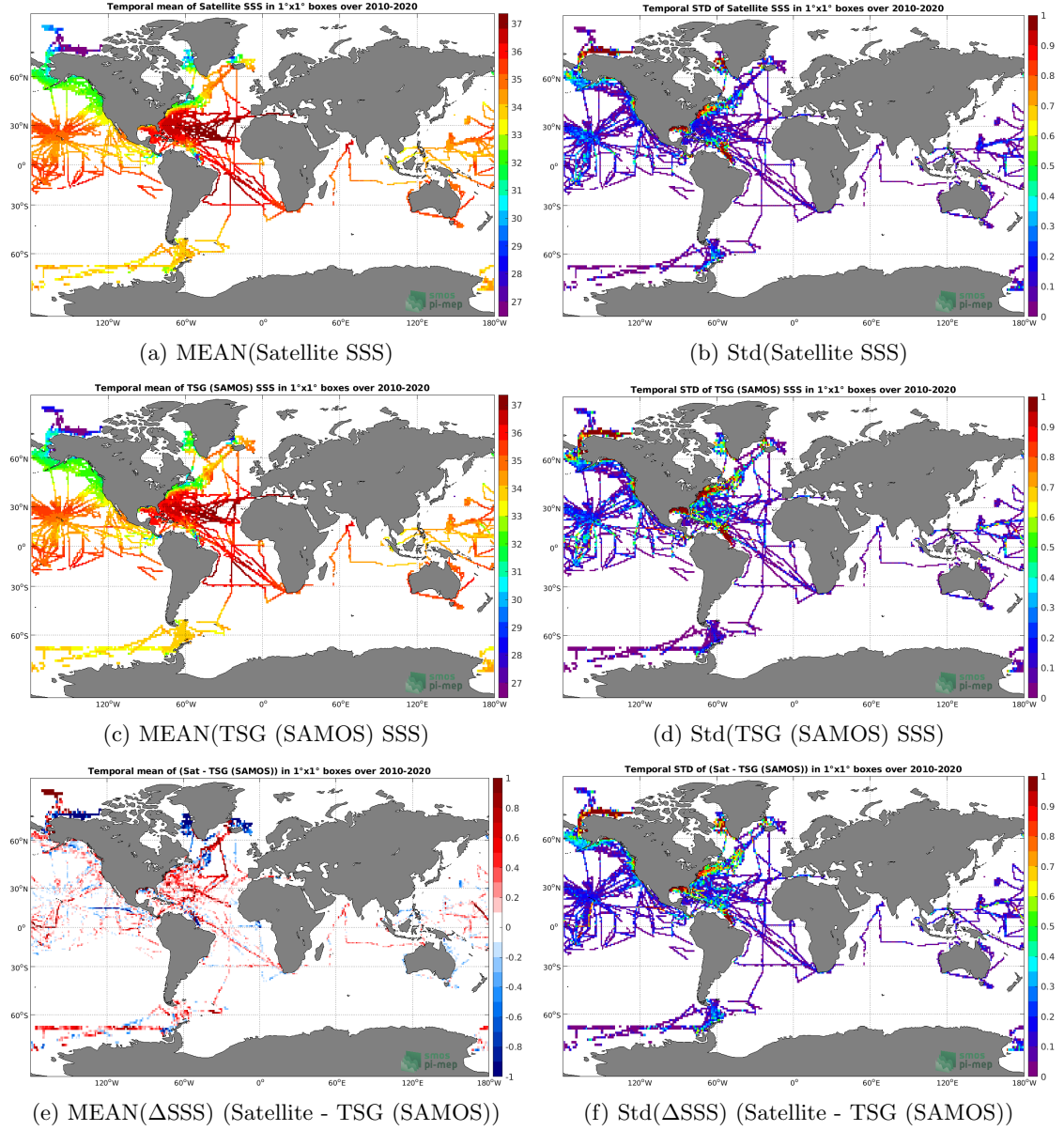
Figure 6: Temporal mean (left) and Std (right) of SSS from SMOS SSS L3 v5 - 18 Days (CATDS-CECOS-LOCEAN) (top), TSG (SAMOS) (middle), and of \Delta SSS (Satellite - TSG (SAMOS)). Only match-up pairs are used to generate these maps.
