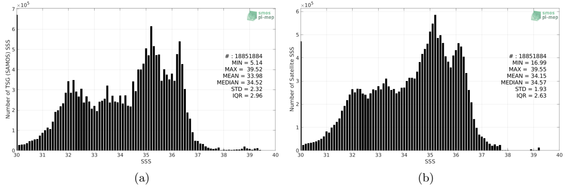
Figure 2: Histograms of SSS from TSG (SAMOS) (a) and SMOS SSS L3 v5 - 18 Days (CATDS-CECOS-LOCEAN) (b) considering all match-up pairs per bins of 0.1 over the Global Ocean Pi-MEP region and for the full satellite product period.
