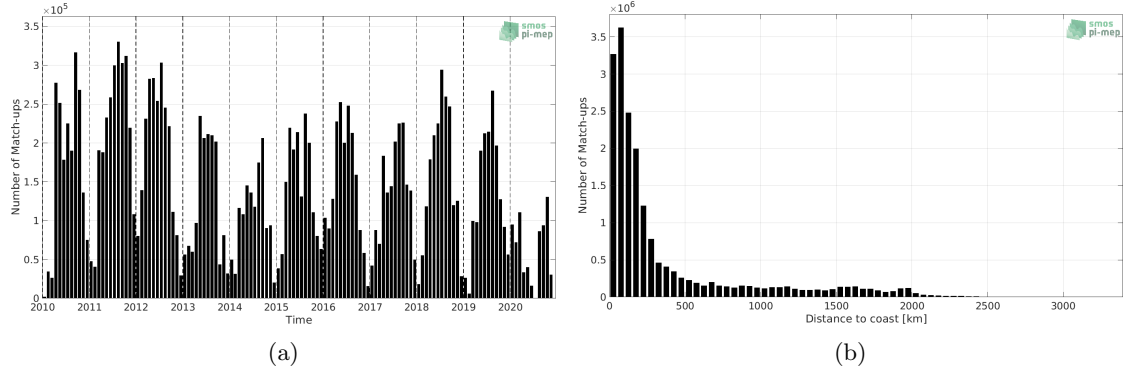
Figure 1: Number of match-ups between TSG (SAMOS) and SMOS SSS L3 v5 - 18 Days (CATDS-CECOS-LOCEAN) SSS as a function of time (a) and as function of the distance to coast (b) over the Global Ocean Pi-MEP region and for the full satellite product period.
