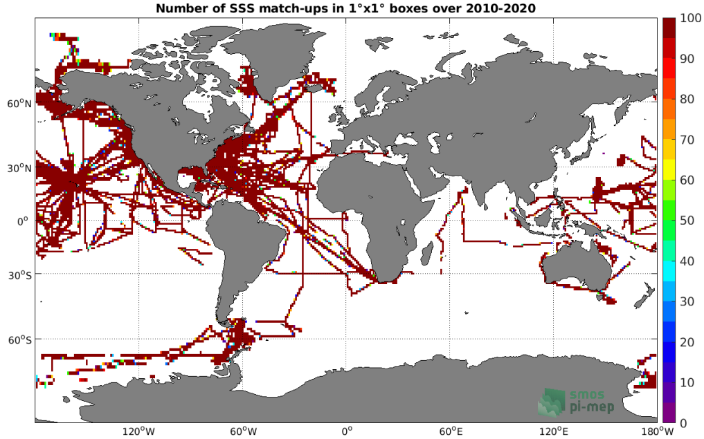
Figure 4: Number of SSS match-ups between TSG (SAMOS) SSS and the SMOS SSS L3 v5 - 18 Days (CATDS-CECOS-LOCEAN) SSS product for the Global Ocean Pi-MEP region over 1^\circ \times 1^\circ boxes and for the full satellite product period.
