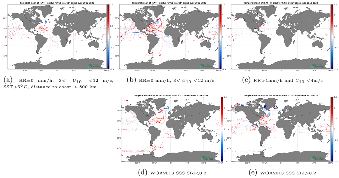
Figure 12: Temporal mean gridded over spatial boxes of size 1^\circ \times 1^\circ of \Delta SSS (SMOS SSS L3 v5 - 18 Days (CATDS-CECOS-LOCEAN) - TSG (SAMOS)) for 5 different subdatasets corresponding to:RR=0 mm/h, 3 < U_{10} < 12 m/s, SST>5°C, distance to coast > 800 km (a), RR=0 mm/h, 3 < U_{10} < 12 m/s (b), RR>1mm/h and U_{10} < 4 m/s (c), WOA2013 SSS Std<0.2 (d), WOA2013 SSS Std>0.2 (e).
